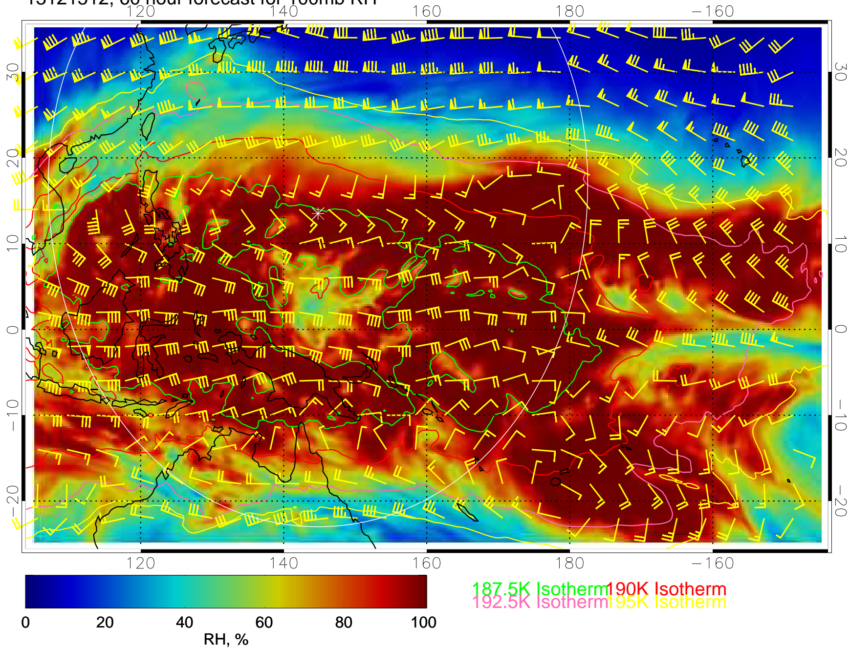
13121512, 60 hour forecast for 100mb RH
