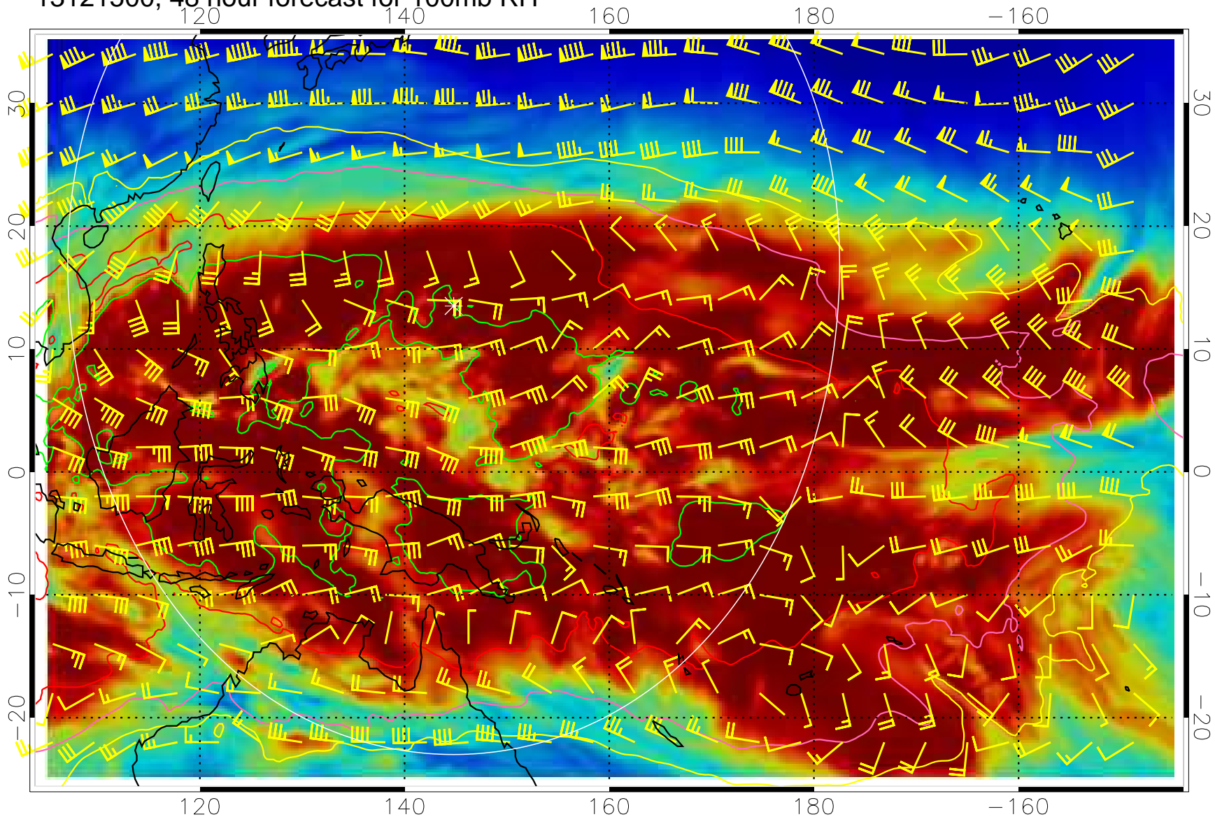
13121500, 48 hour forecast for 100mb RH
