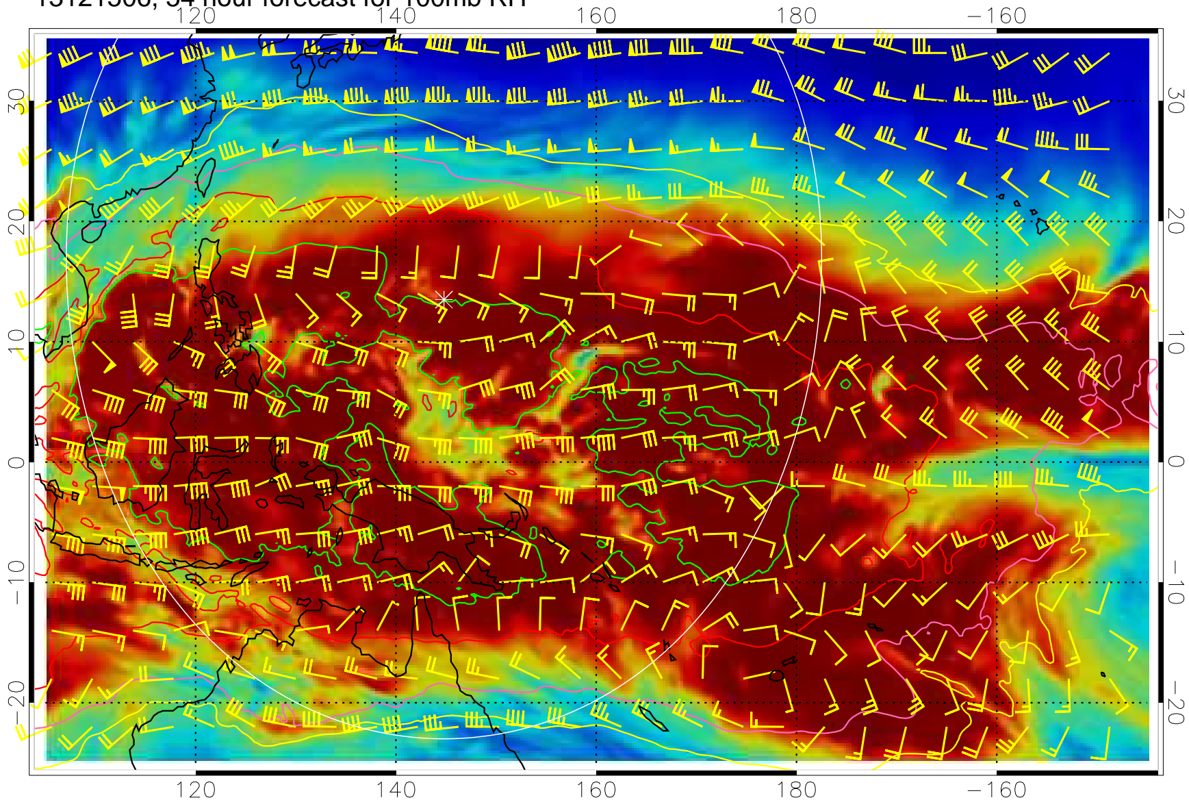
13121506, 54 hour forecast for 100mb RH
