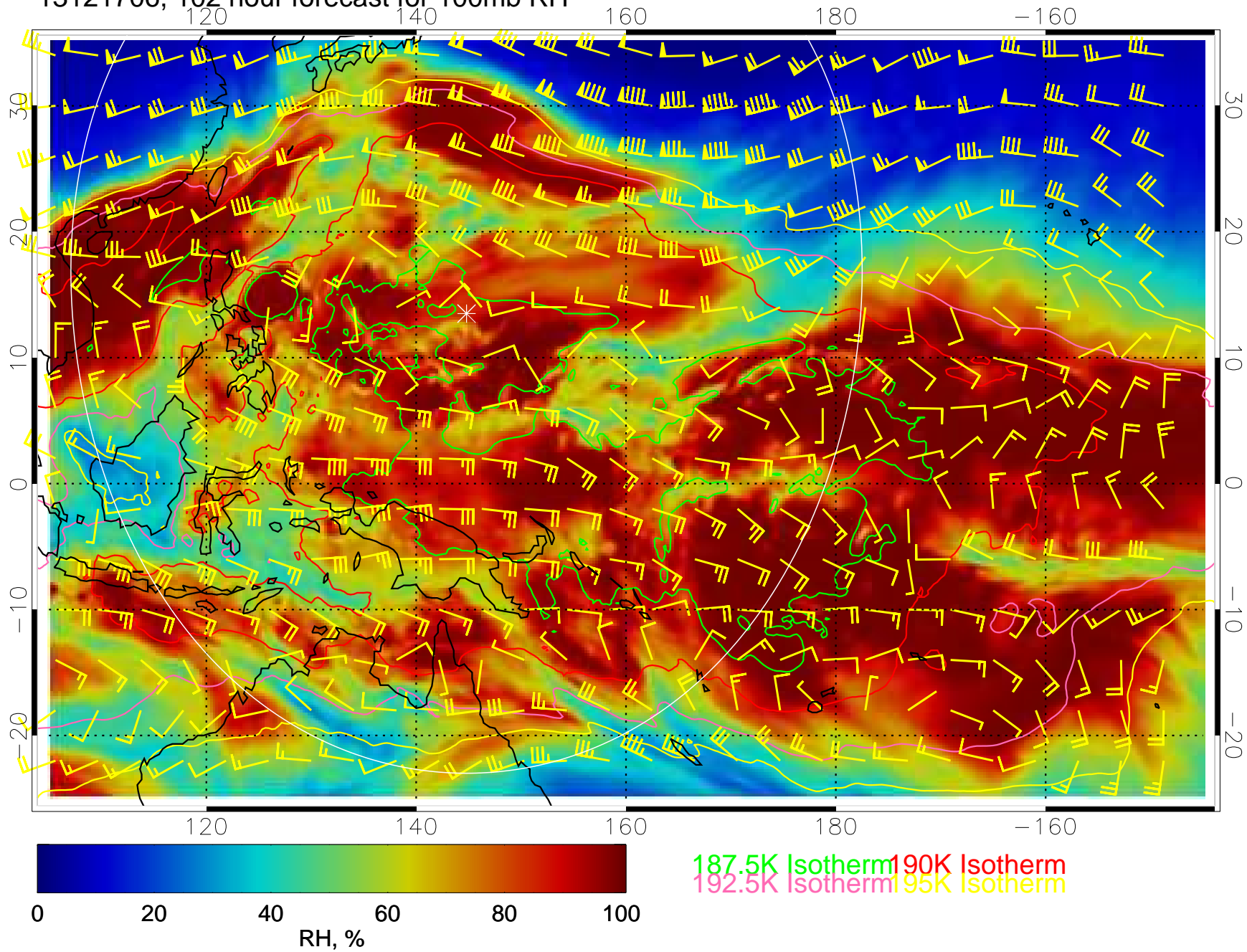
13121706, 102 hour forecast for 100mb RH
