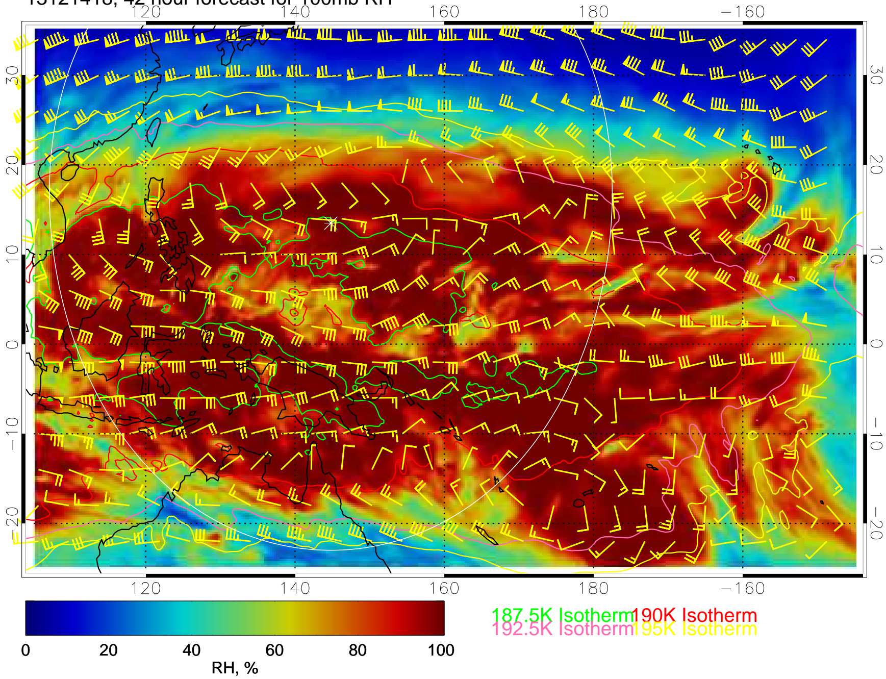
13121418, 42 hour forecast for 100mb RH
