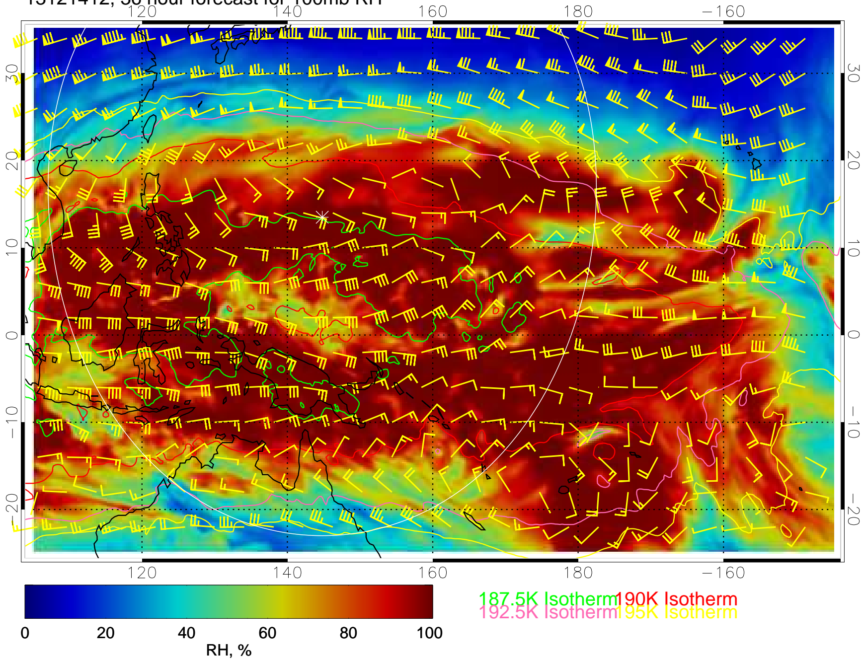
13121412, 36 hour forecast for 100mb RH
