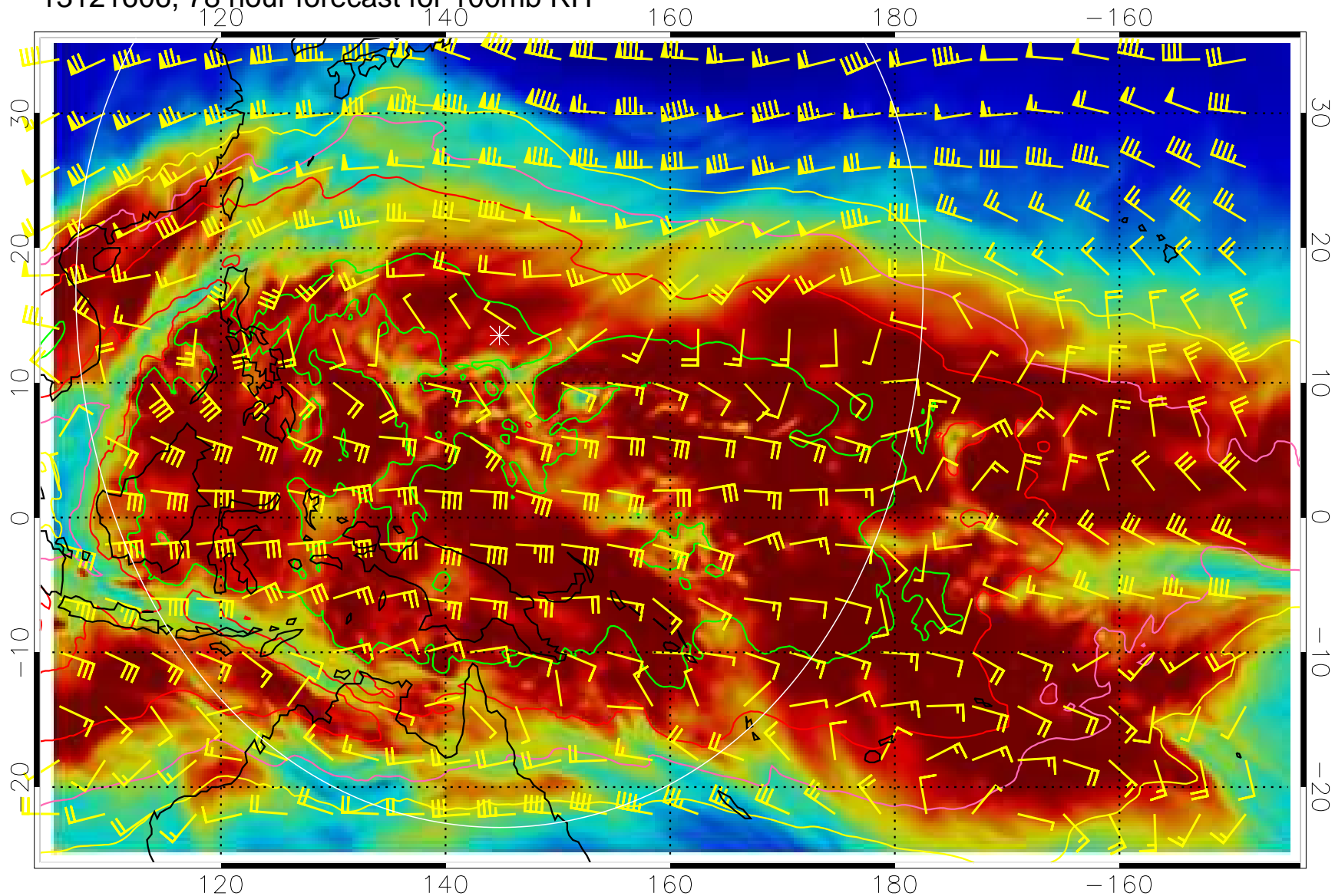
13121606, 78 hour forecast for 100mb RH
