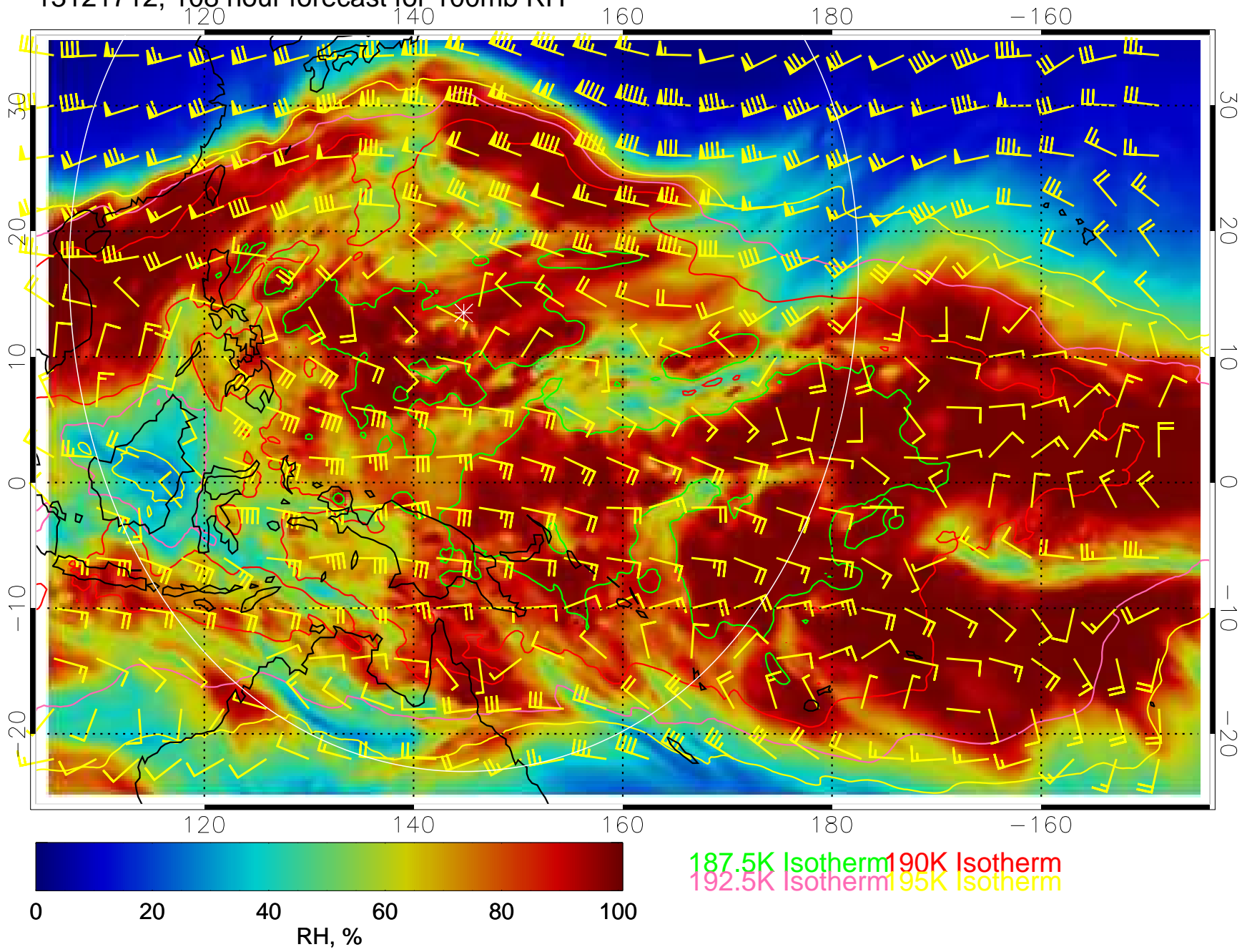
13121712, 108 hour forecast for 100mb RH
