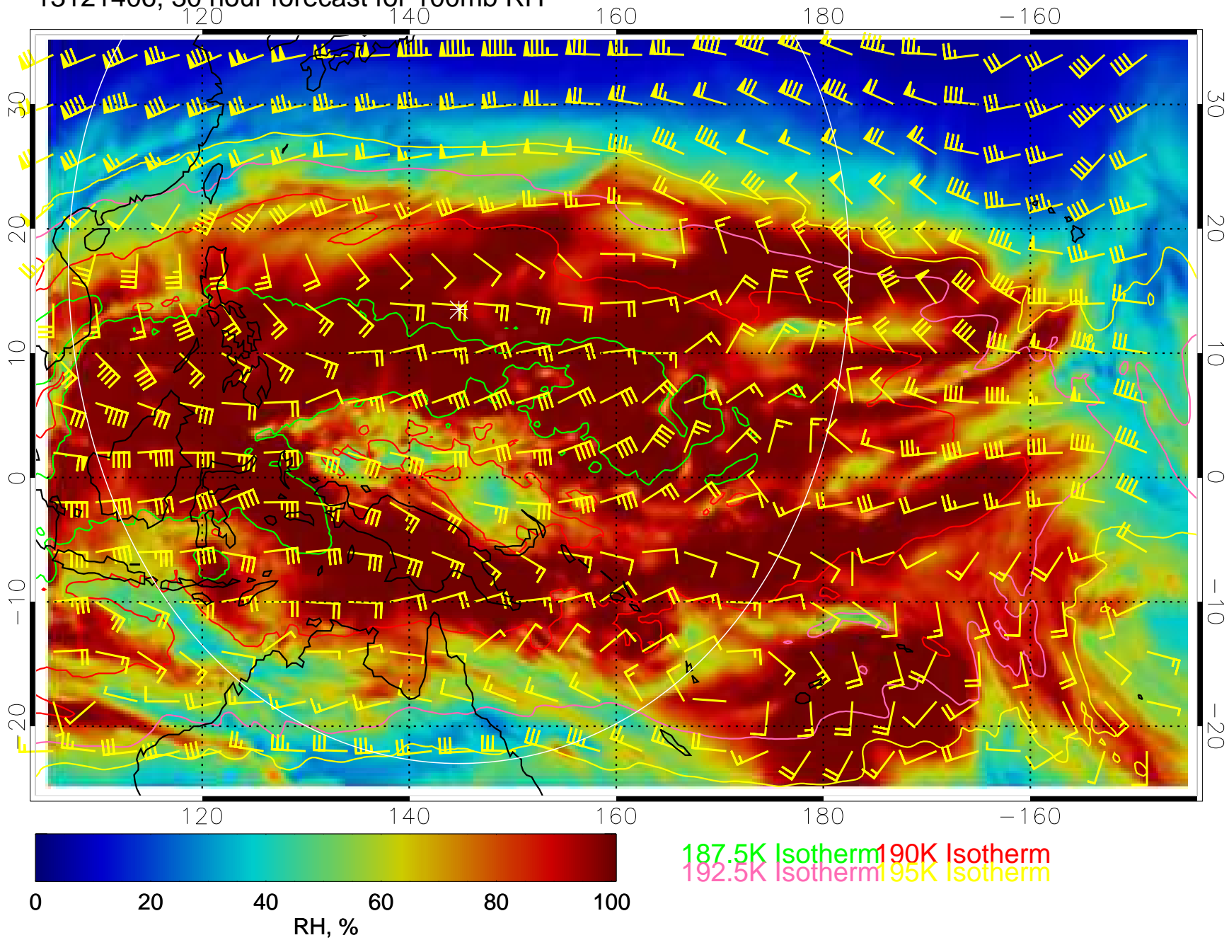
13121406, 30 hour forecast for 100mb RH
