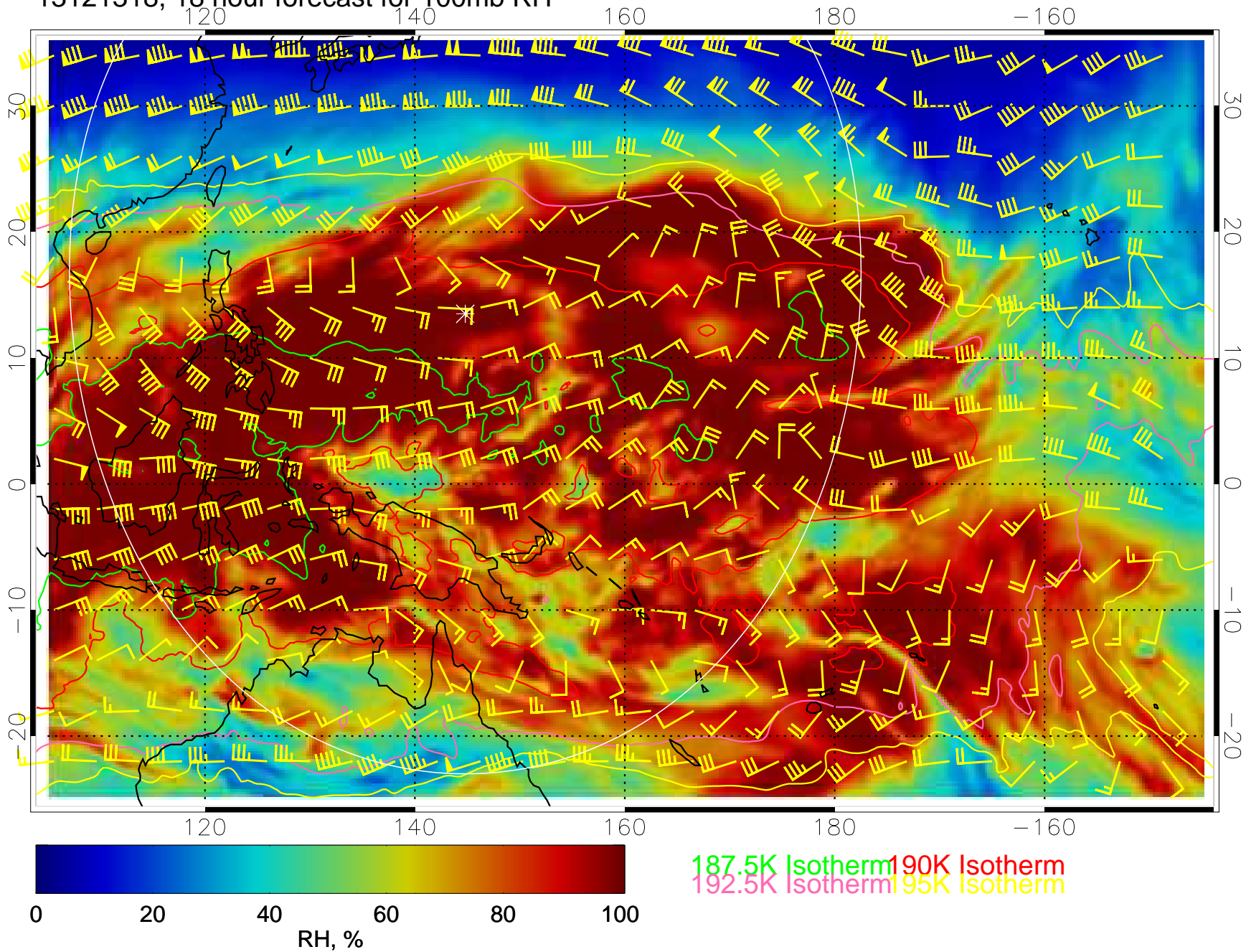
13121318, 18 hour forecast for 100mb RH
