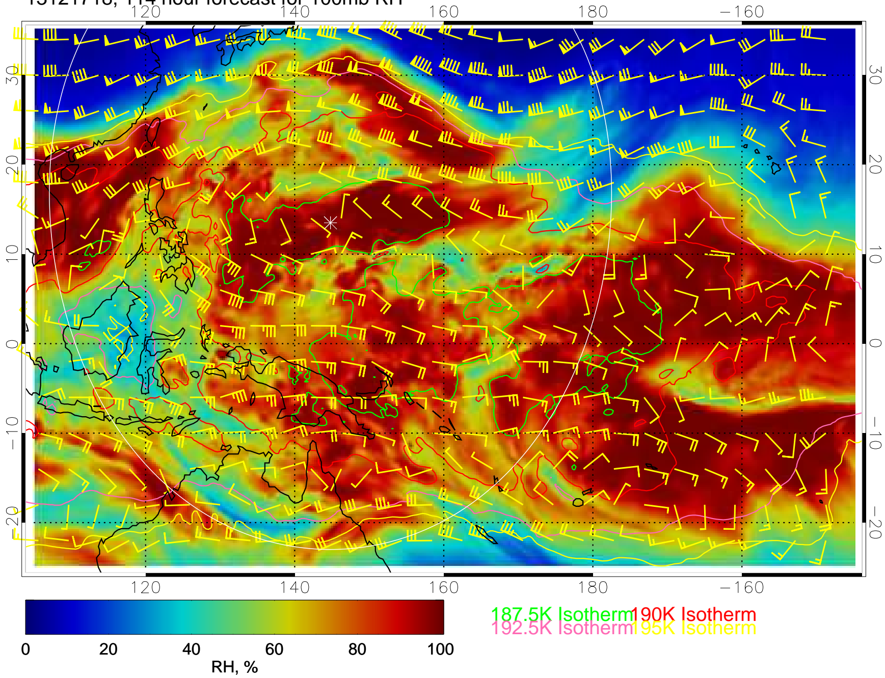
13121718, 114 hour forecast for 100mb RH
