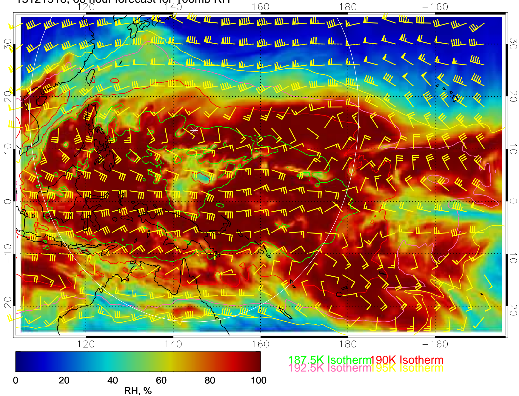
13121518, 66 hour forecast for 100mb RH
