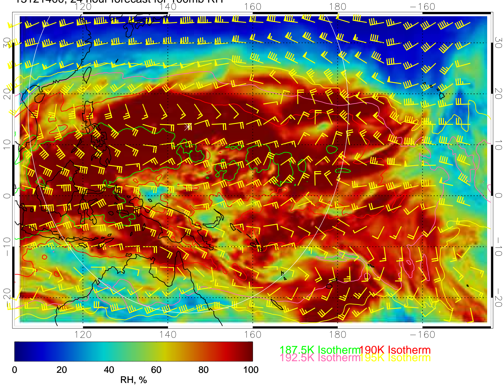
13121400, 24 hour forecast for 100mb RH
