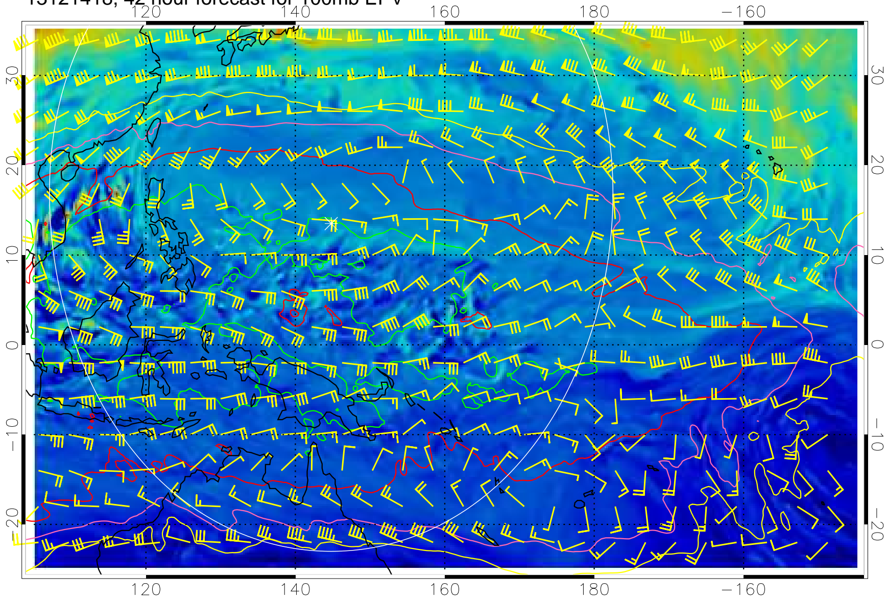
13121418, 42 hour forecast for 100mb EPV
