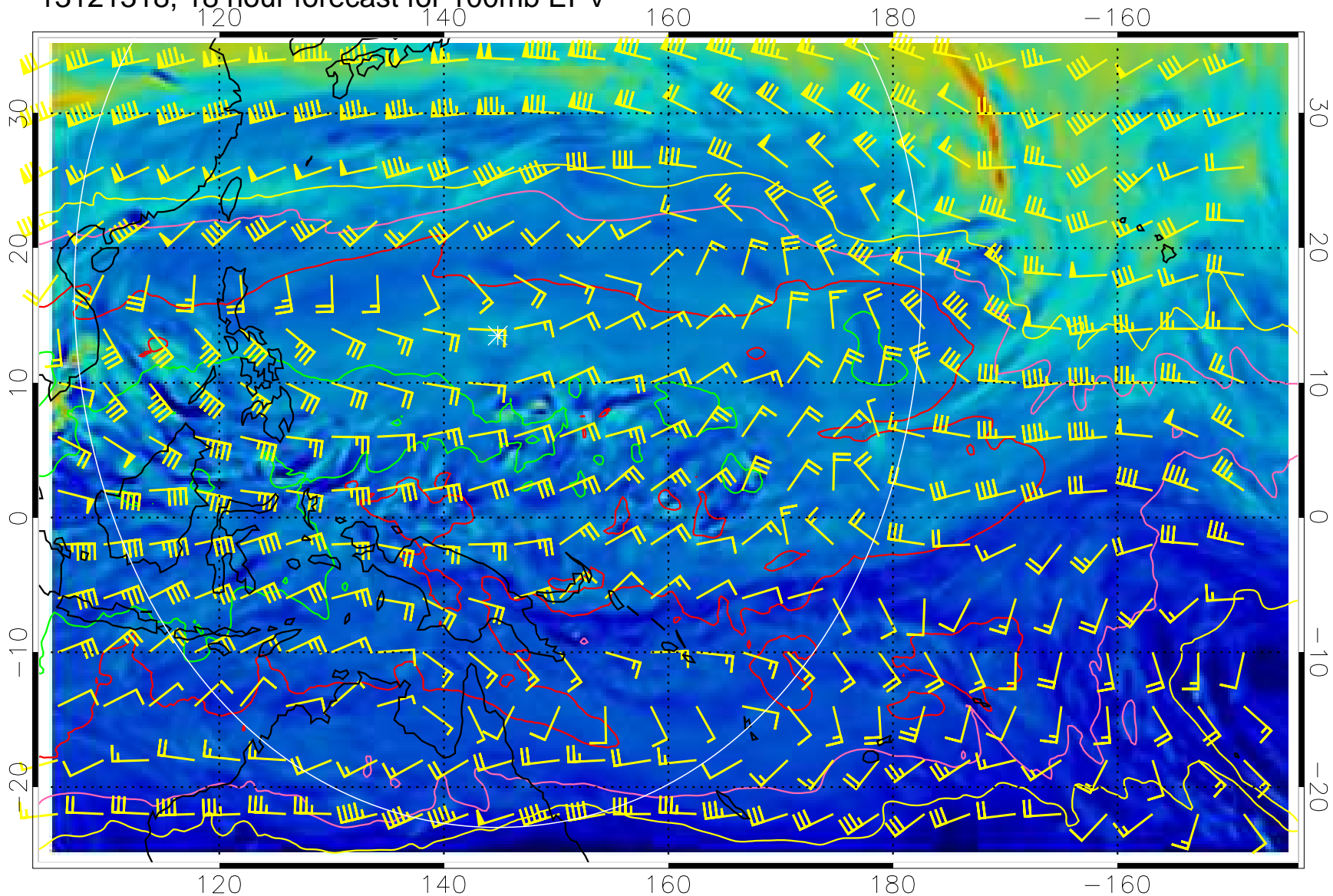
13121318, 18 hour forecast for 100mb EPV
