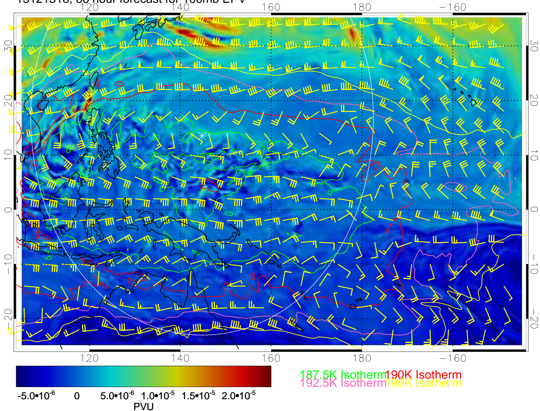
13121518, 66 hour forecast for 100mb EPV
