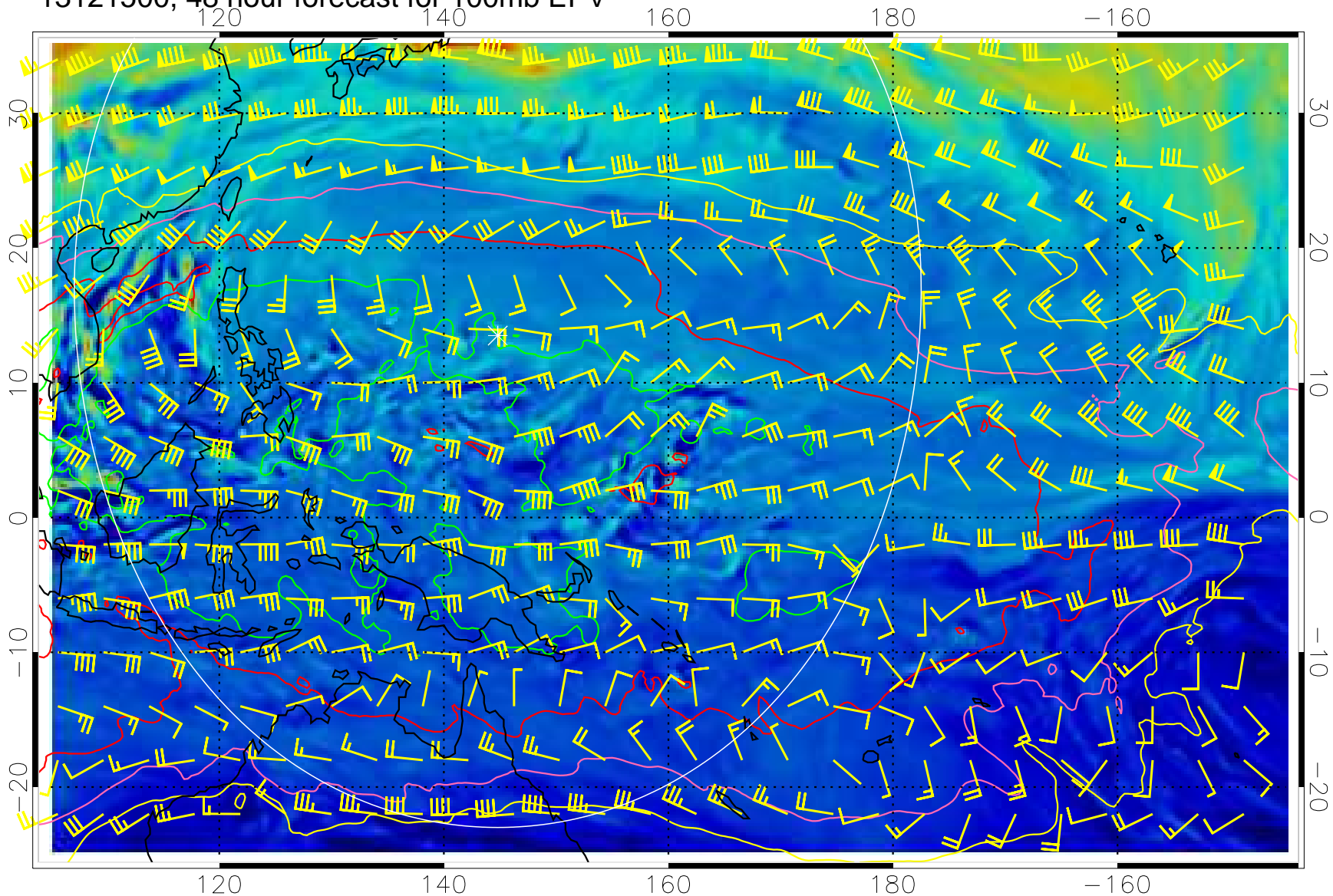
13121500, 48 hour forecast for 100mb EPV
