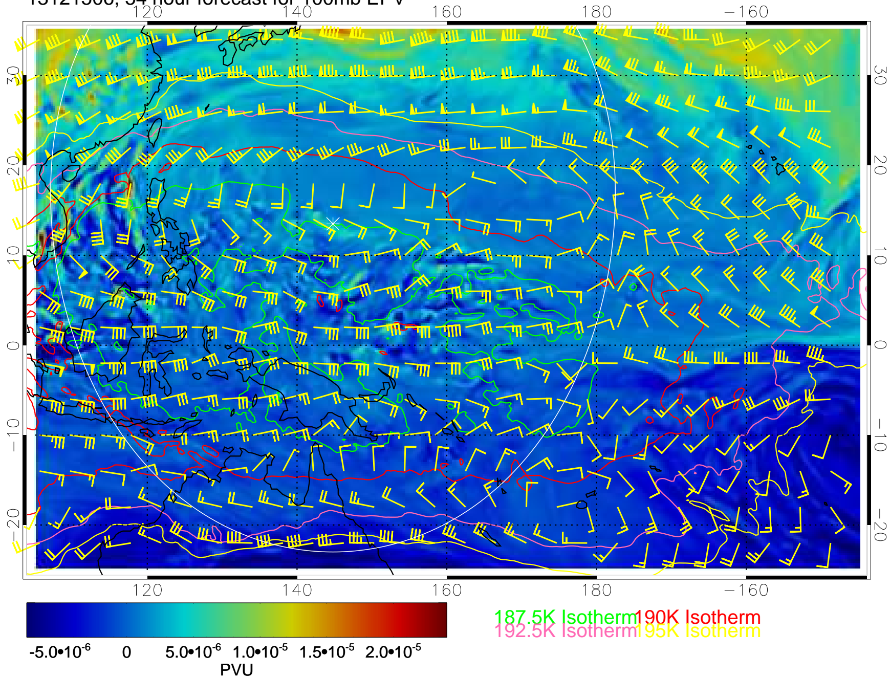
13121506, 54 hour forecast for 100mb EPV
