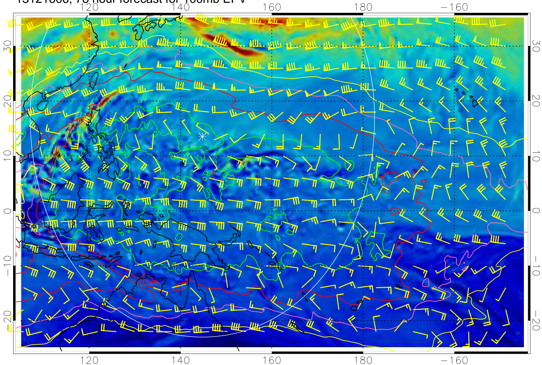
13121606, 78 hour forecast for 100mb EPV
