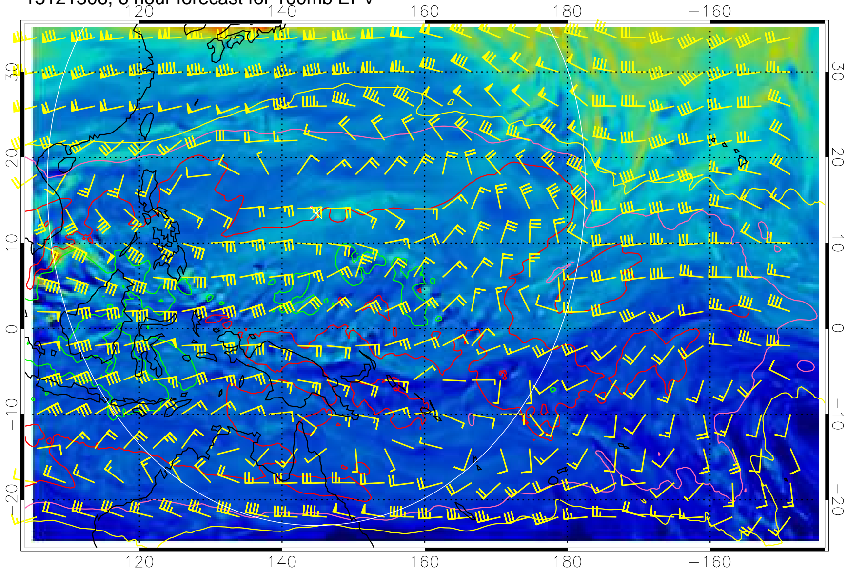
13121306, 6 hour forecast for 100mb EPV
