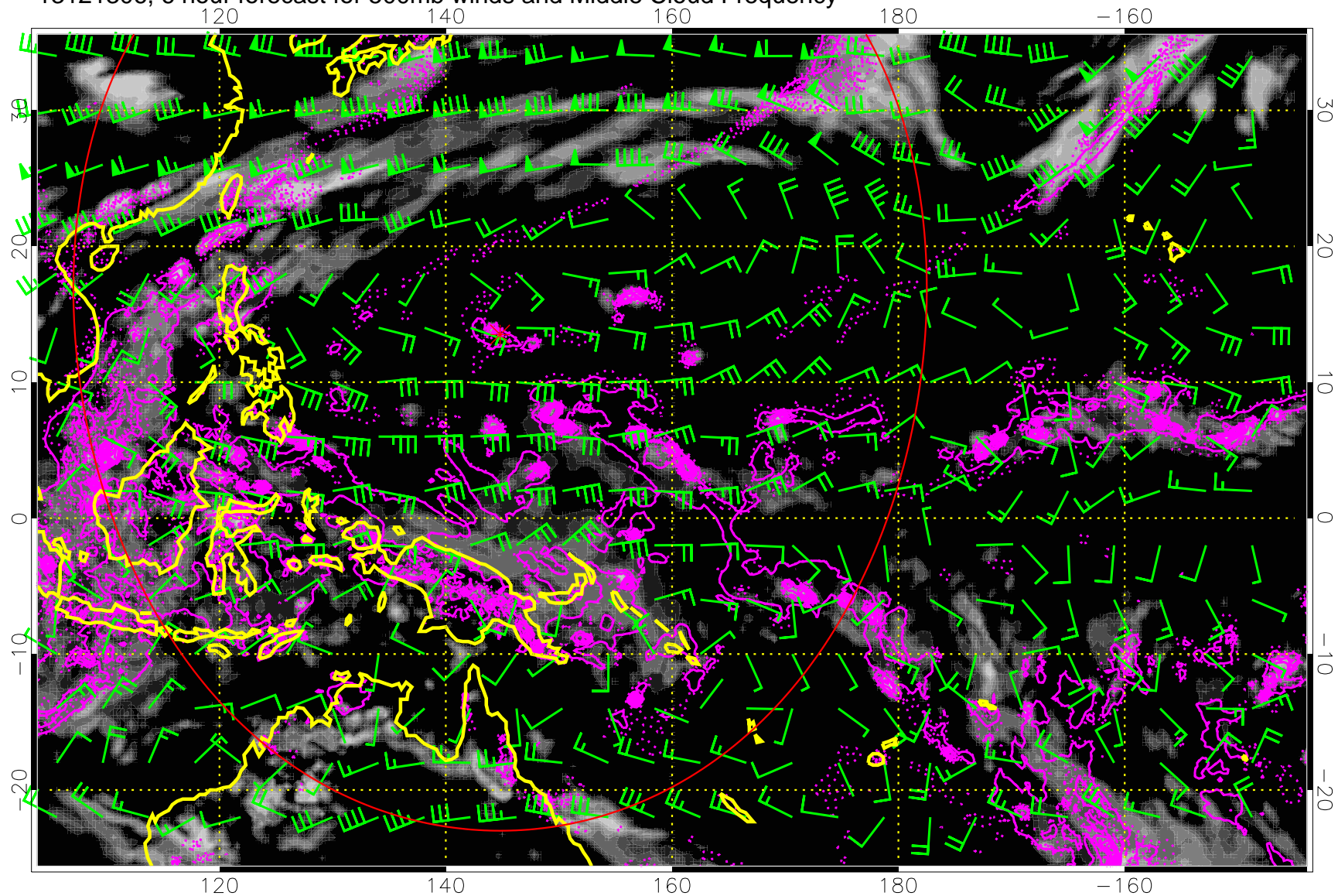
13121306, 6 hour forecast for 500mb winds and Middle Cloud Frequency
