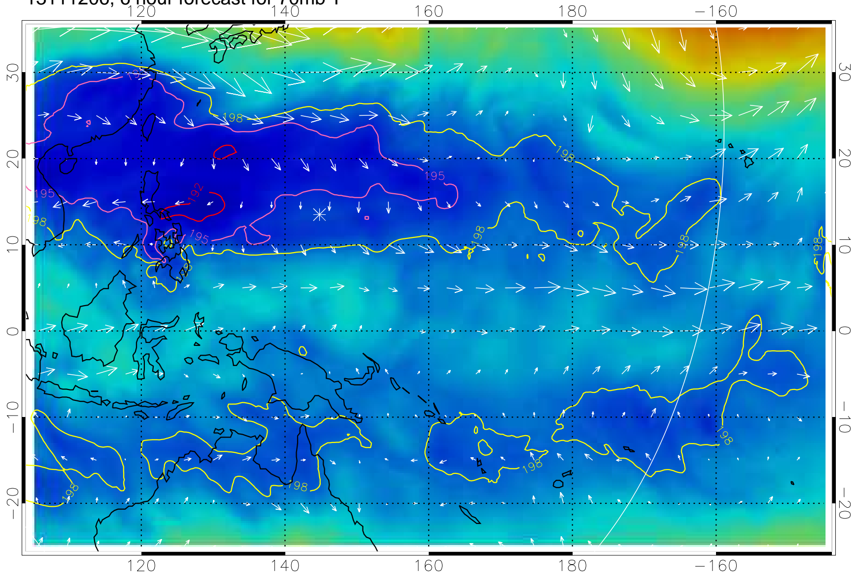
13111206, 6 hour forecast for 70mb T
