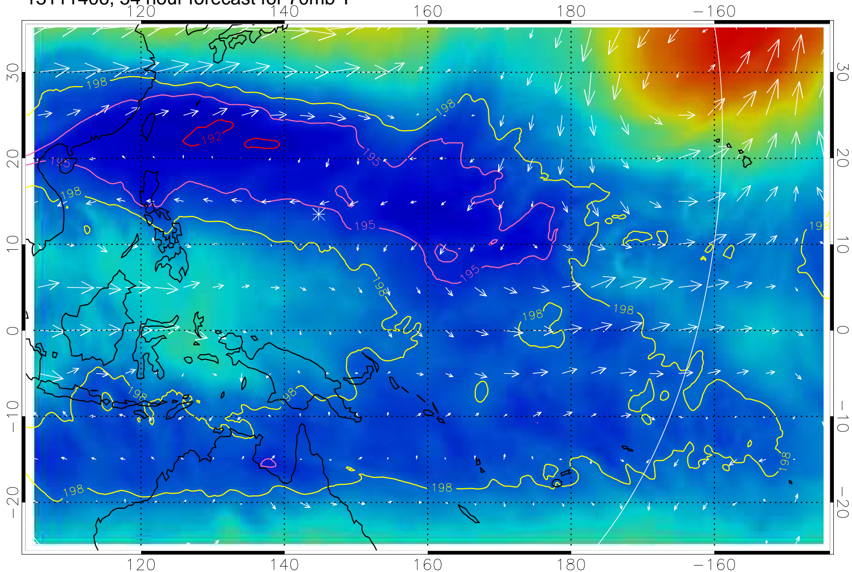
13111406, 54 hour forecast for 70mb T
