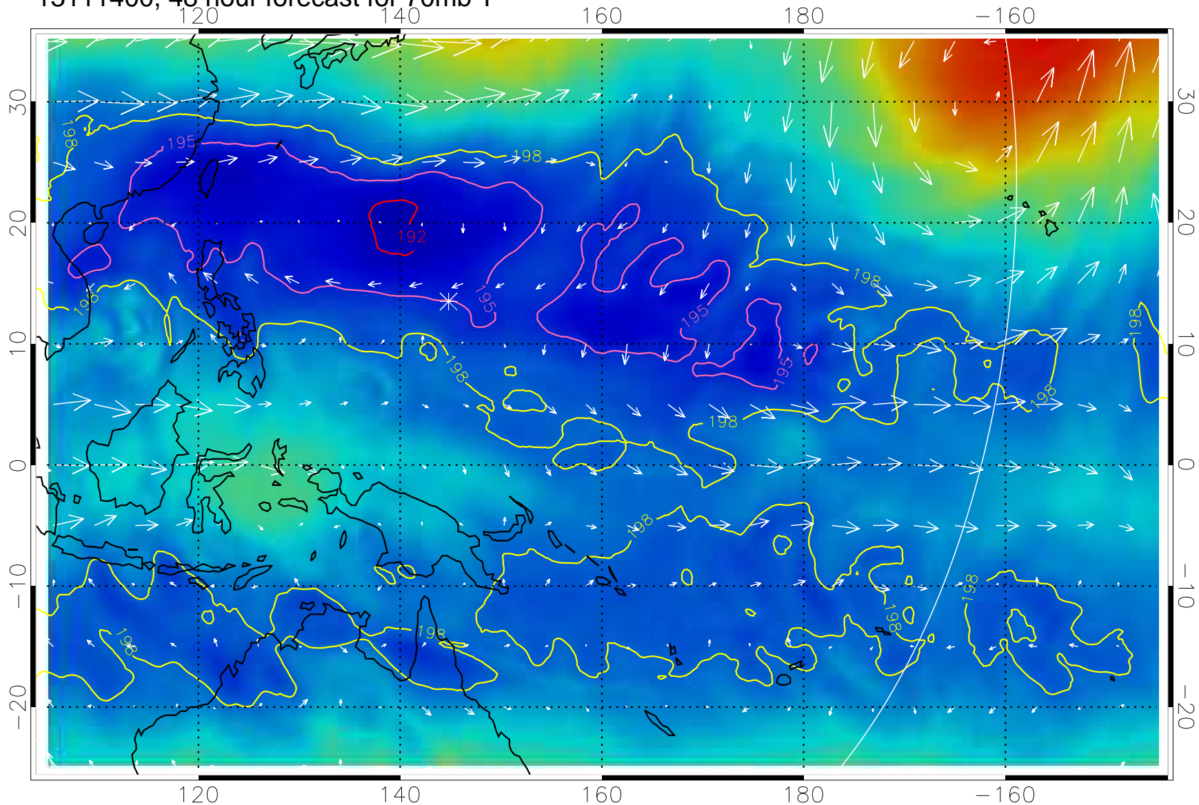
13111400, 48 hour forecast for 70mb T
