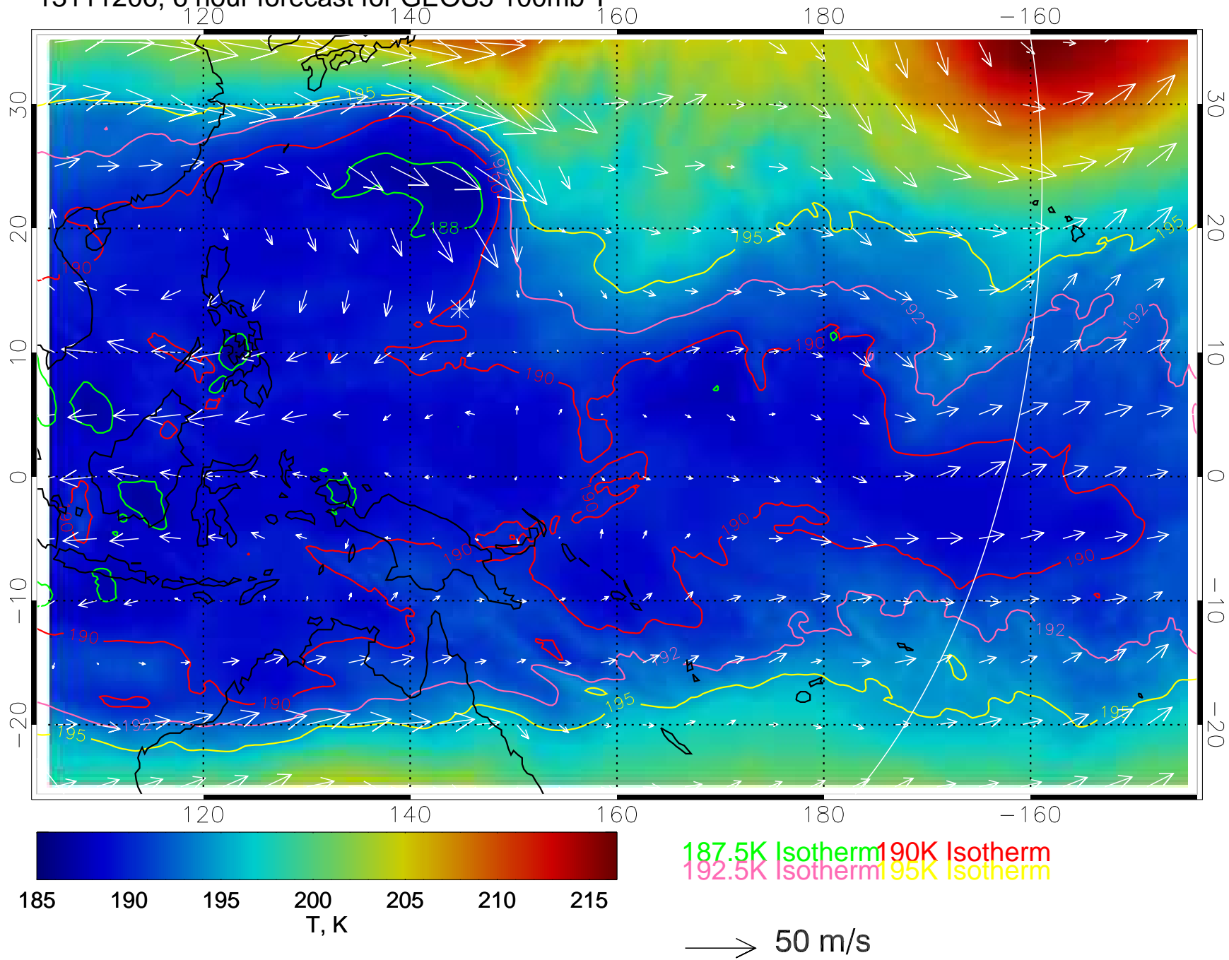
13111206, 6 hour forecast for GEOS5 100mb T
