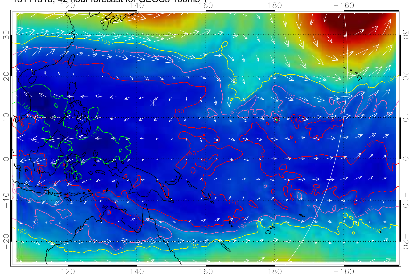
13111318, 42 hour forecast for GEOS5 100mb T
