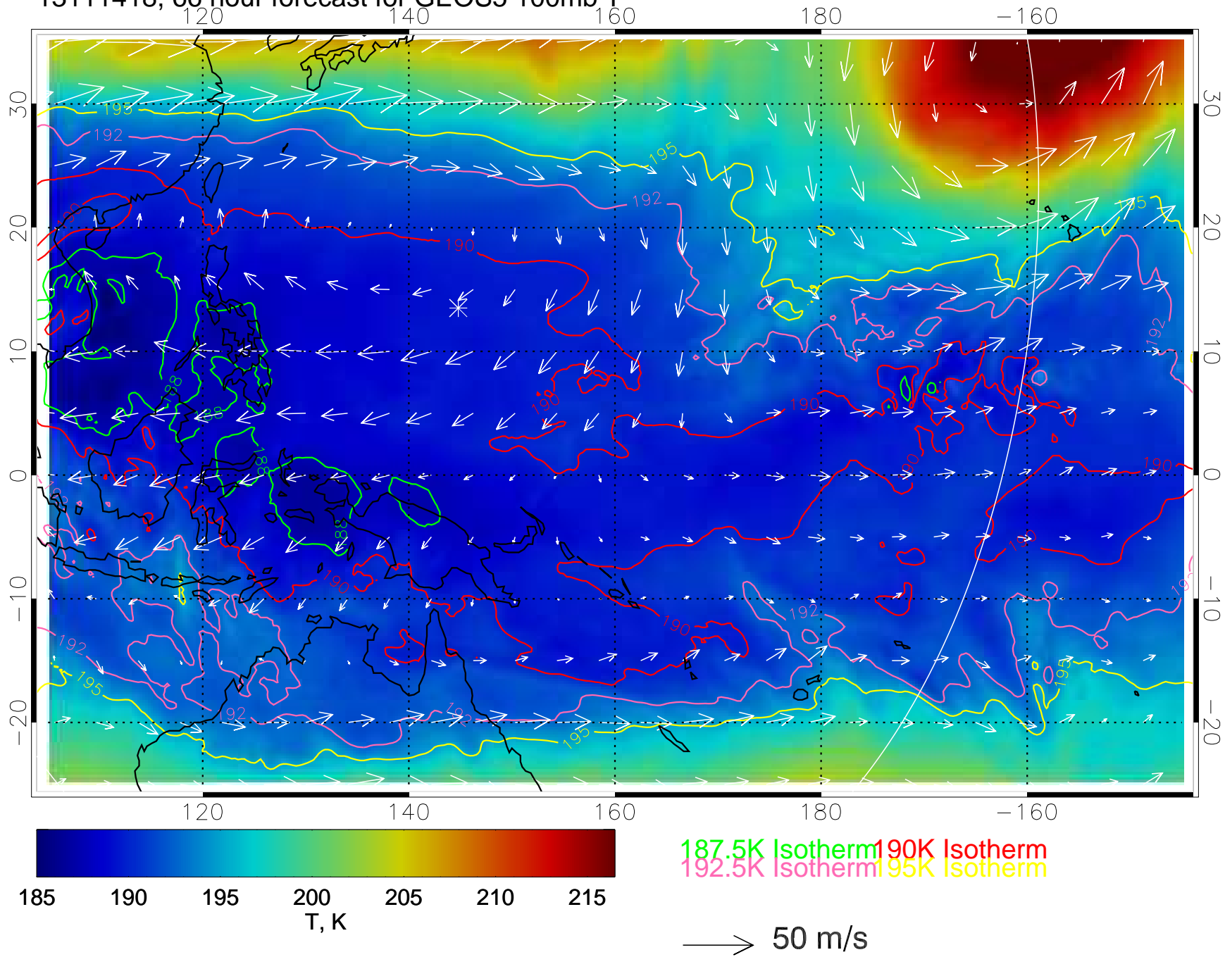
13111418, 66 hour forecast for GEOS5 100mb T
