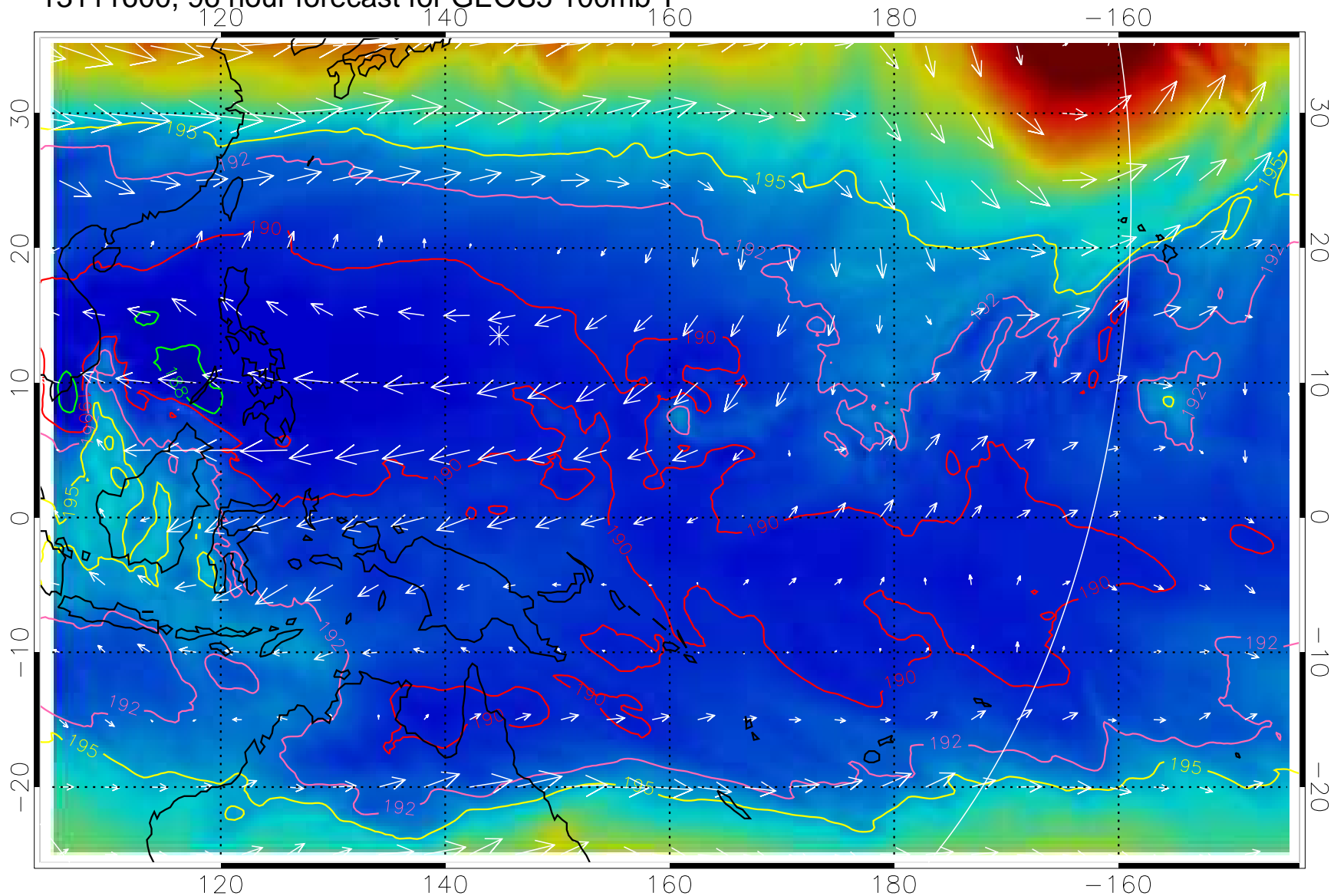
13111600, 96 hour forecast for GEOS5 100mb T
