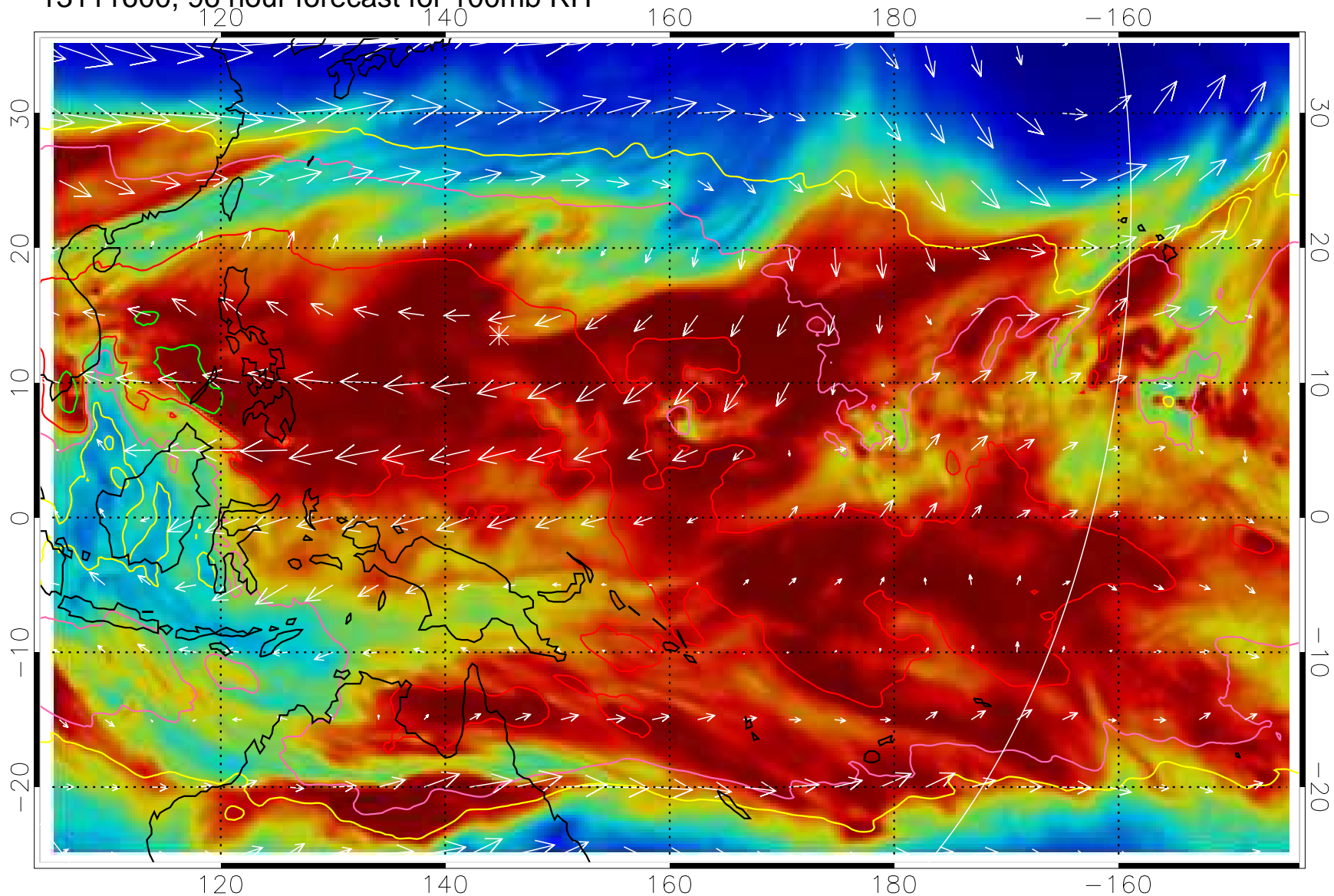
13111600, 96 hour forecast for 100mb RH
