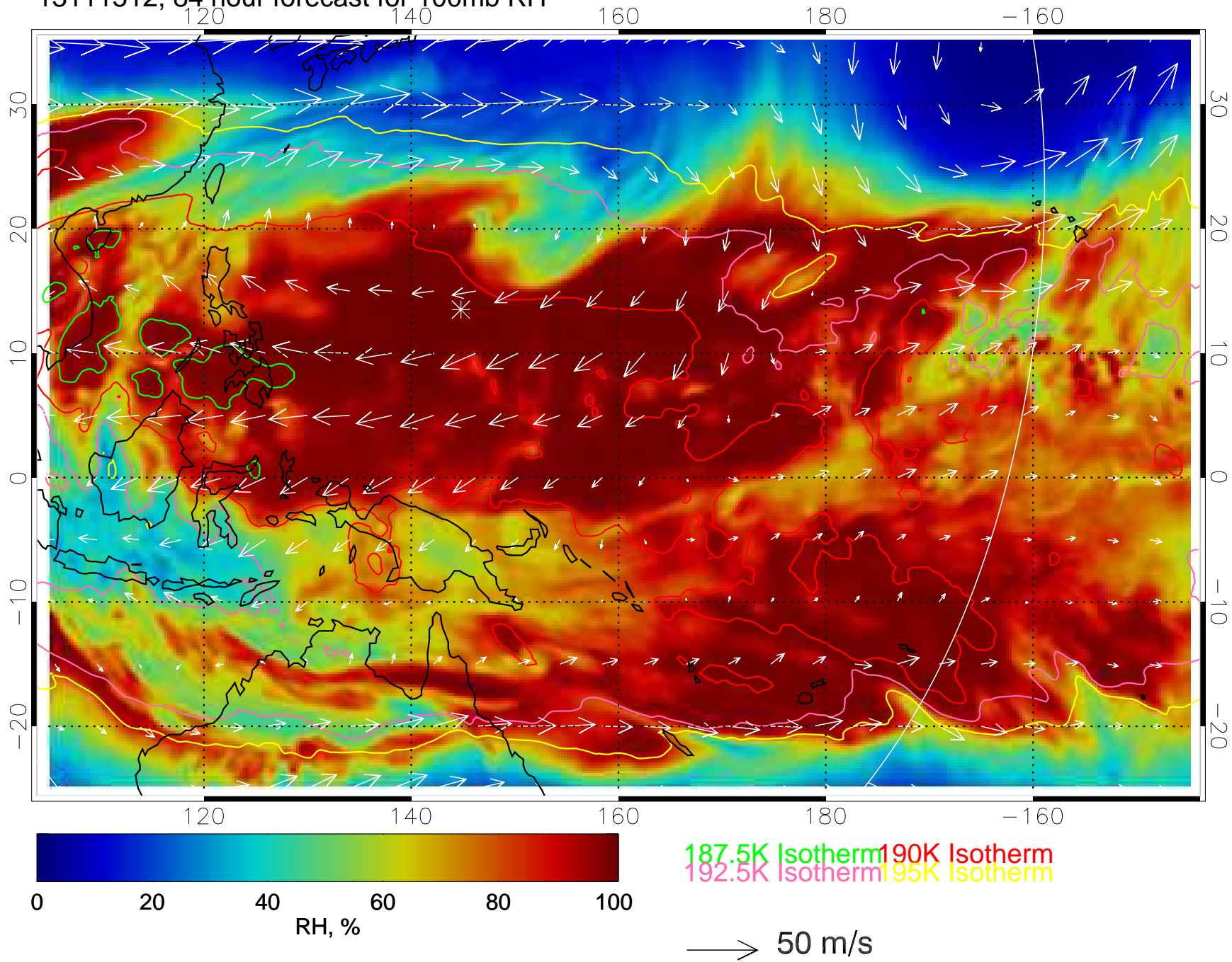
13111512, 84 hour forecast for 100mb RH
