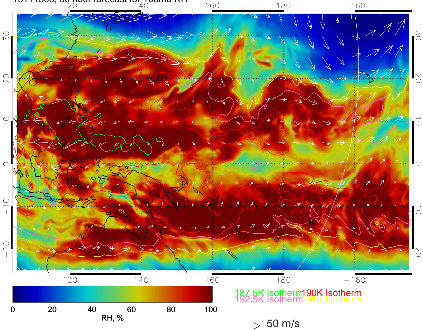
13111306, 30 hour forecast for 100mb RH
