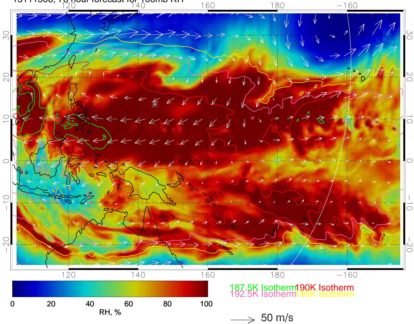
13111506, 78 hour forecast for 100mb RH
