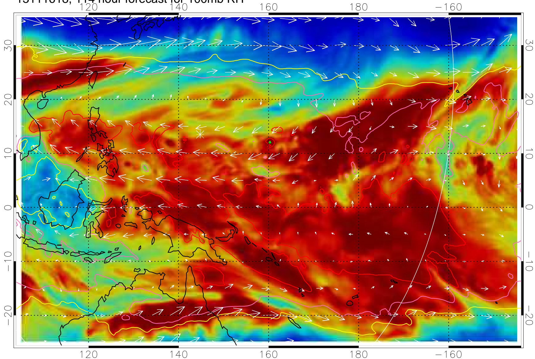
13111618, 114 hour forecast for 100mb RH
