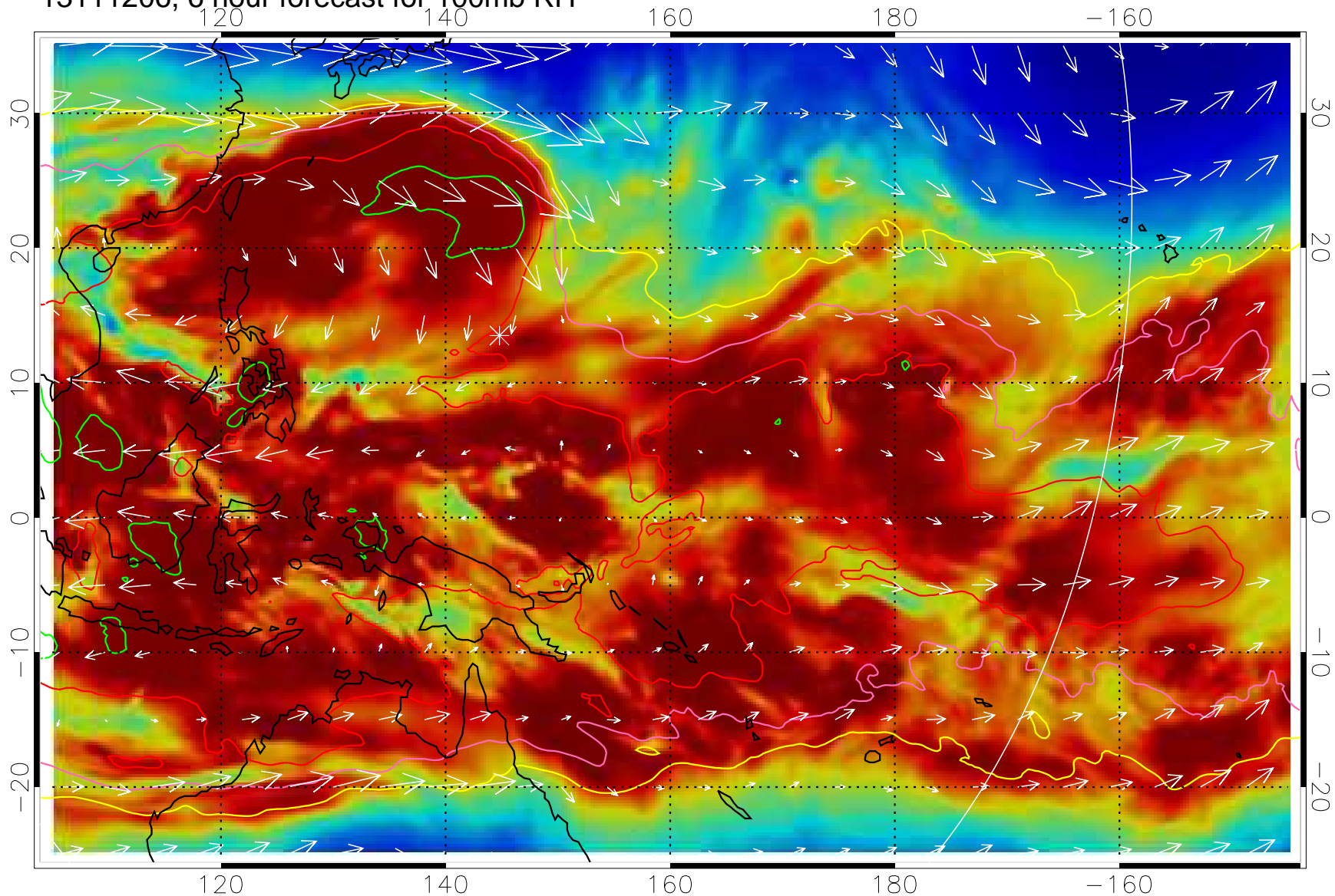
13111206, 6 hour forecast for 100mb RH
