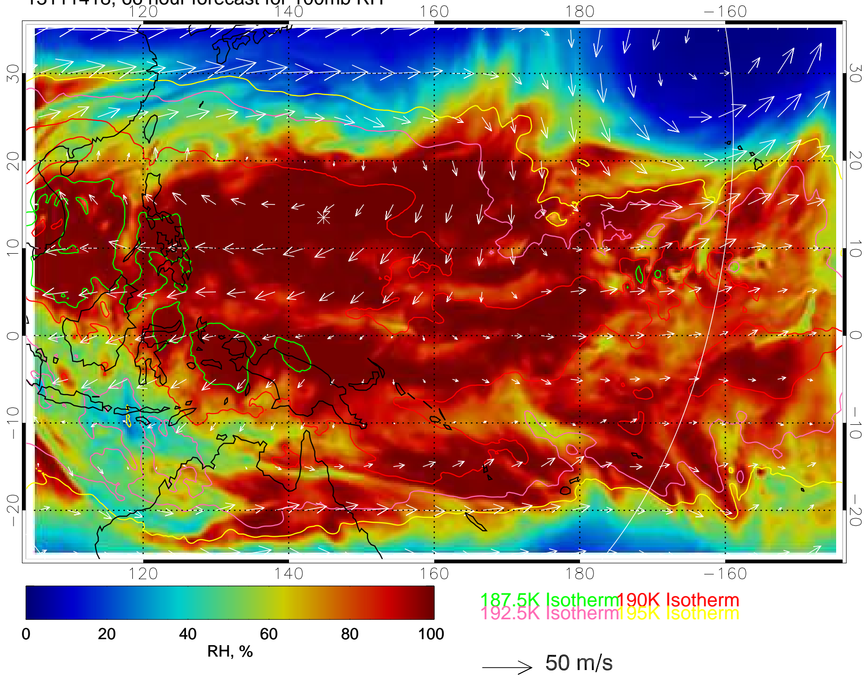
13111418, 66 hour forecast for 100mb RH
