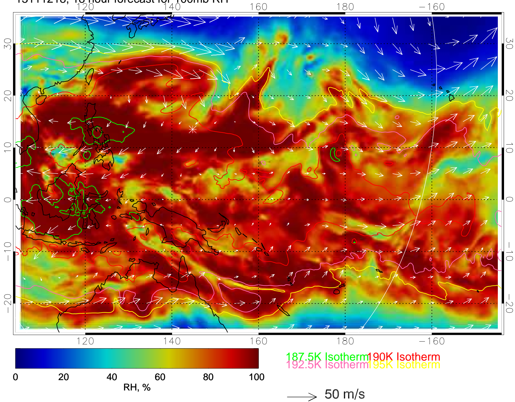
13111218, 18 hour forecast for 100mb RH
