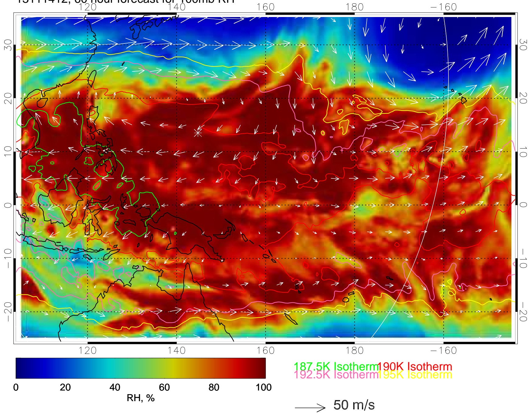
13111412, 60 hour forecast for 100mb RH
