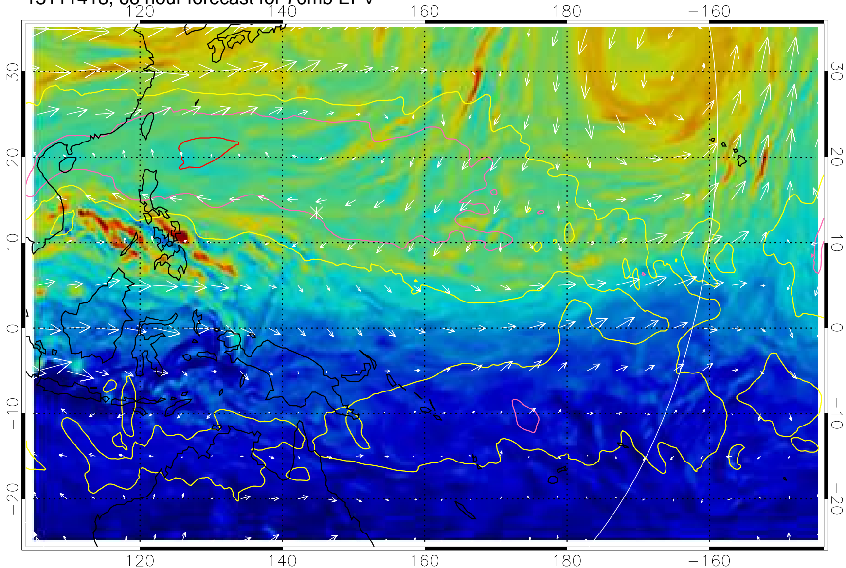
13111418, 66 hour forecast for 70mb EPV
