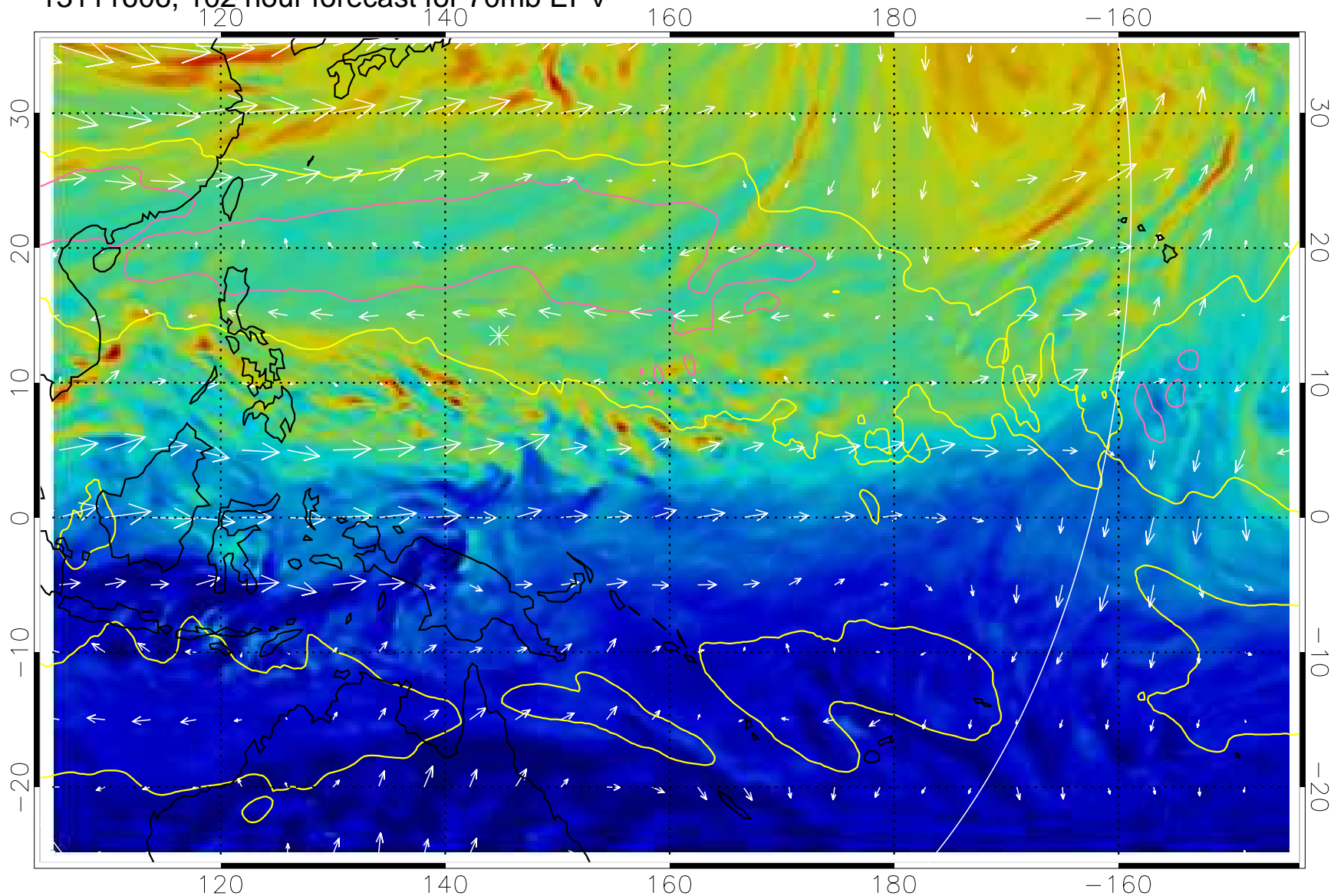
13111606, 102 hour forecast for 70mb EPV
