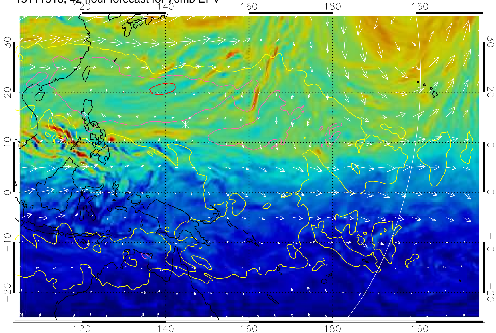
13111318, 42 hour forecast for 70mb EPV
