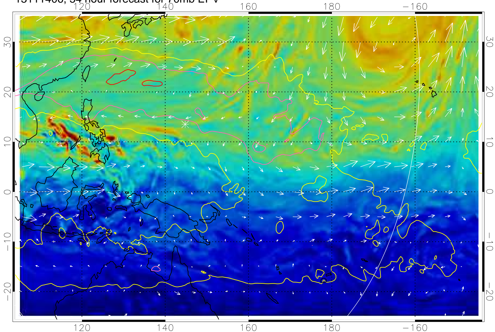
13111406, 54 hour forecast for 70mb EPV
