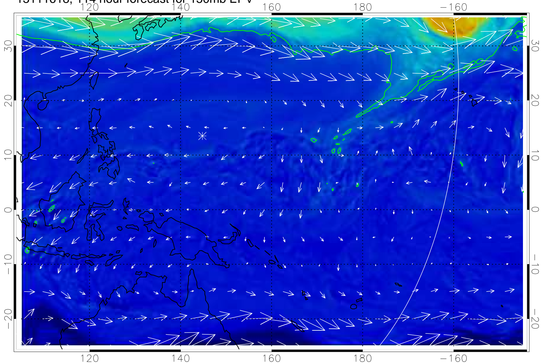
13111618, 114 hour forecast for 150mb EPV
