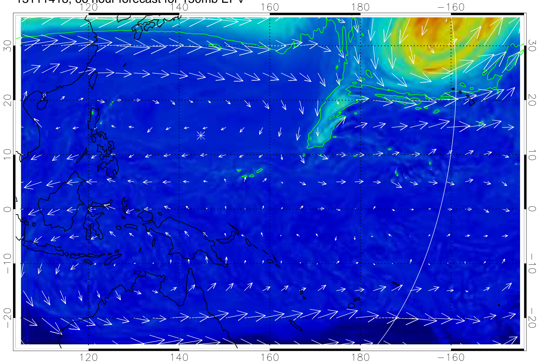
13111418, 66 hour forecast for 150mb EPV
