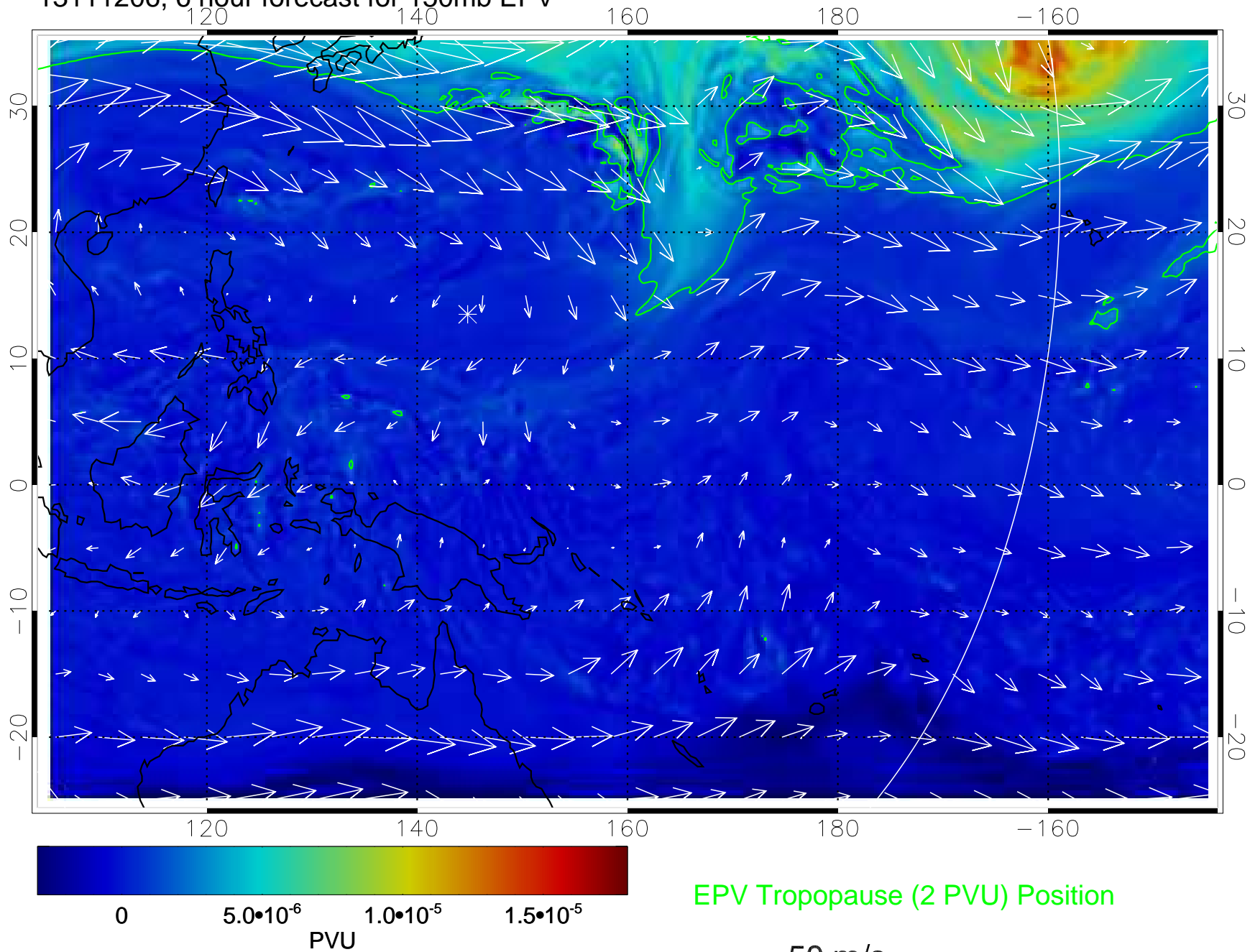
13111206, 6 hour forecast for 150mb EPV
