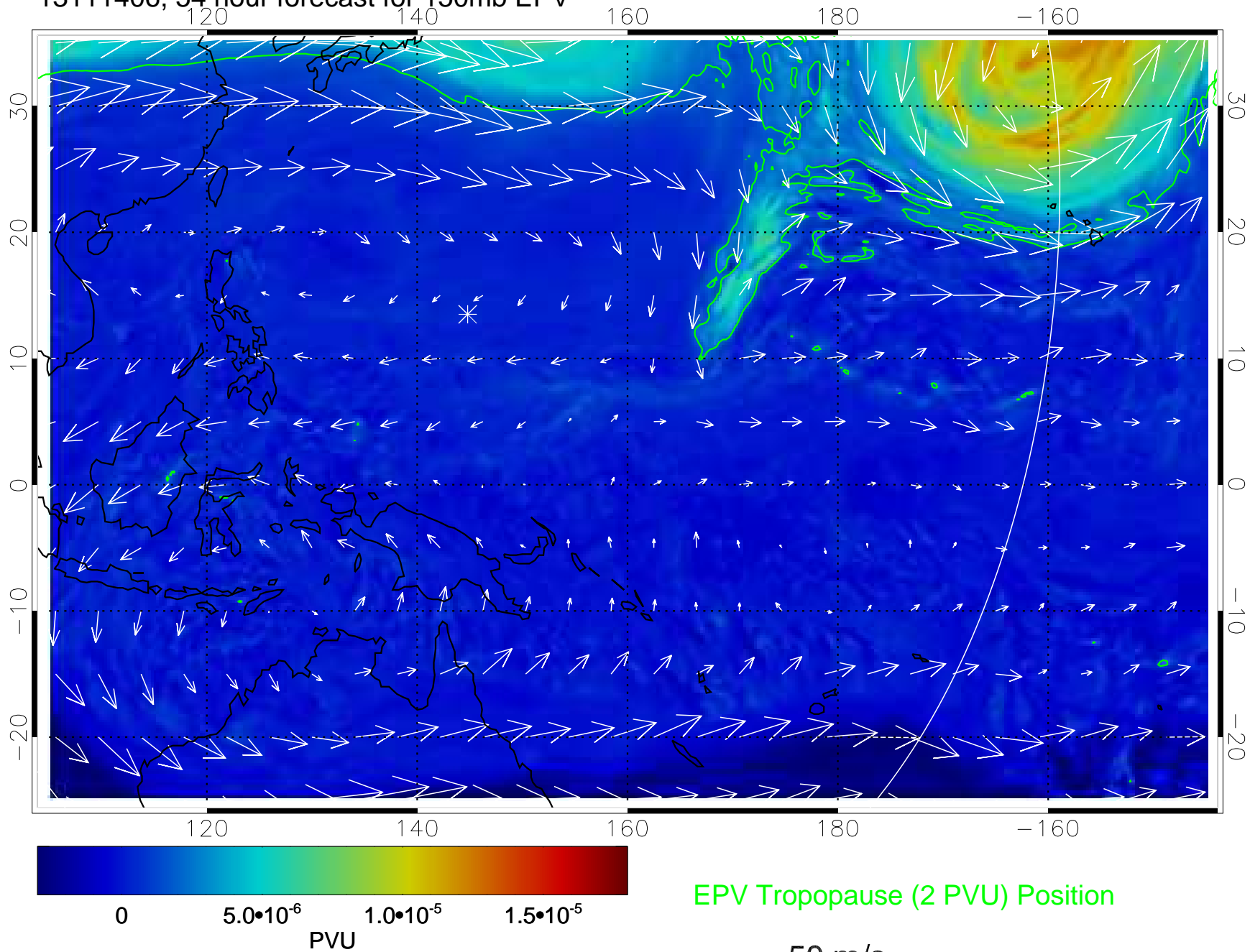
13111406, 54 hour forecast for 150mb EPV
