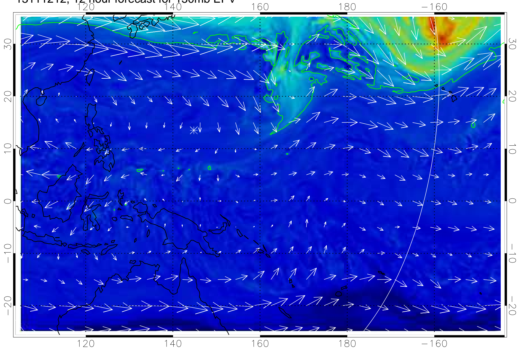
13111212, 12 hour forecast for 150mb EPV
