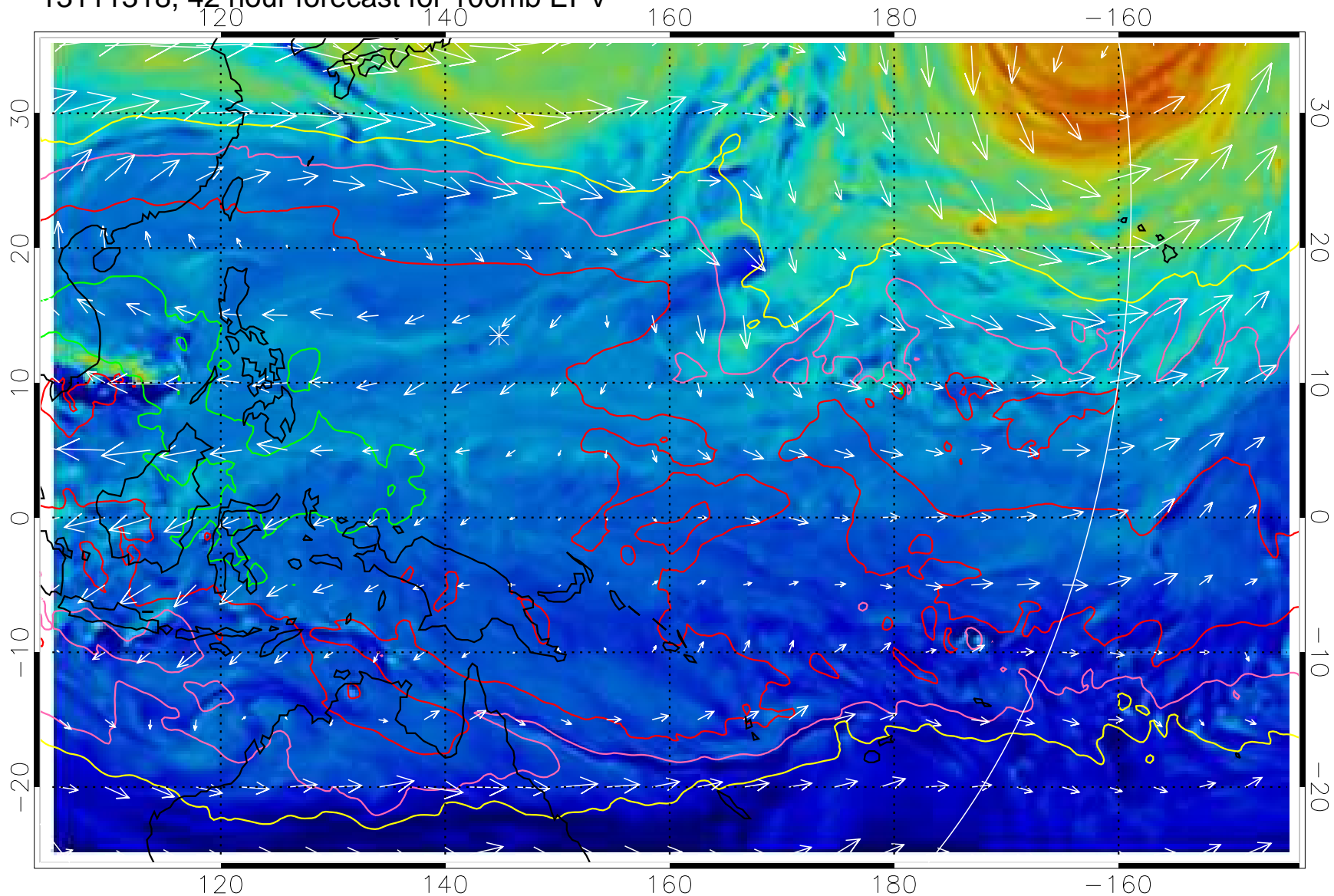
13111318, 42 hour forecast for 100mb EPV
