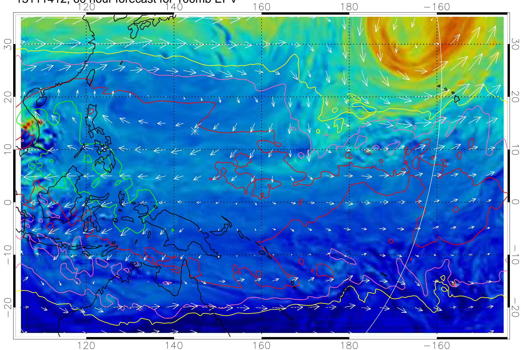
13111412, 60 hour forecast for 100mb EPV
