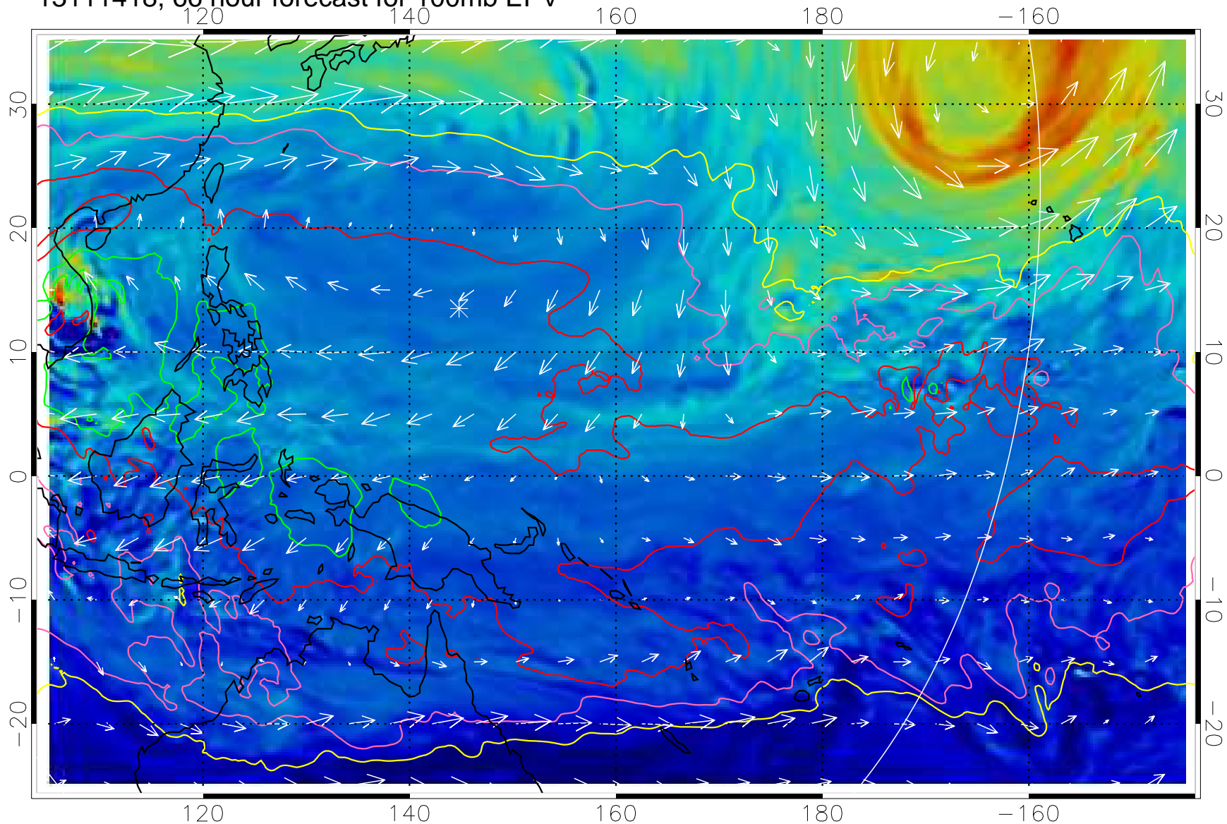
13111418, 66 hour forecast for 100mb EPV
