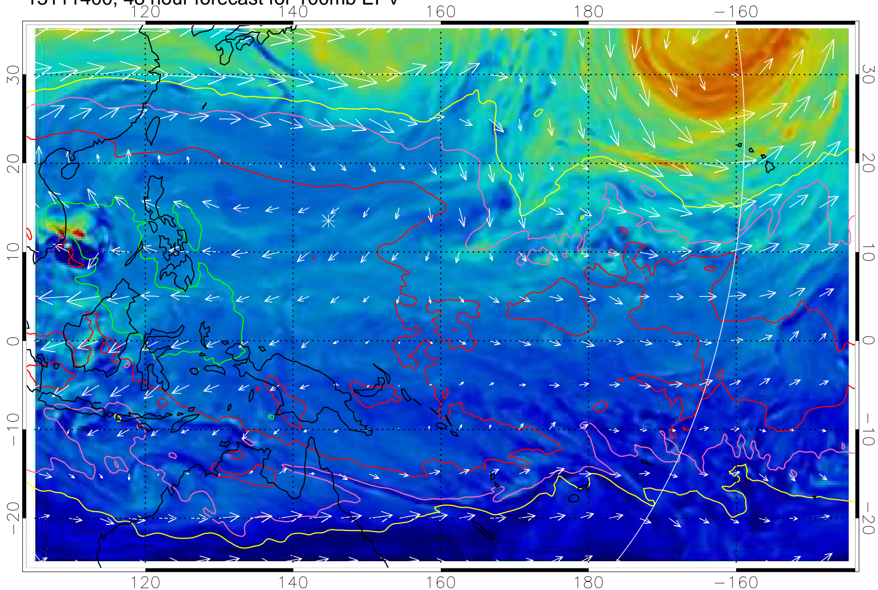
13111400, 48 hour forecast for 100mb EPV
