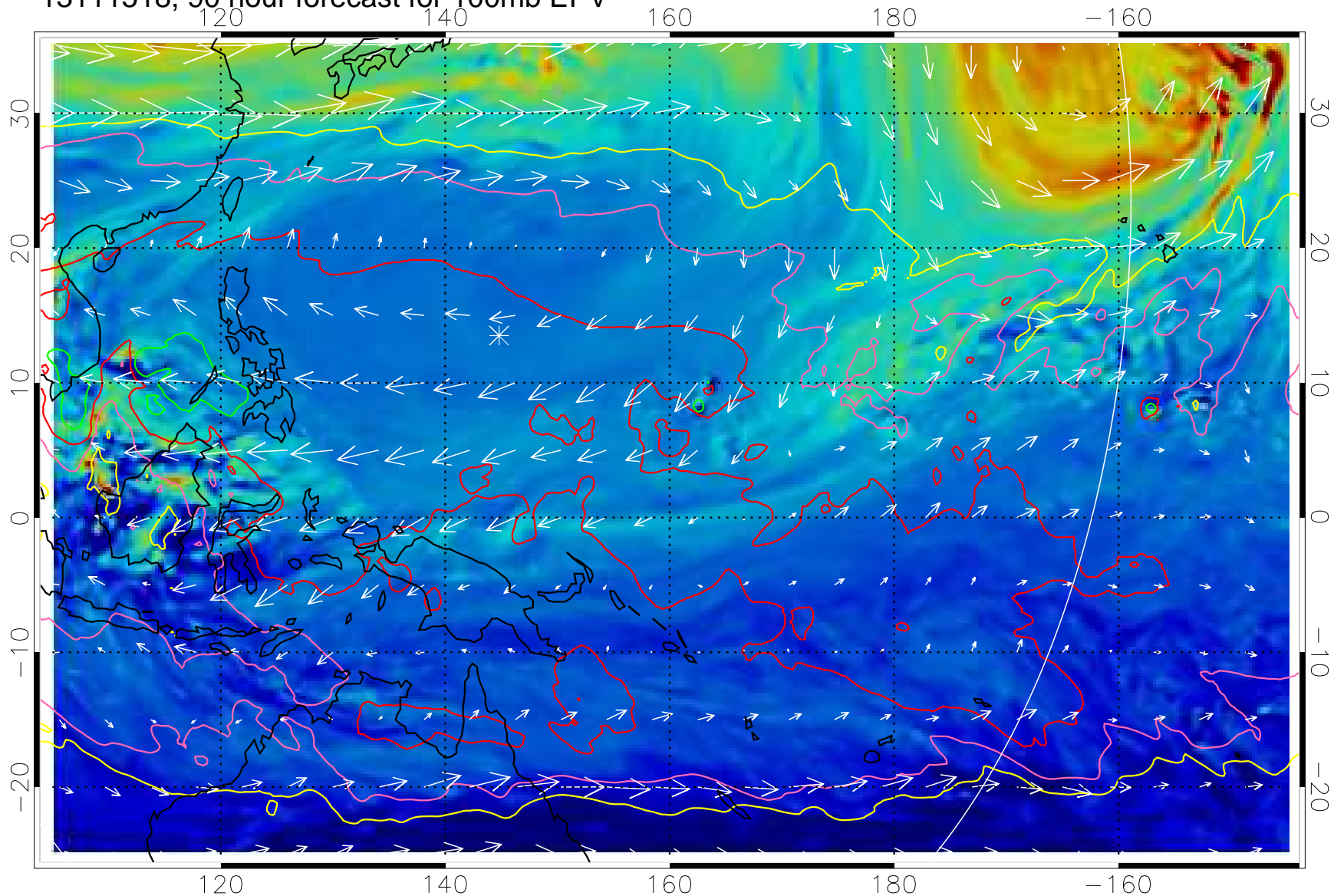
13111518, 90 hour forecast for 100mb EPV
