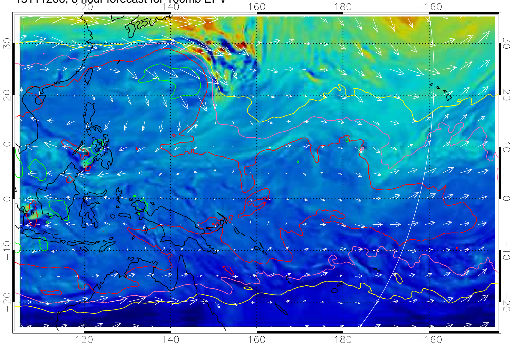
13111206, 6 hour forecast for 100mb EPV
