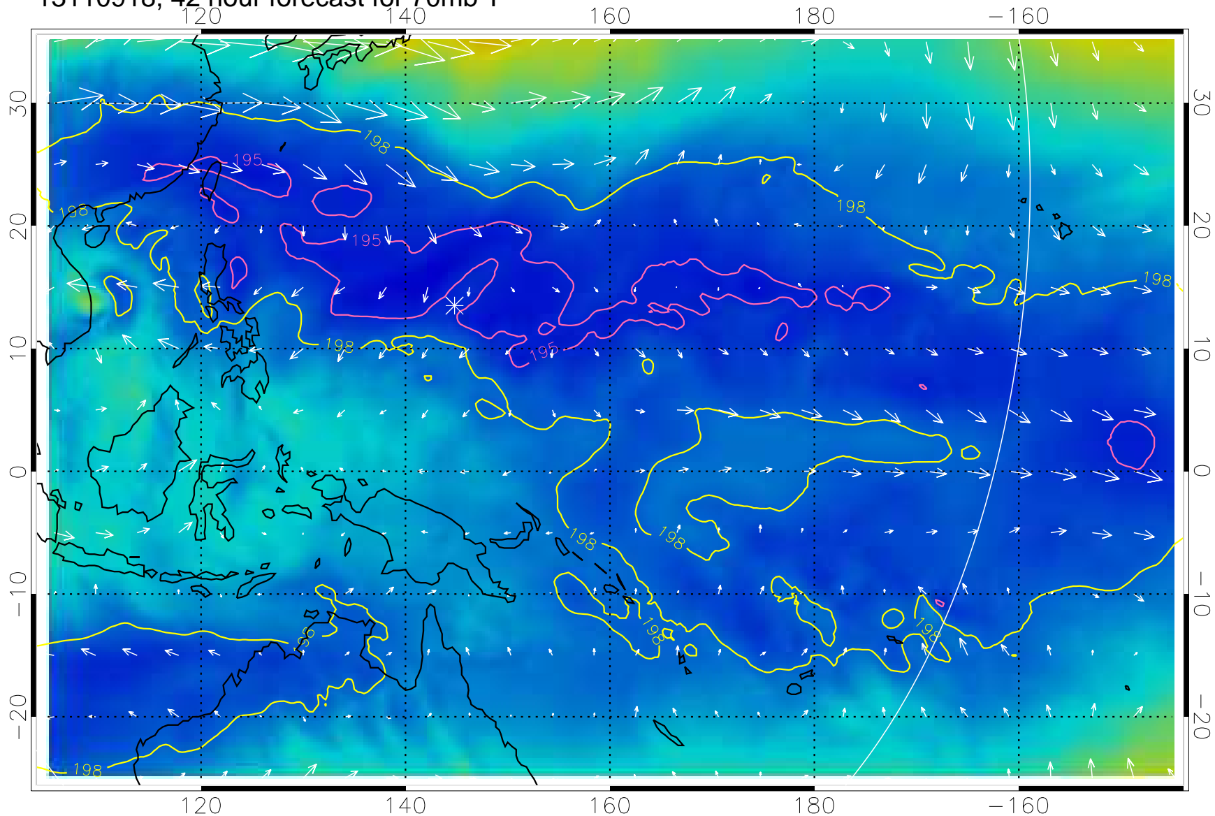
13110918, 42 hour forecast for 70mb T
