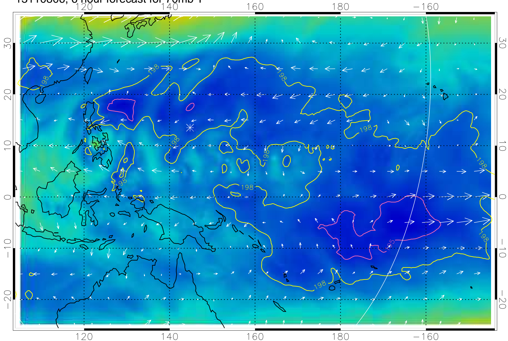
13110806, 6 hour forecast for 70mb T
