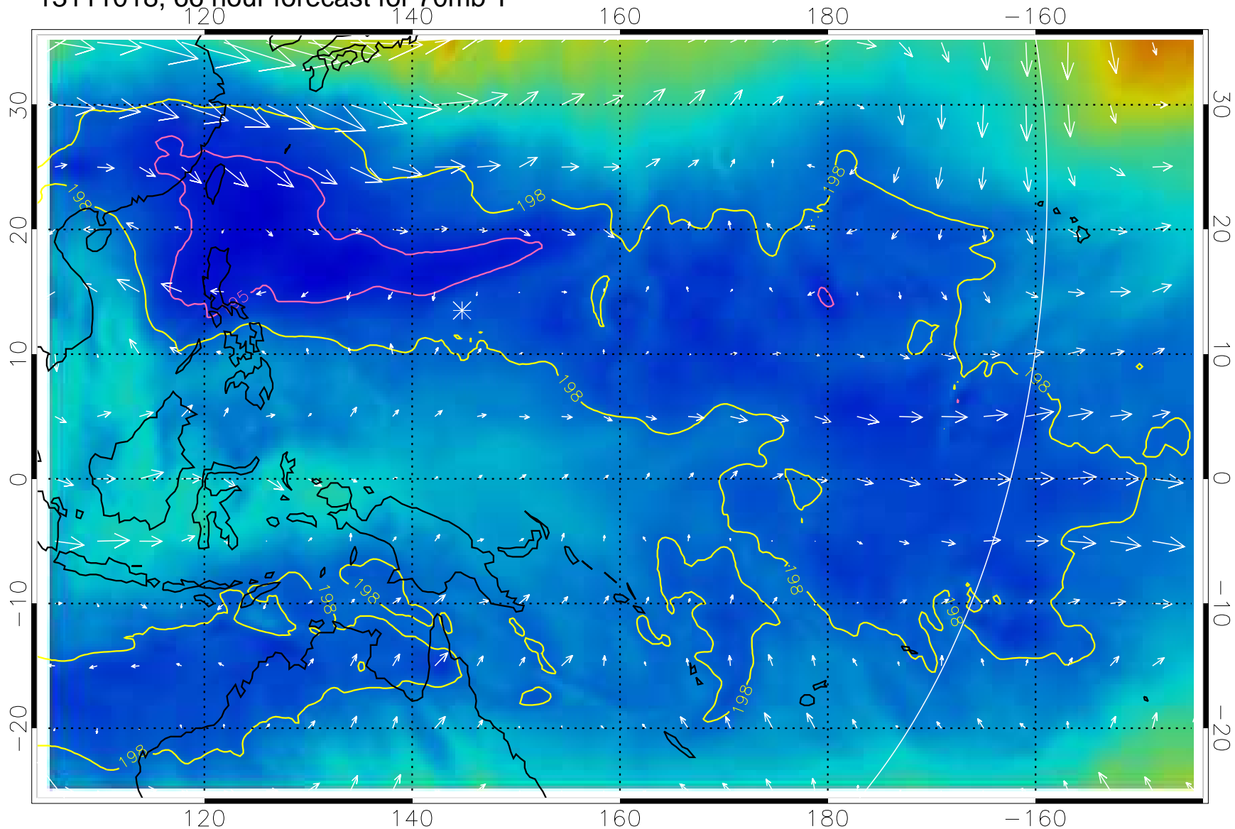
13111018, 66 hour forecast for 70mb T
