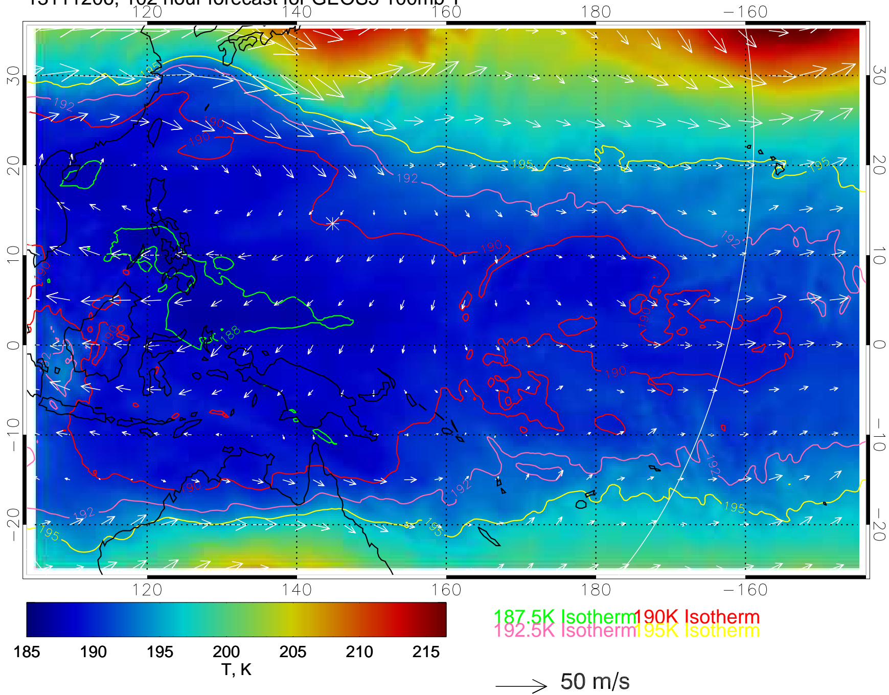
13111206, 102 hour forecast for GEOS5 100mb T
