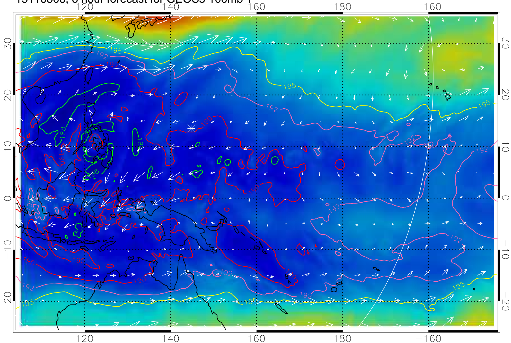
13110806, 6 hour forecast for GEOS5 100mb T
