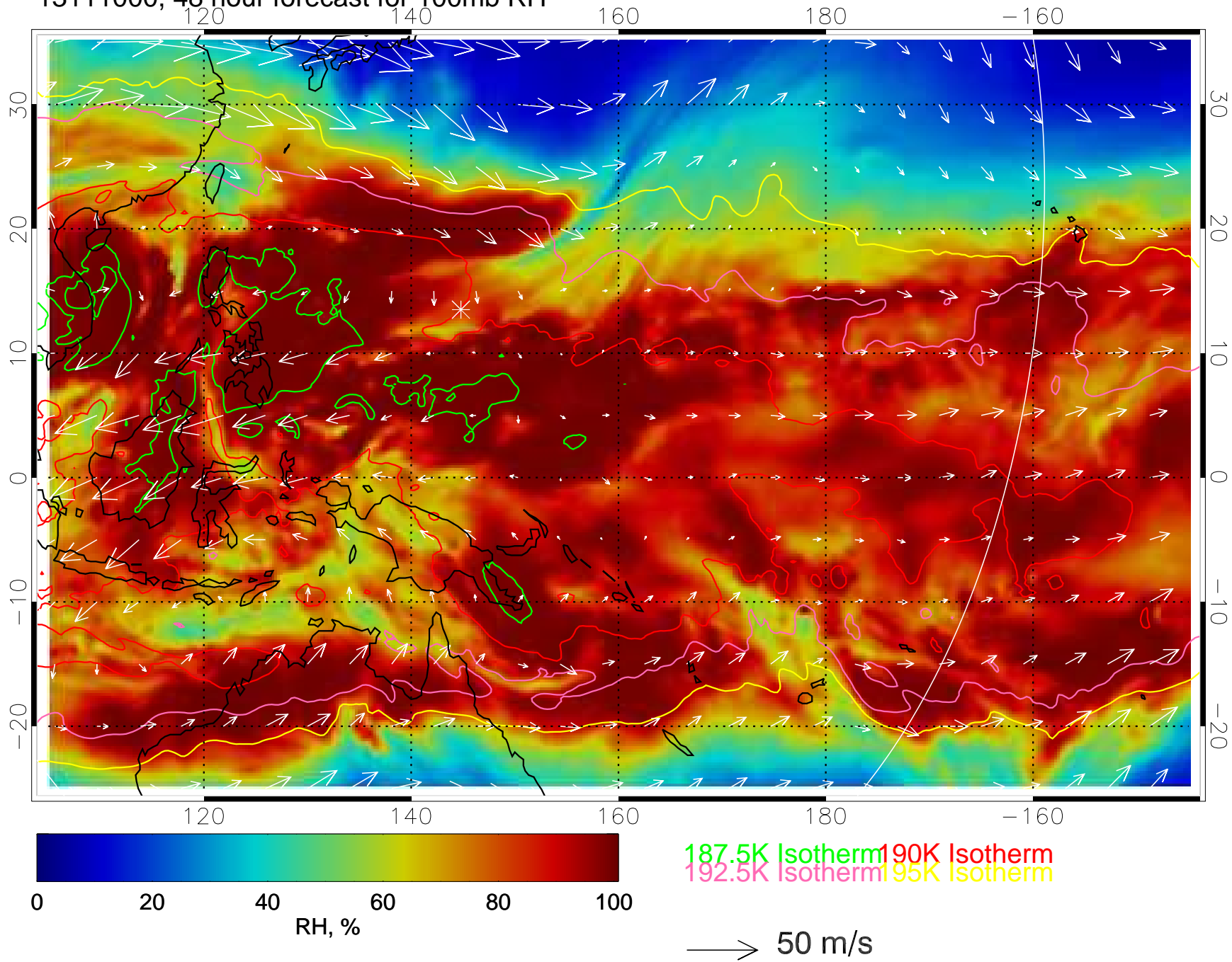
13111000, 48 hour forecast for 100mb RH
