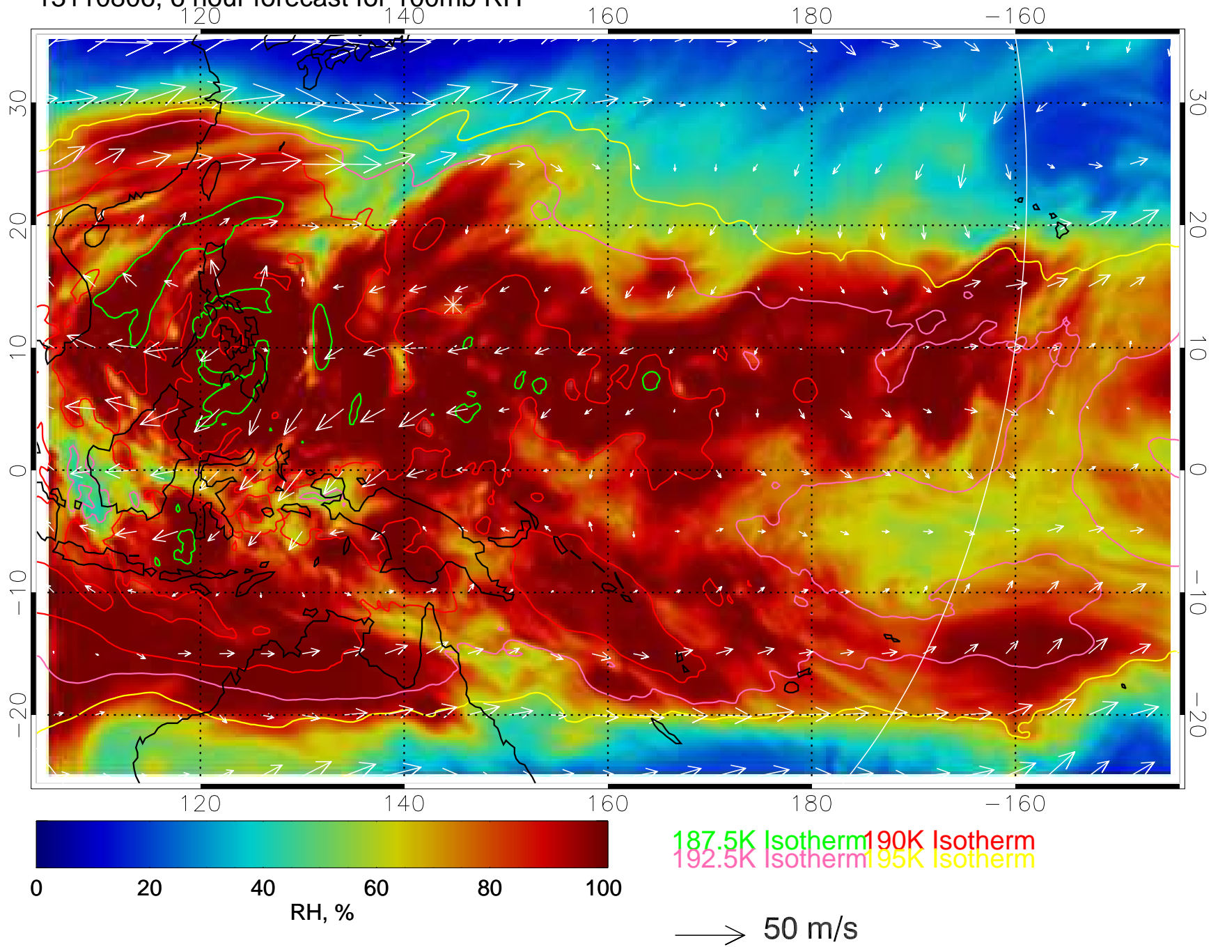
13110806, 6 hour forecast for 100mb RH
