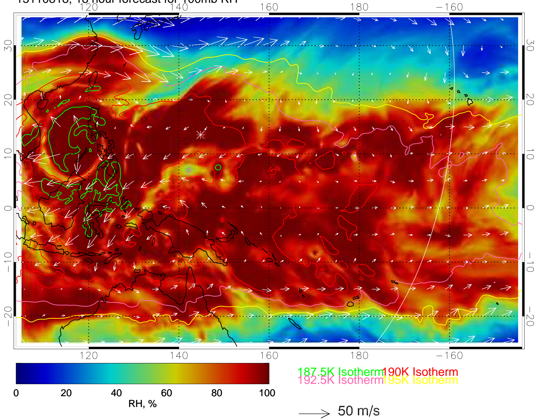
13110818, 18 hour forecast for 100mb RH
