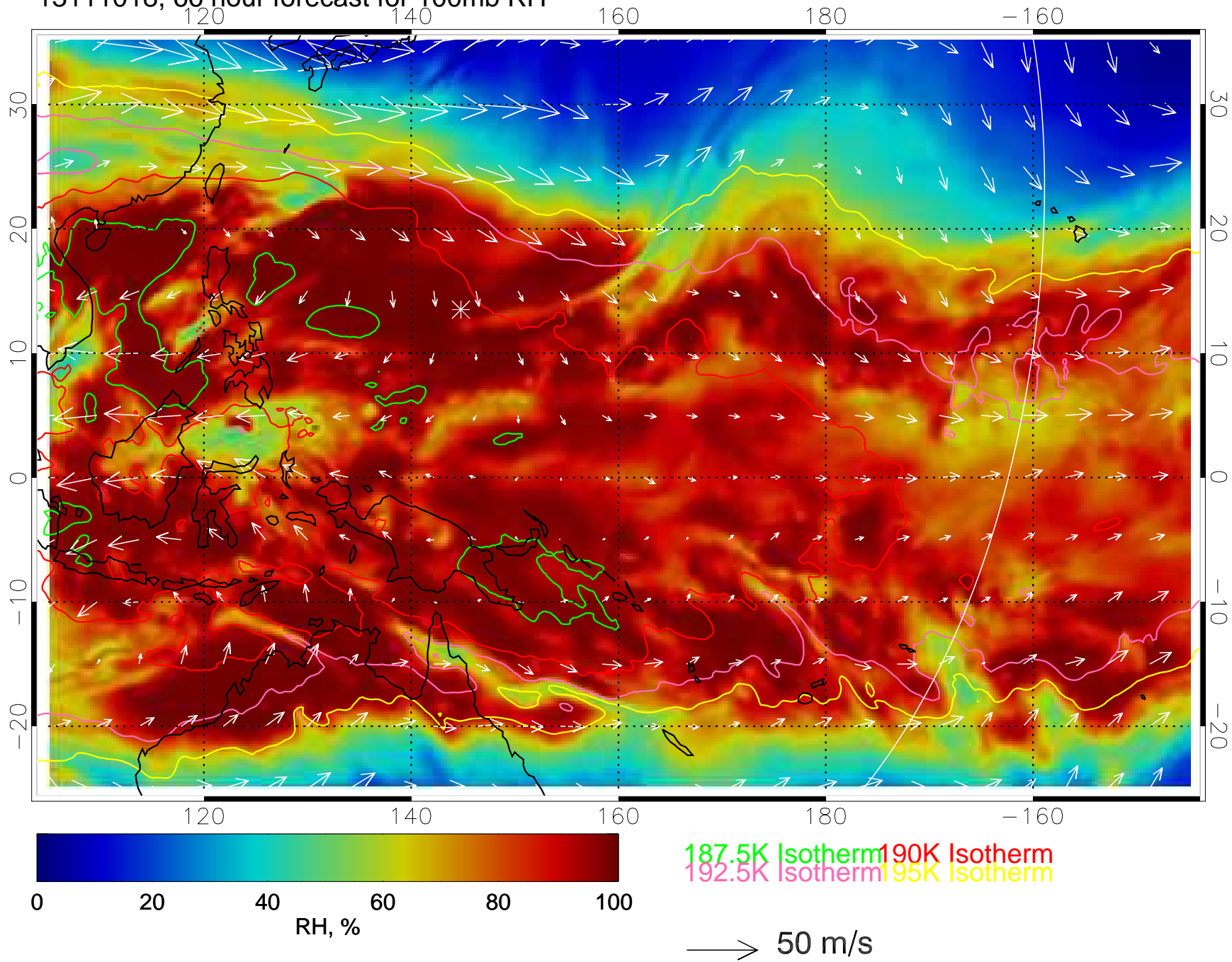
13111018, 66 hour forecast for 100mb RH
