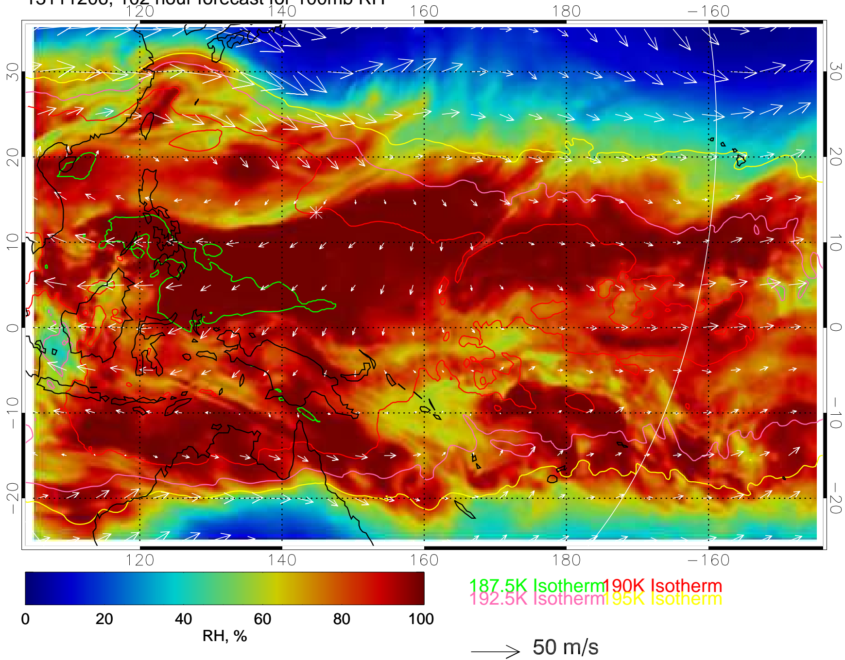
13111206, 102 hour forecast for 100mb RH
