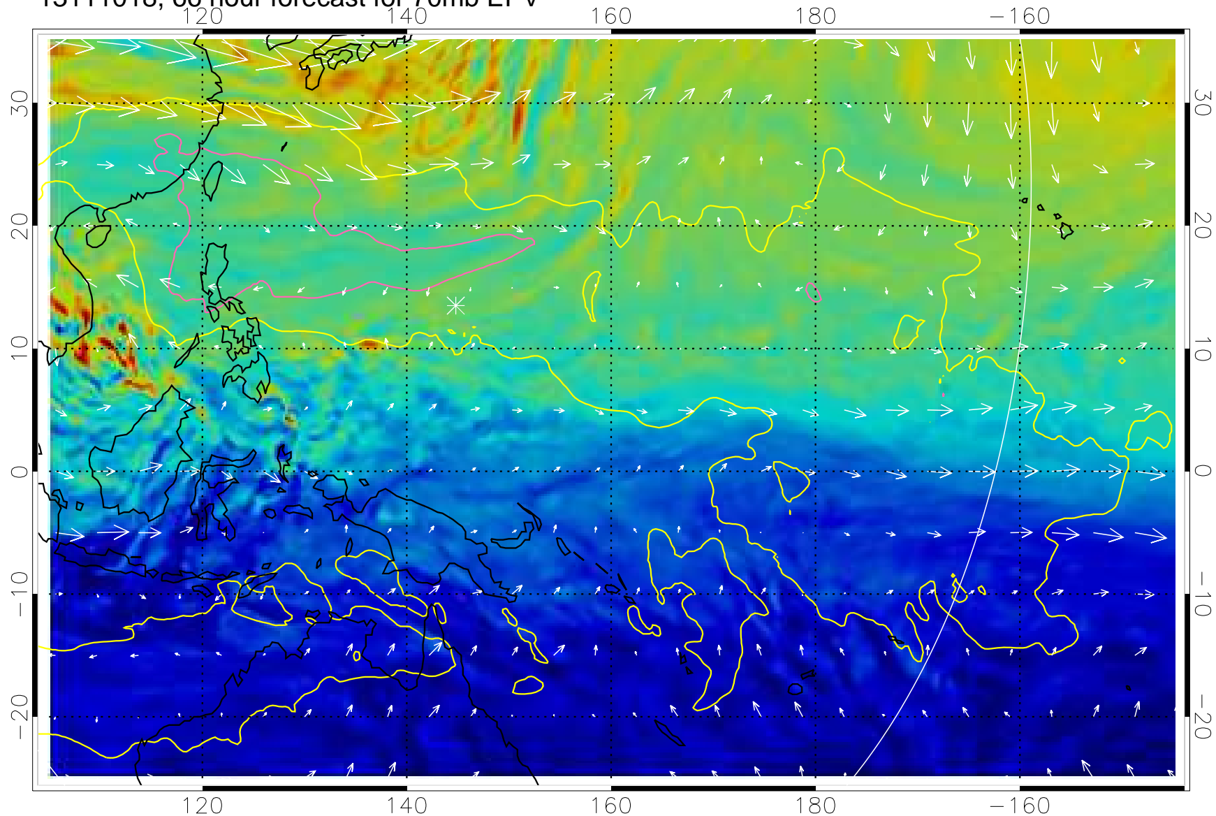
13111018, 66 hour forecast for 70mb EPV
