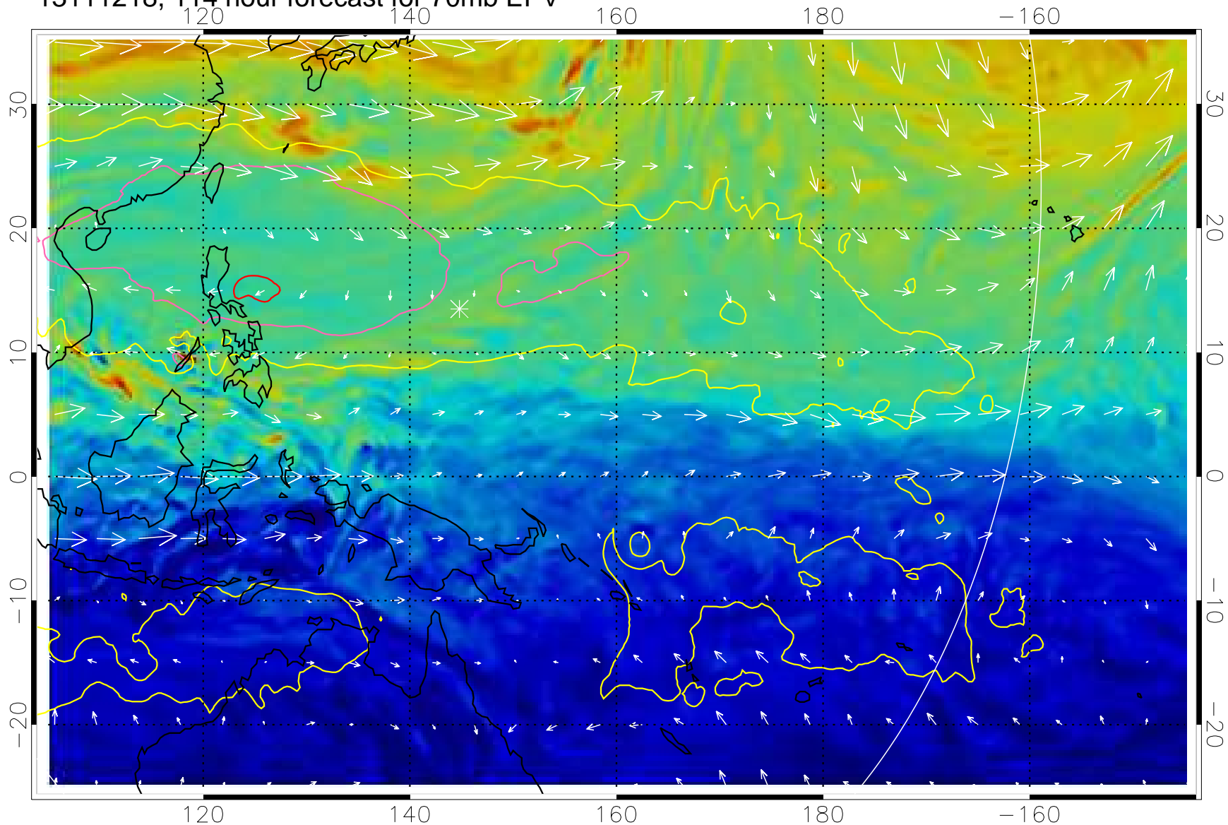
13111218, 114 hour forecast for 70mb EPV
