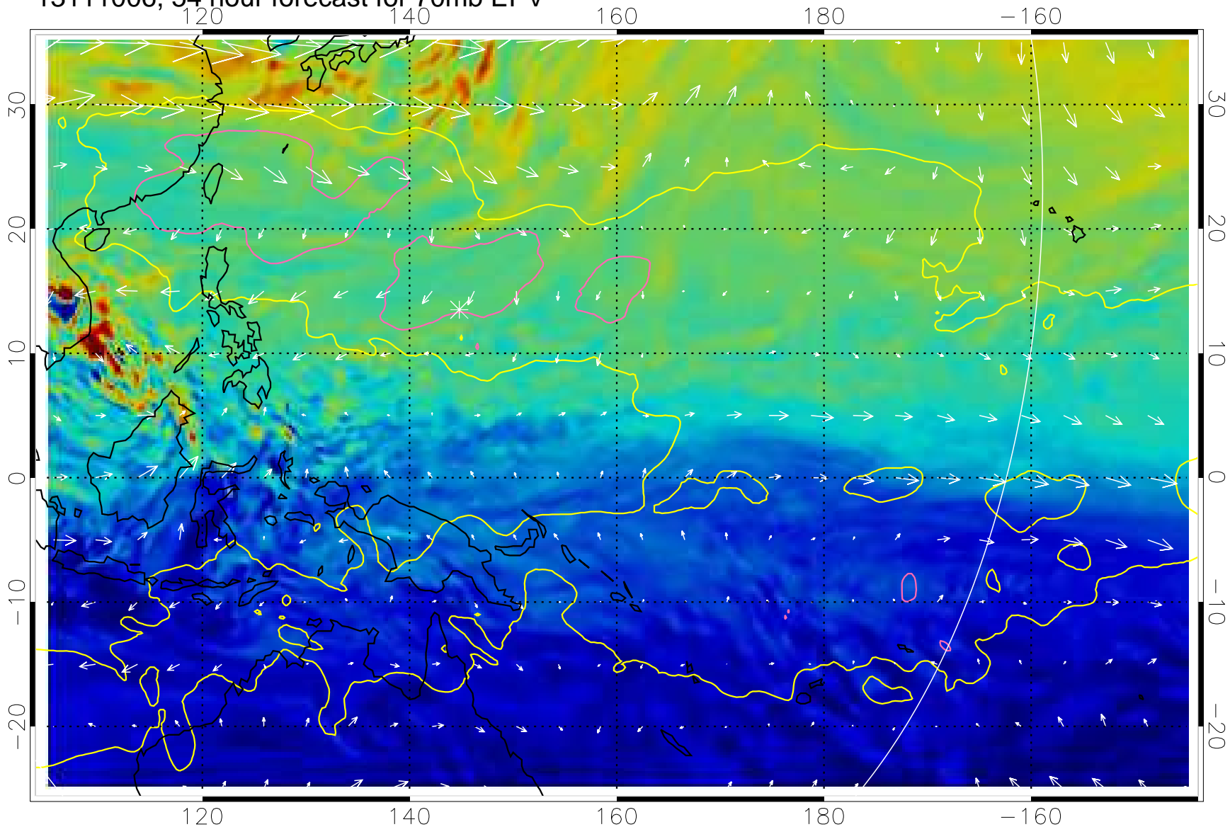
13111006, 54 hour forecast for 70mb EPV
