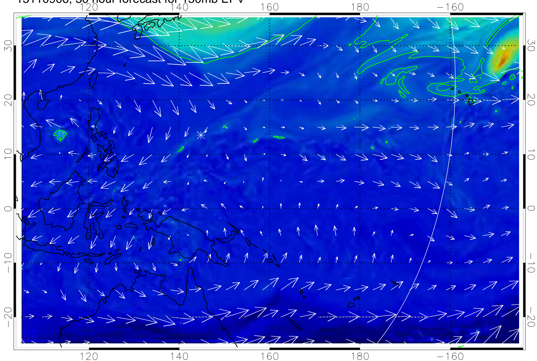
13110906, 30 hour forecast for 150mb EPV
