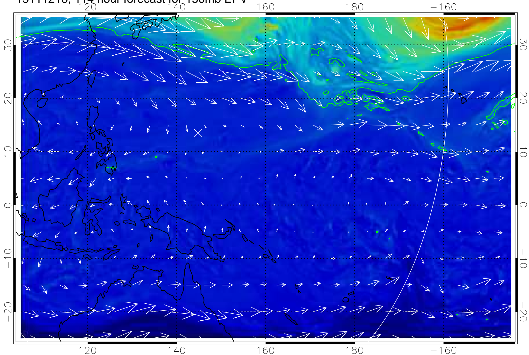
13111218, 114 hour forecast for 150mb EPV
