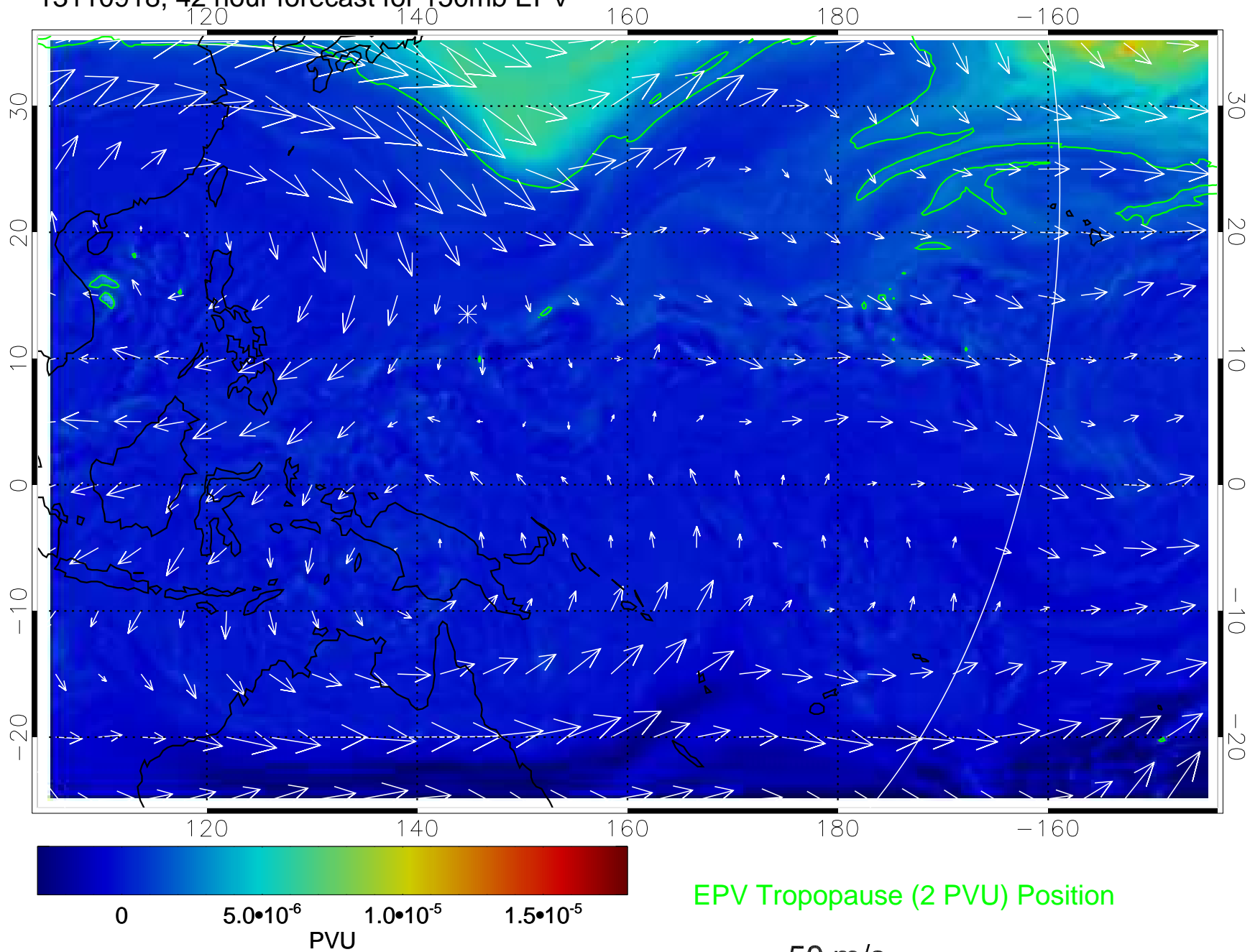
13110918, 42 hour forecast for 150mb EPV
