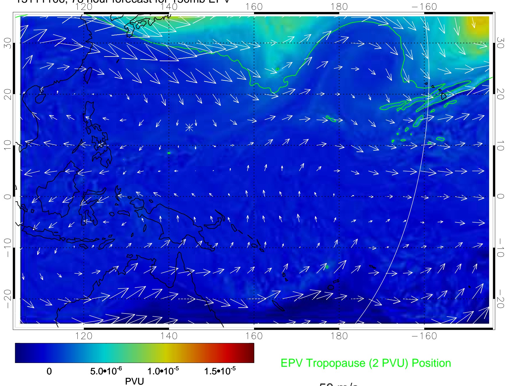
13111106, 78 hour forecast for 150mb EPV
