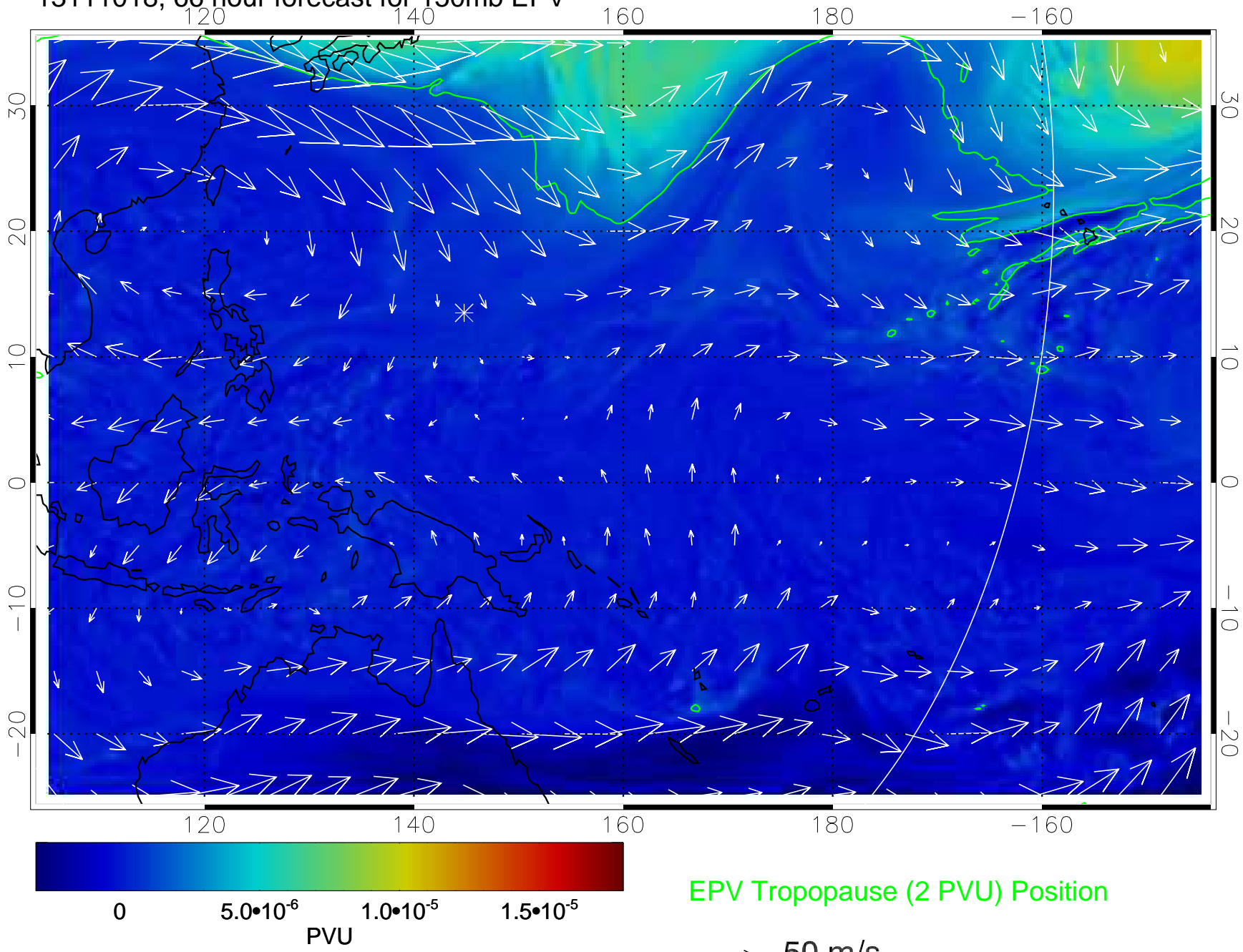
13111018, 66 hour forecast for 150mb EPV
