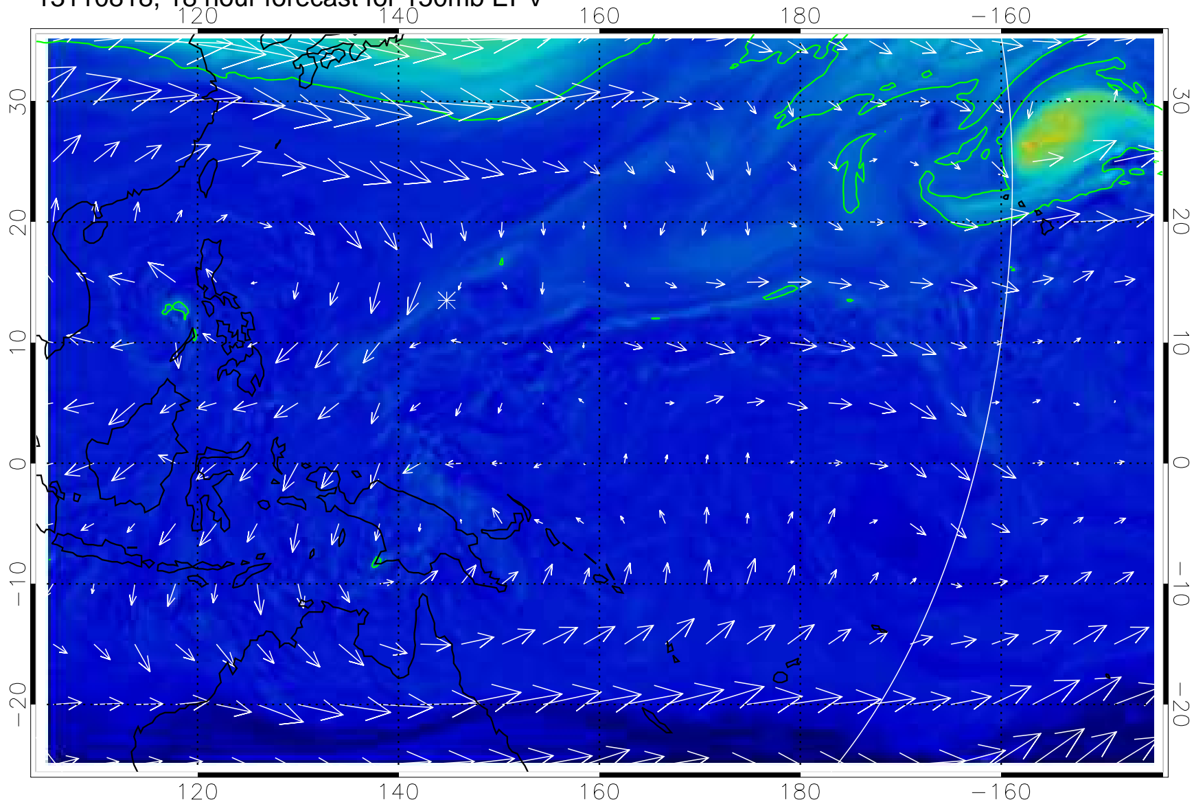
13110818, 18 hour forecast for 150mb EPV
