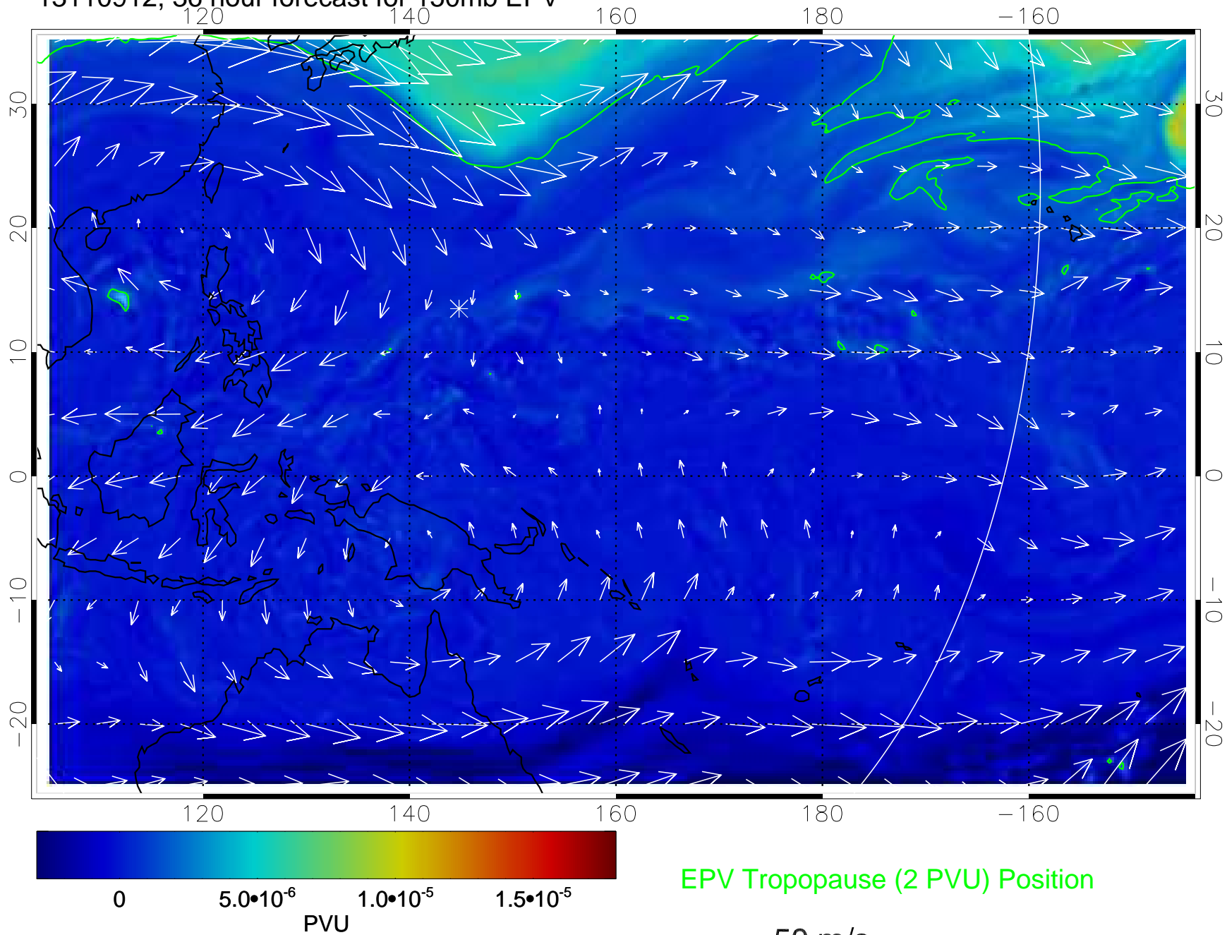
13110912, 36 hour forecast for 150mb EPV
