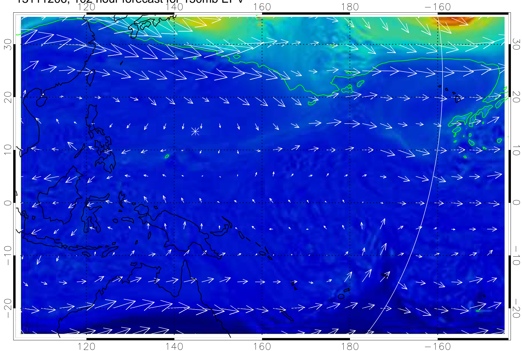
13111206, 102 hour forecast for 150mb EPV
