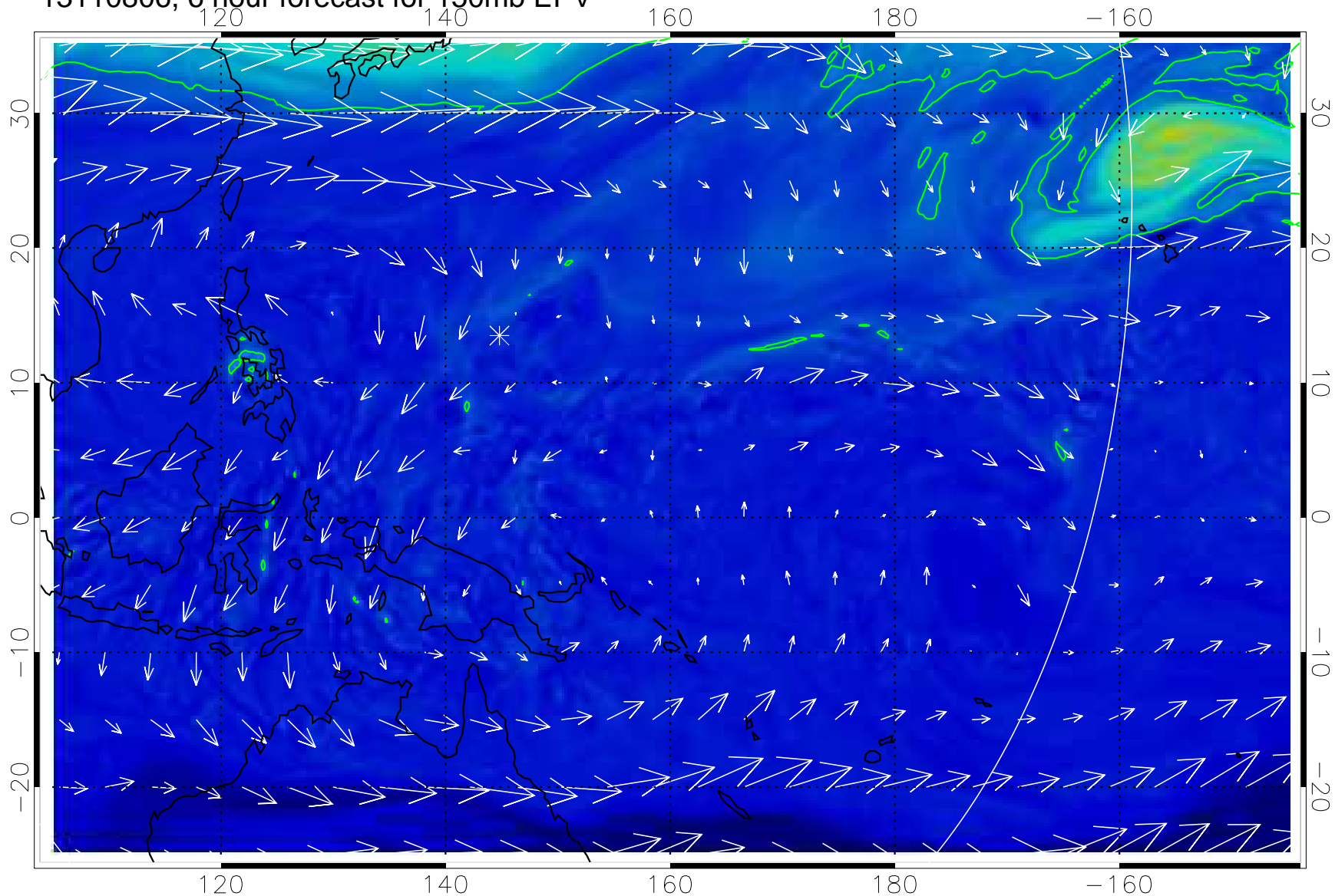
13110806, 6 hour forecast for 150mb EPV
