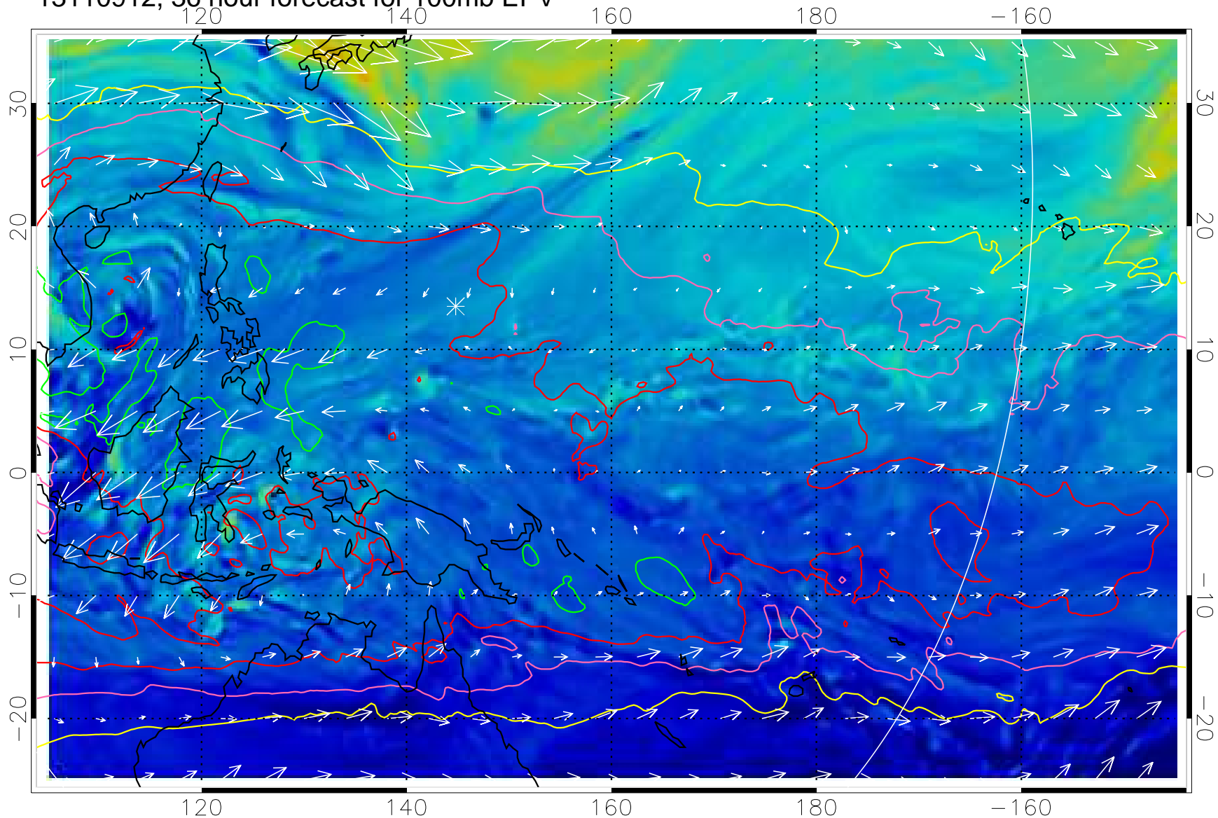
13110912, 36 hour forecast for 100mb EPV
