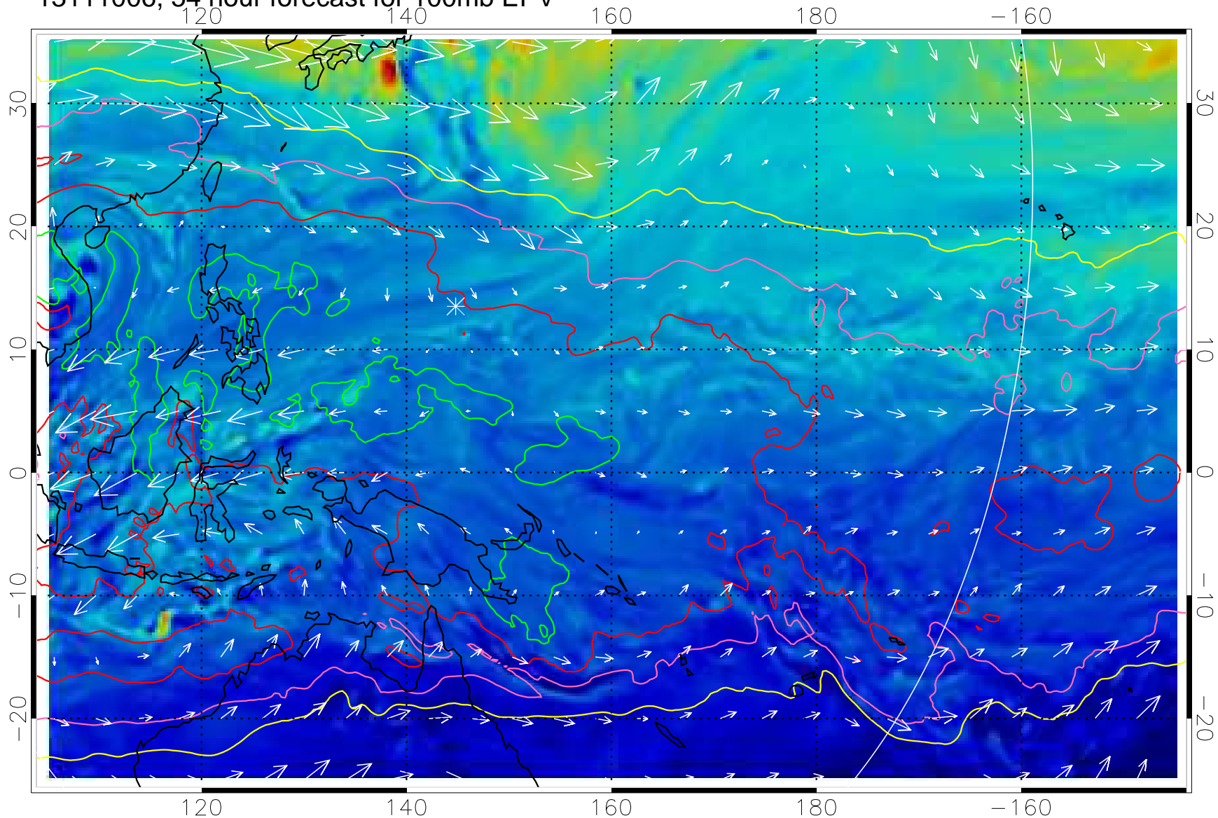
13111006, 54 hour forecast for 100mb EPV
