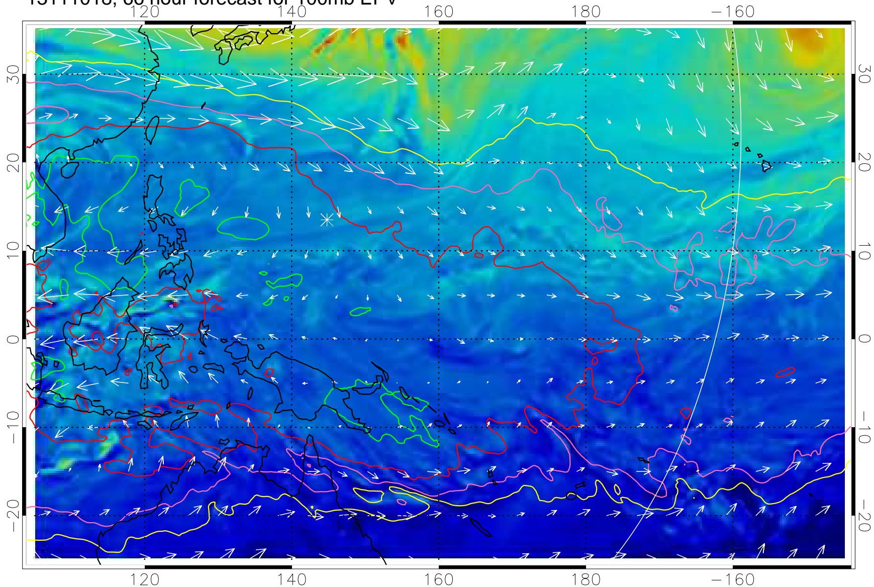
13111018, 66 hour forecast for 100mb EPV
