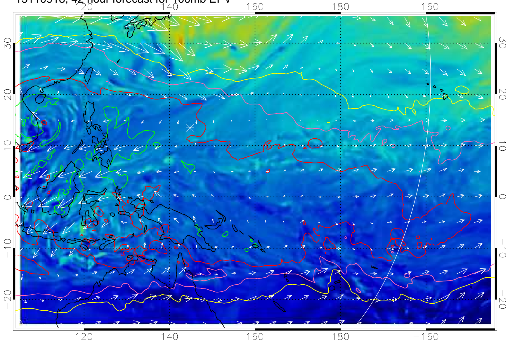
13110918, 42 hour forecast for 100mb EPV
