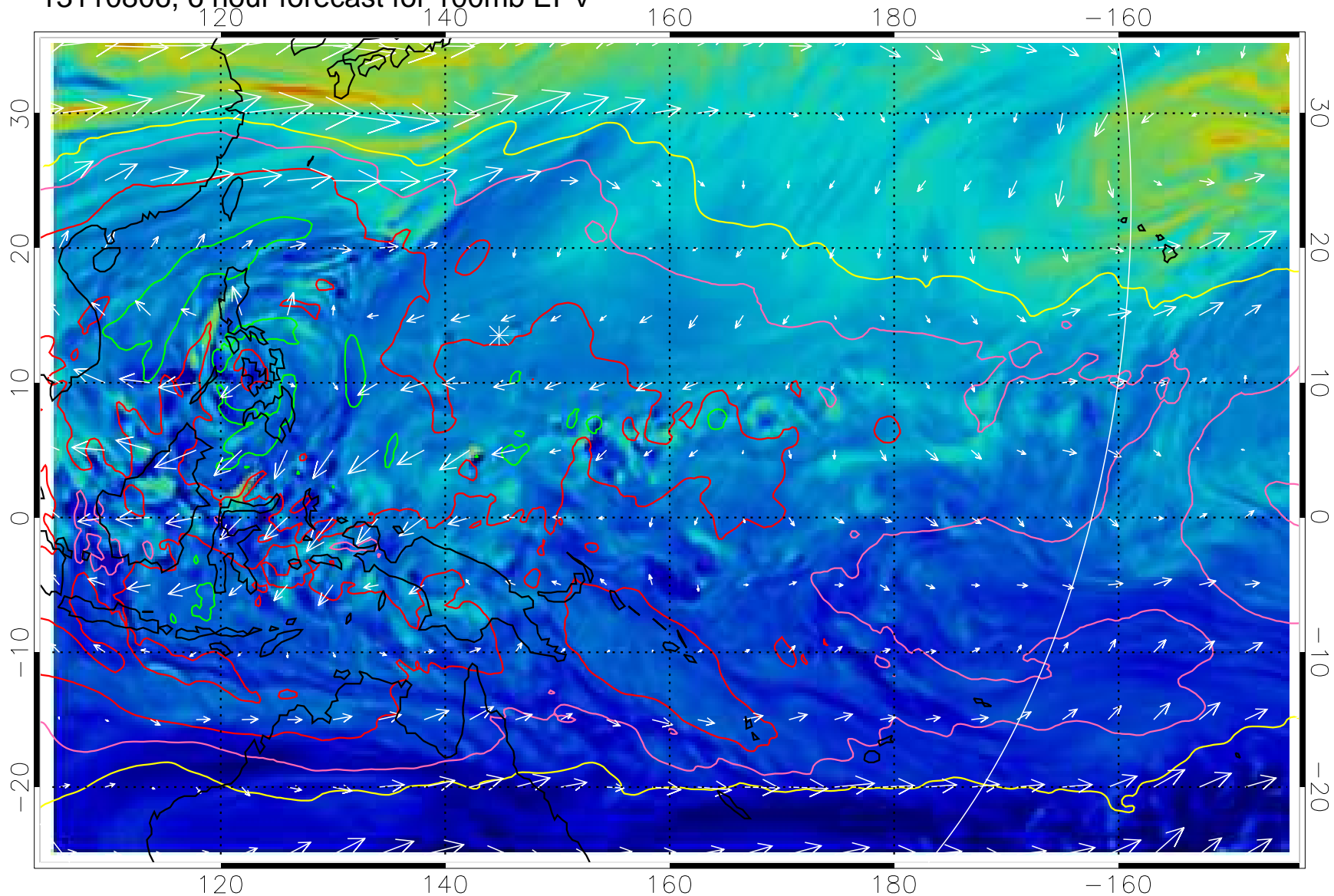
13110806, 6 hour forecast for 100mb EPV
