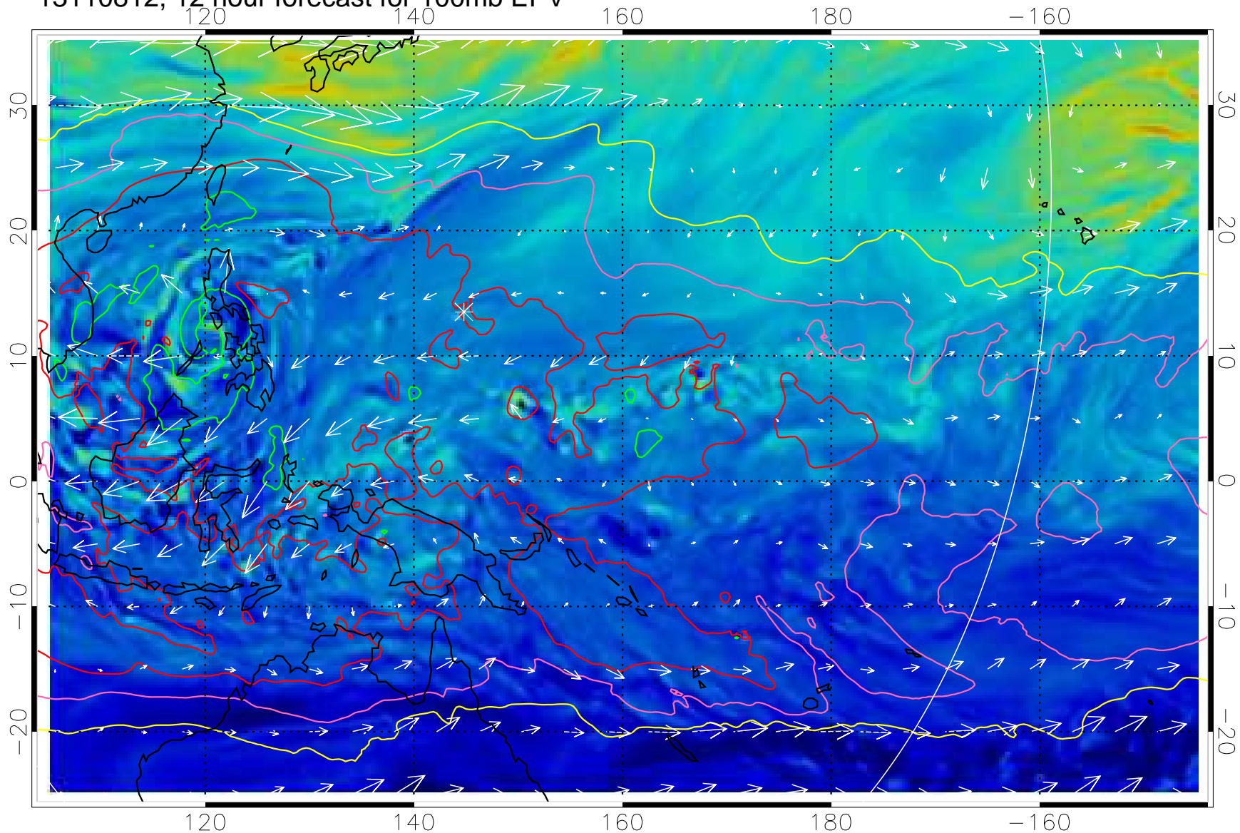
13110812, 12 hour forecast for 100mb EPV
