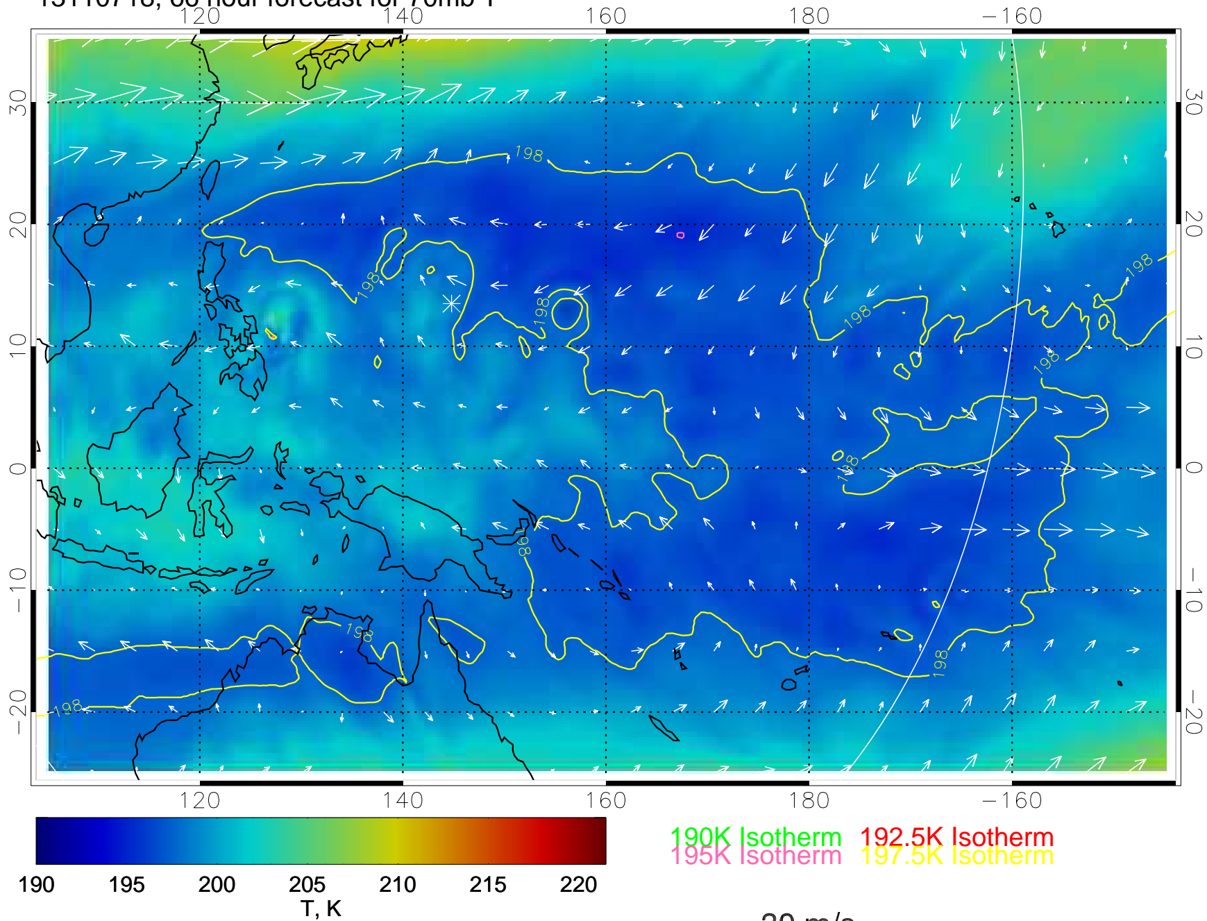
13110718, 66 hour forecast for 70mb T
