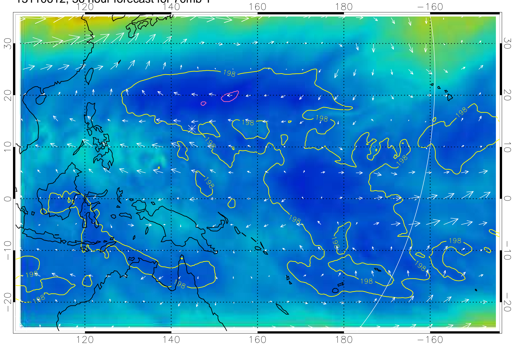
13110612, 36 hour forecast for 70mb T
