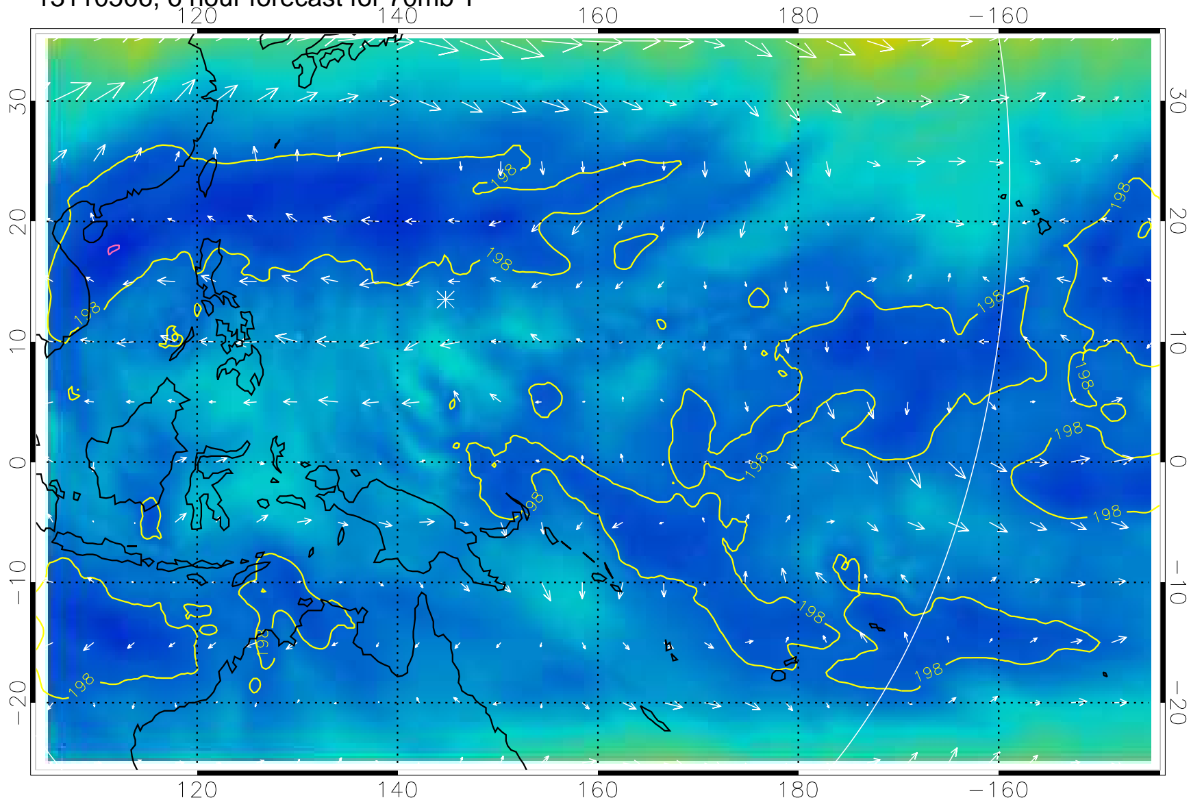
13110506, 6 hour forecast for 70mb T
