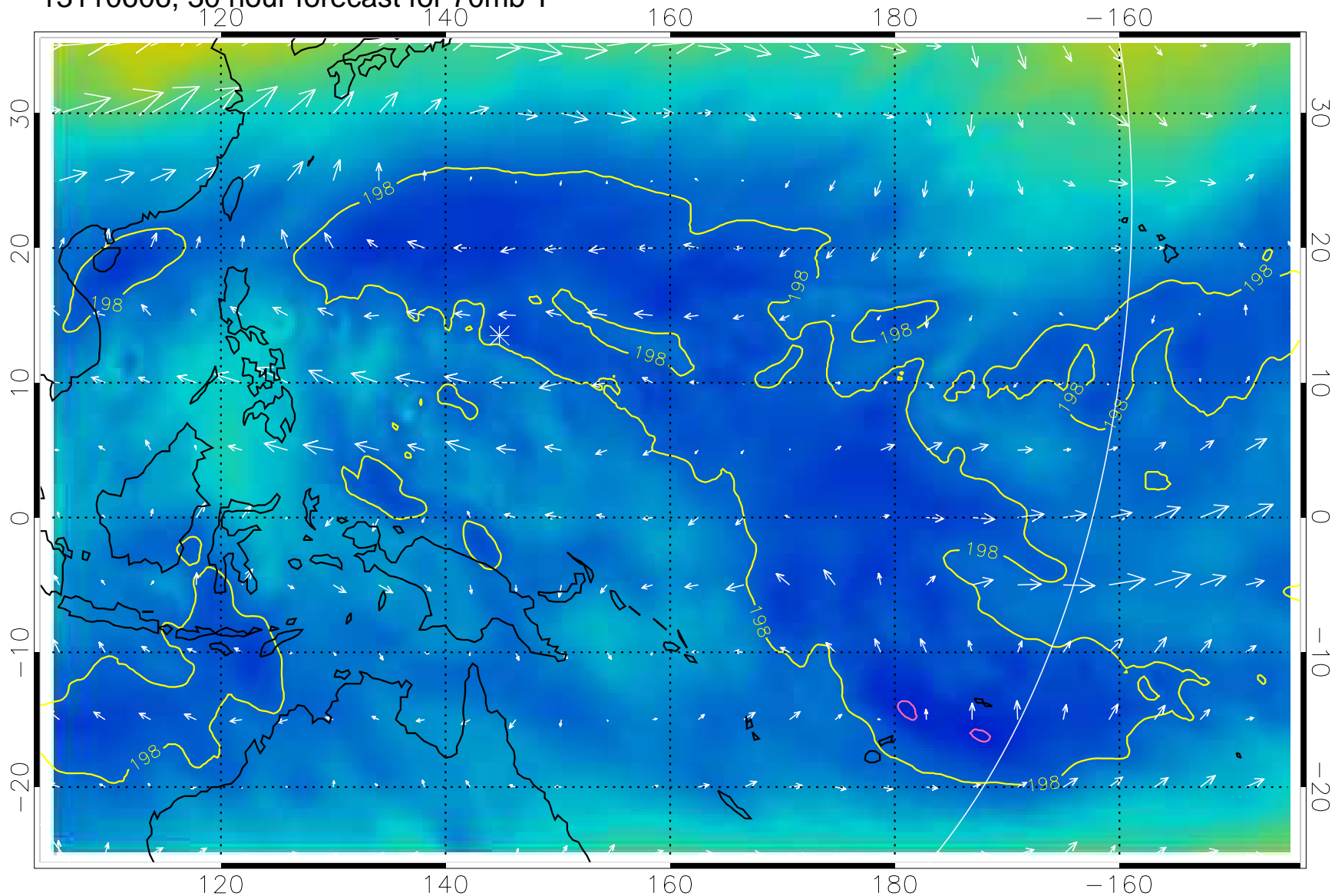
13110606, 30 hour forecast for 70mb T
