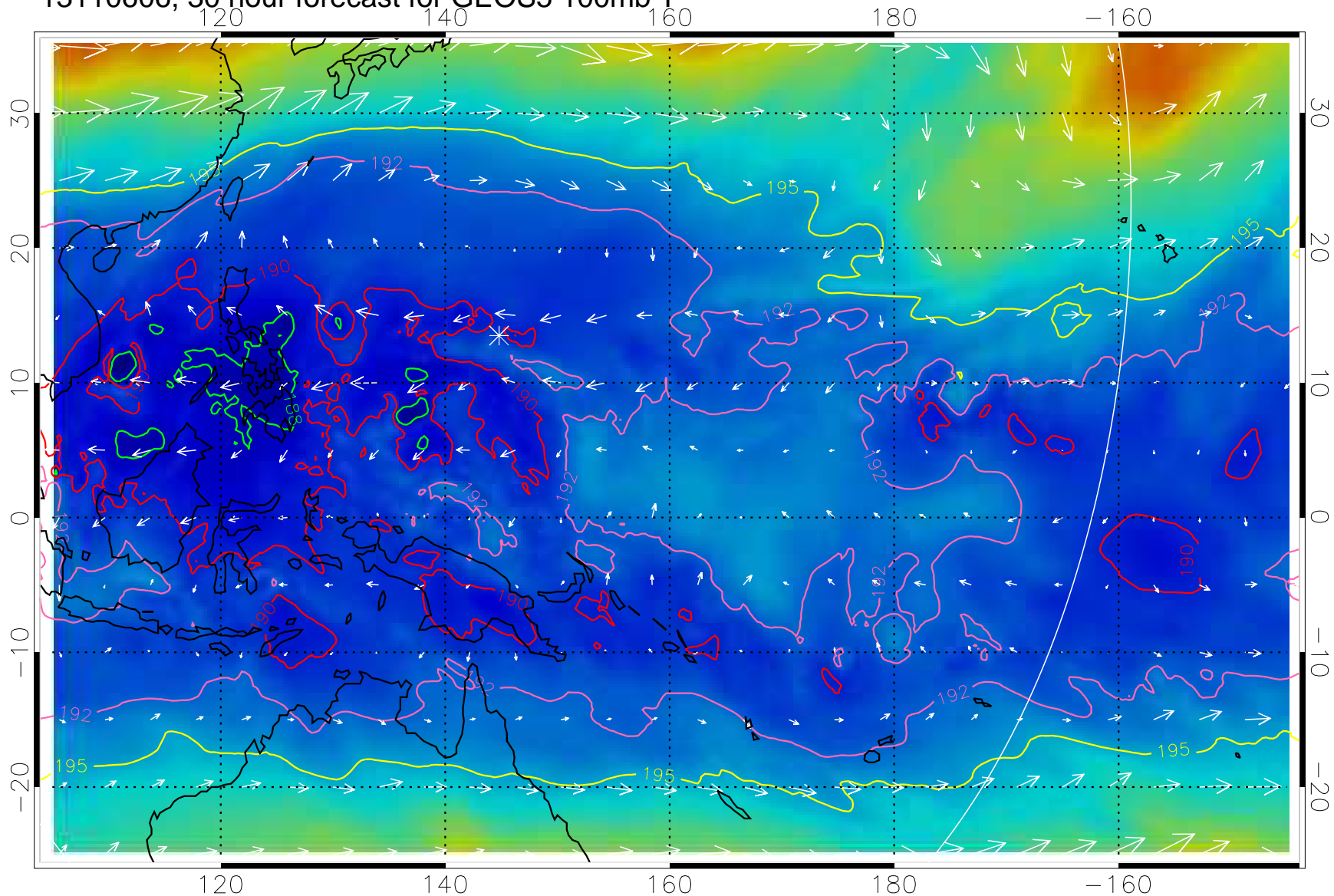
13110606, 30 hour forecast for GEOS5 100mb T
