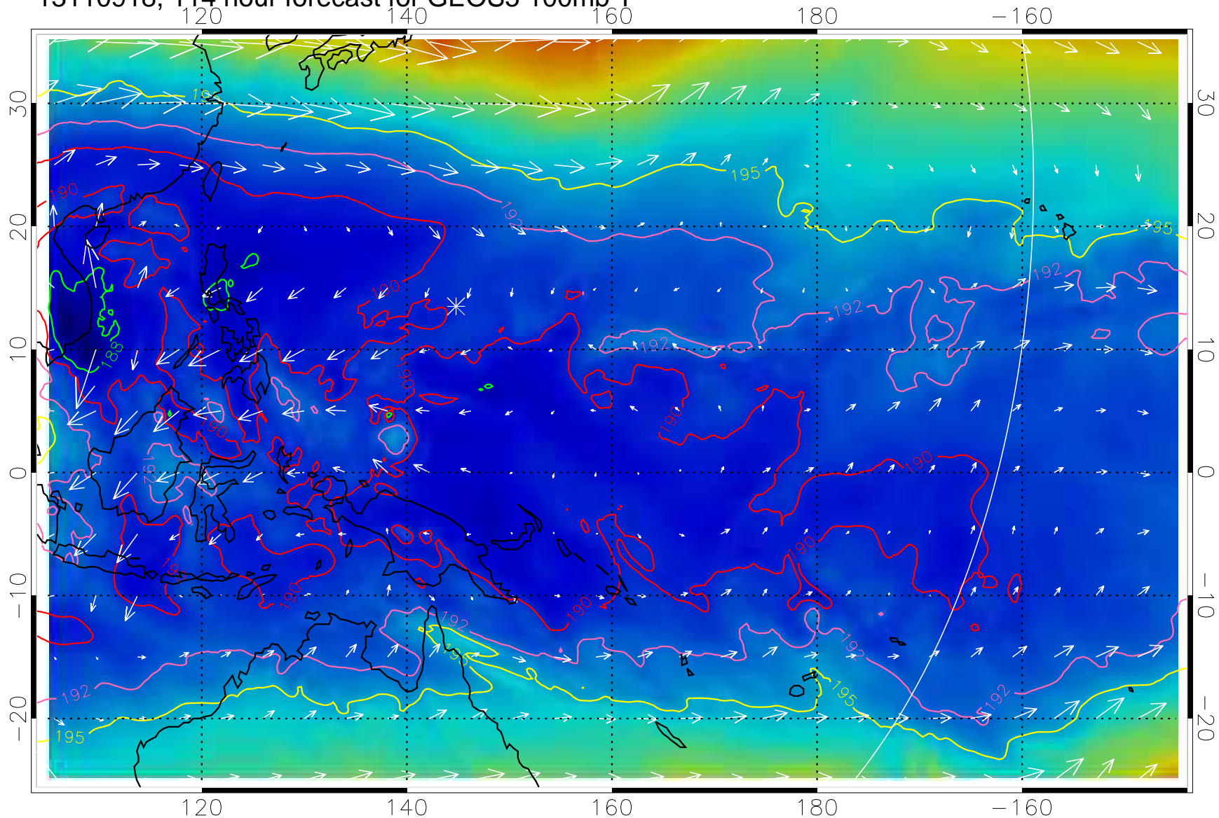
13110918, 114 hour forecast for GEOS5 100mb T
