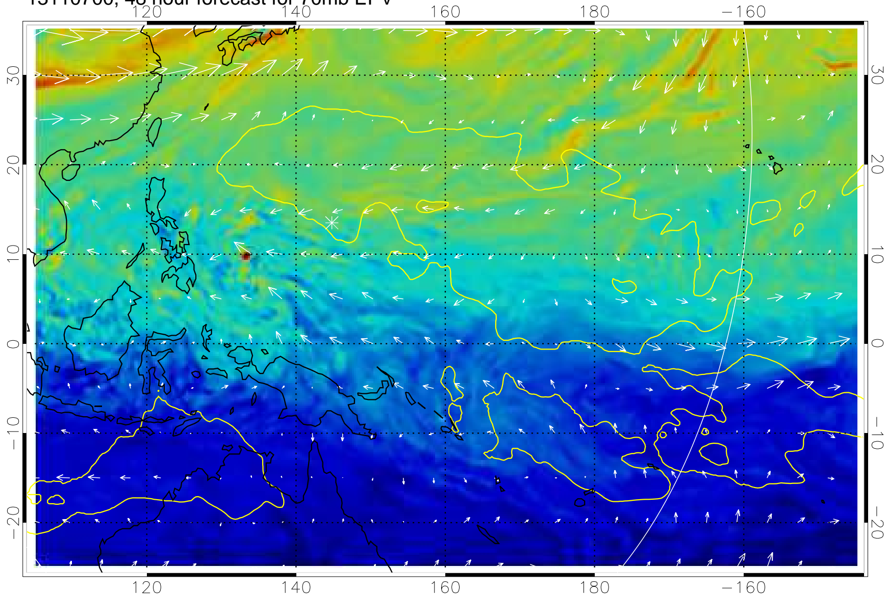
13110700, 48 hour forecast for 70mb EPV
