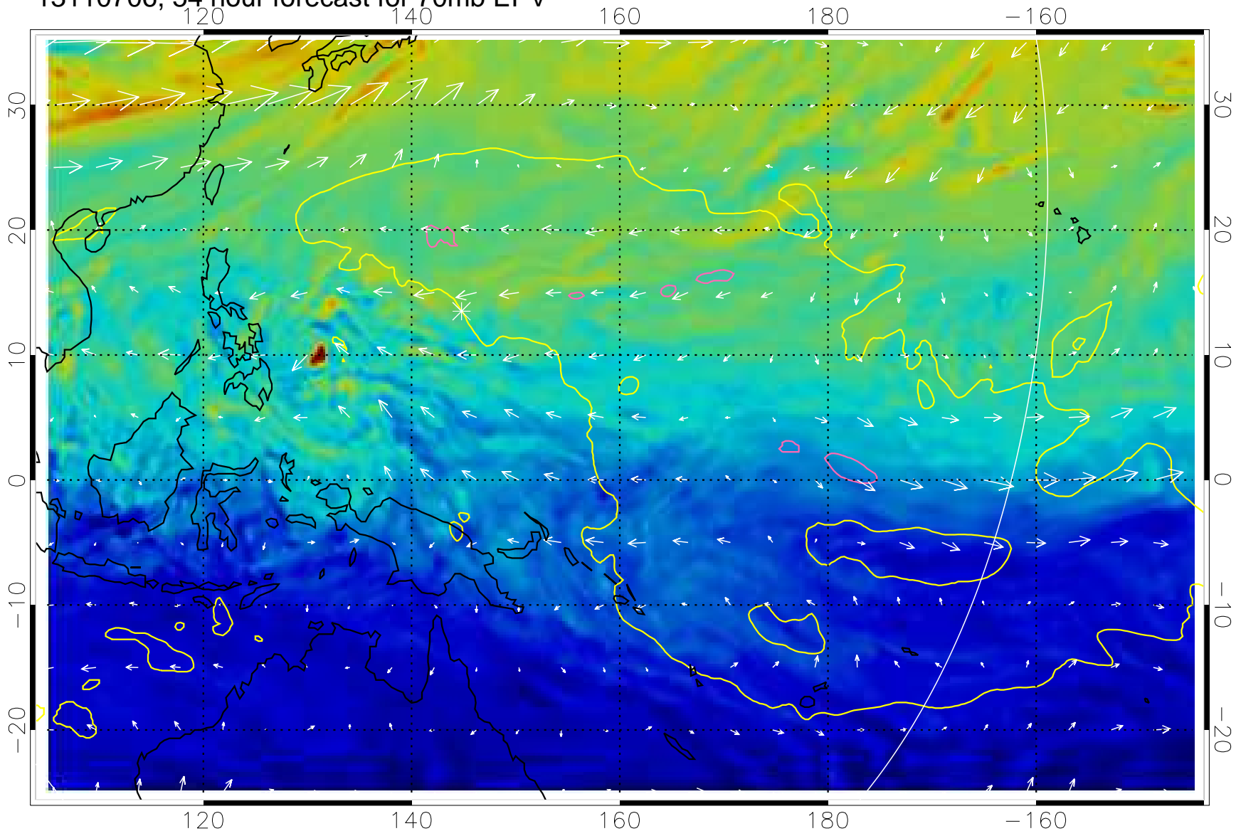
13110706, 54 hour forecast for 70mb EPV
