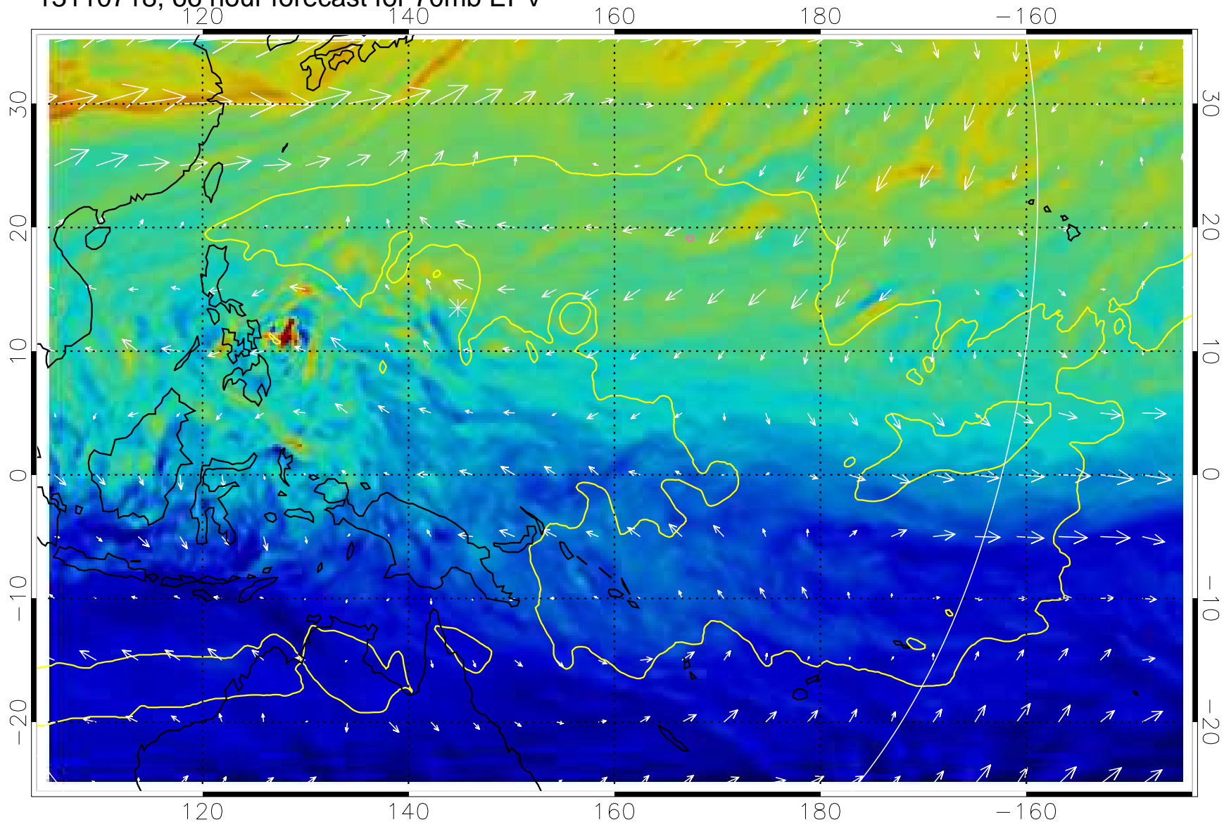
13110718, 66 hour forecast for 70mb EPV
