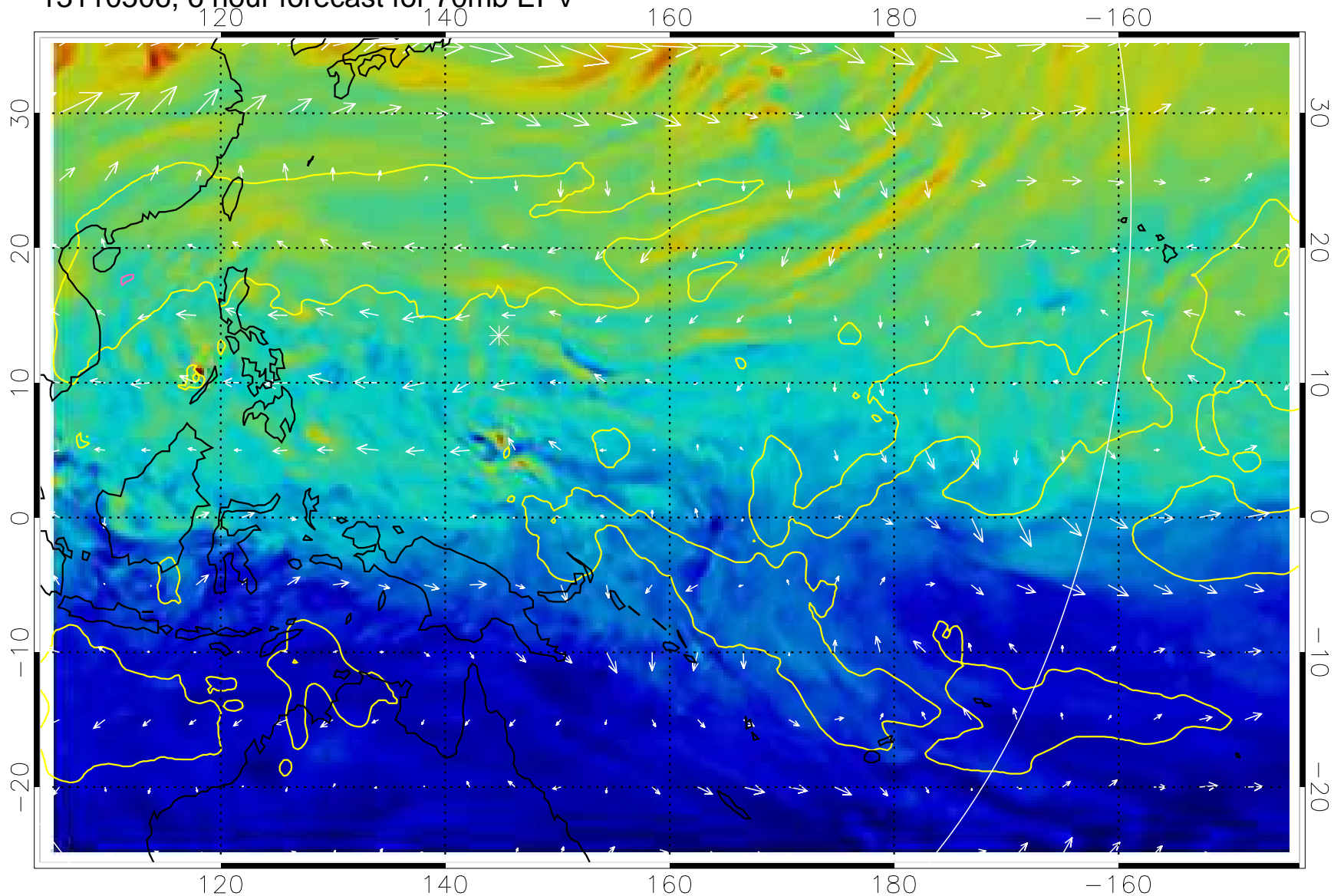
13110506, 6 hour forecast for 70mb EPV
