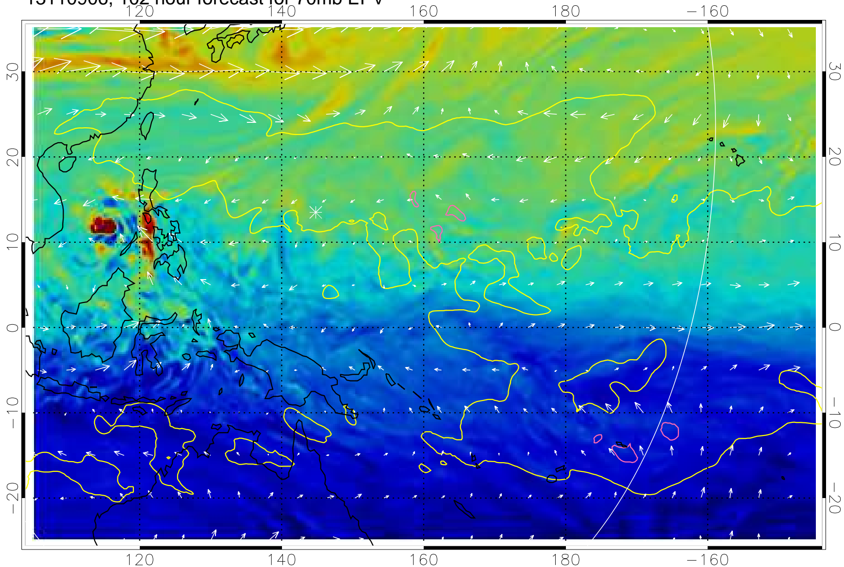
13110906, 102 hour forecast for 70mb EPV
