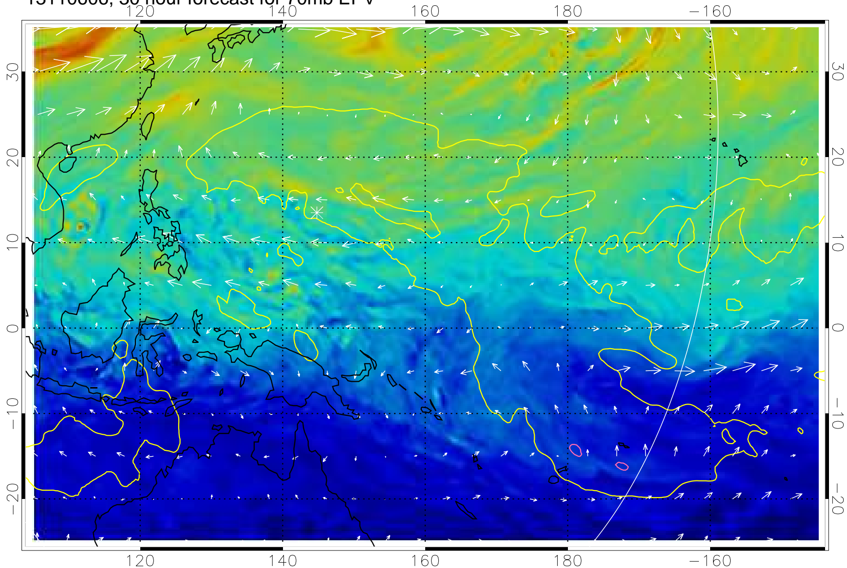
13110606, 30 hour forecast for 70mb EPV
