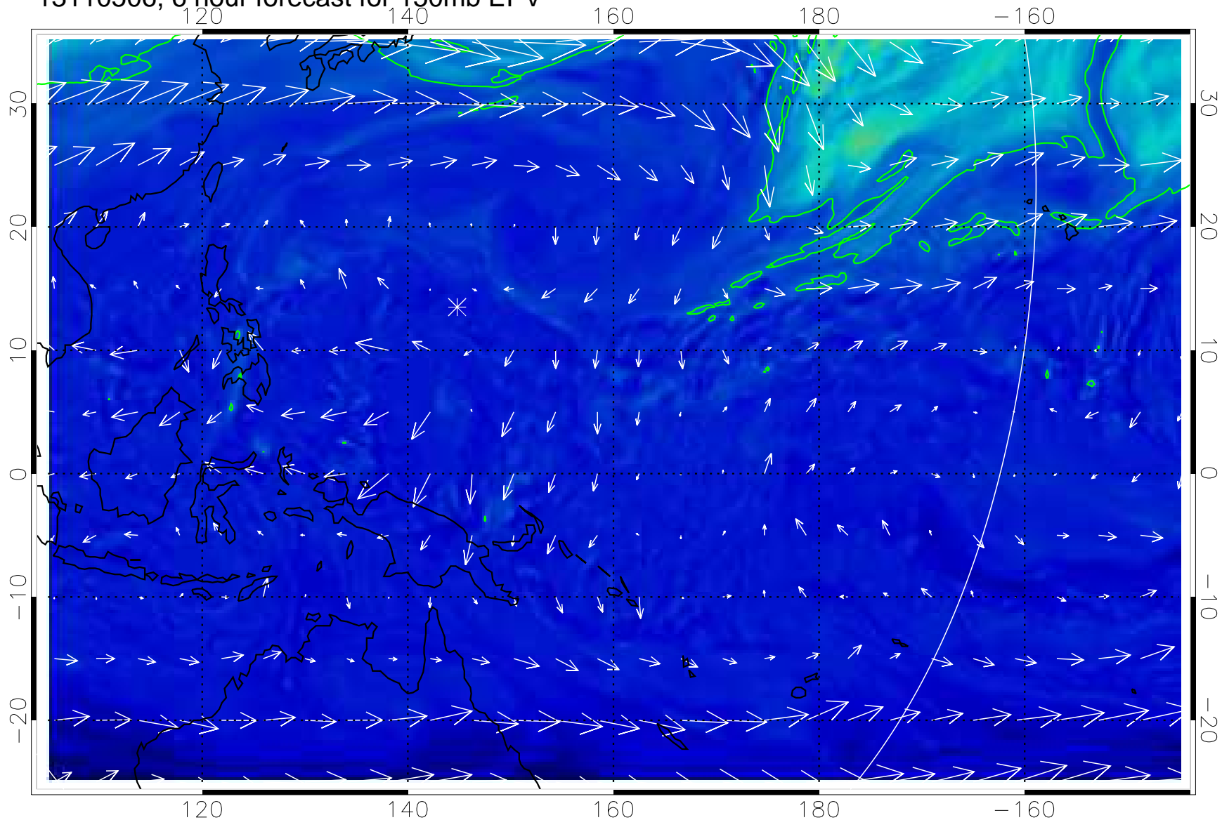
13110506, 6 hour forecast for 150mb EPV
