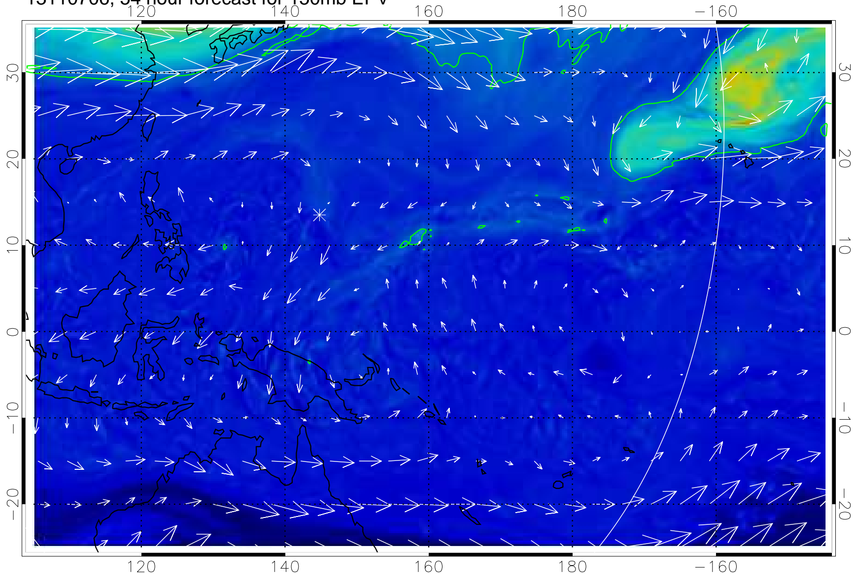
13110706, 54 hour forecast for 150mb EPV
