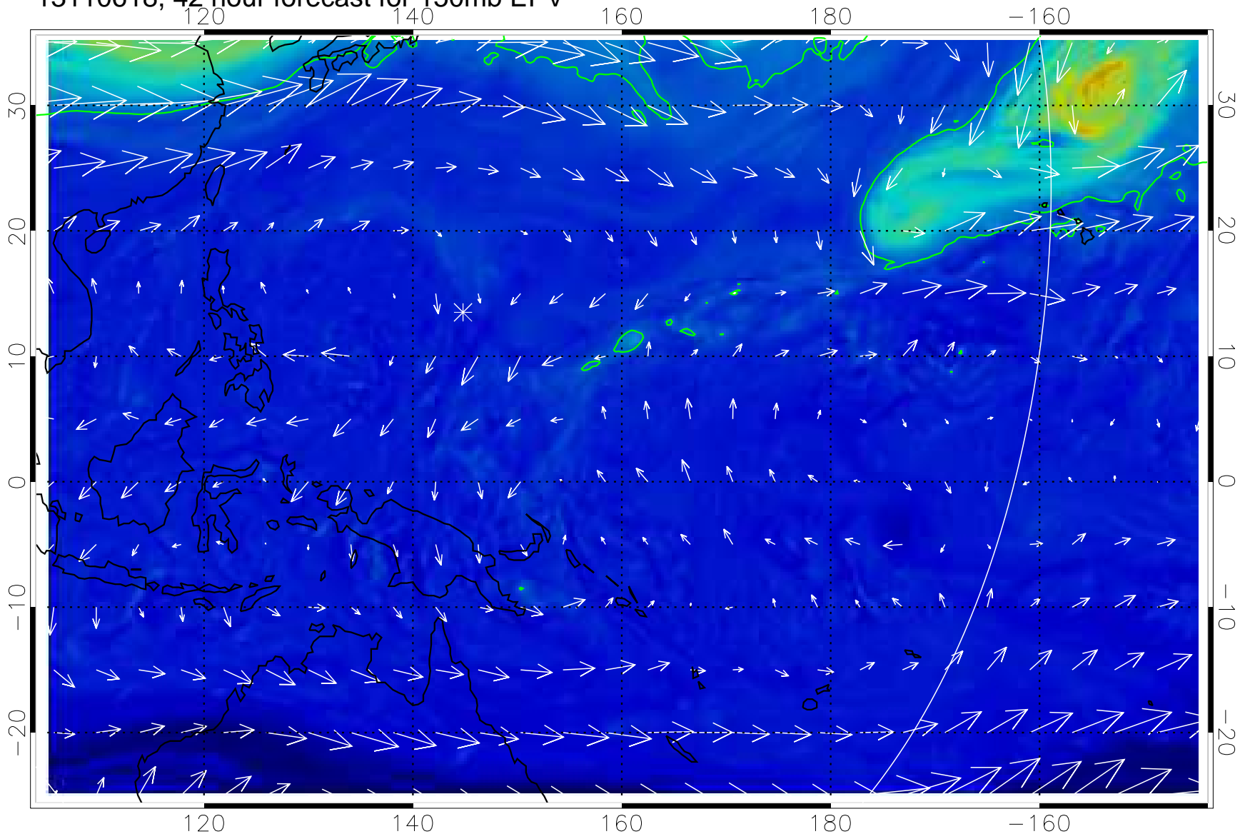
13110618, 42 hour forecast for 150mb EPV
