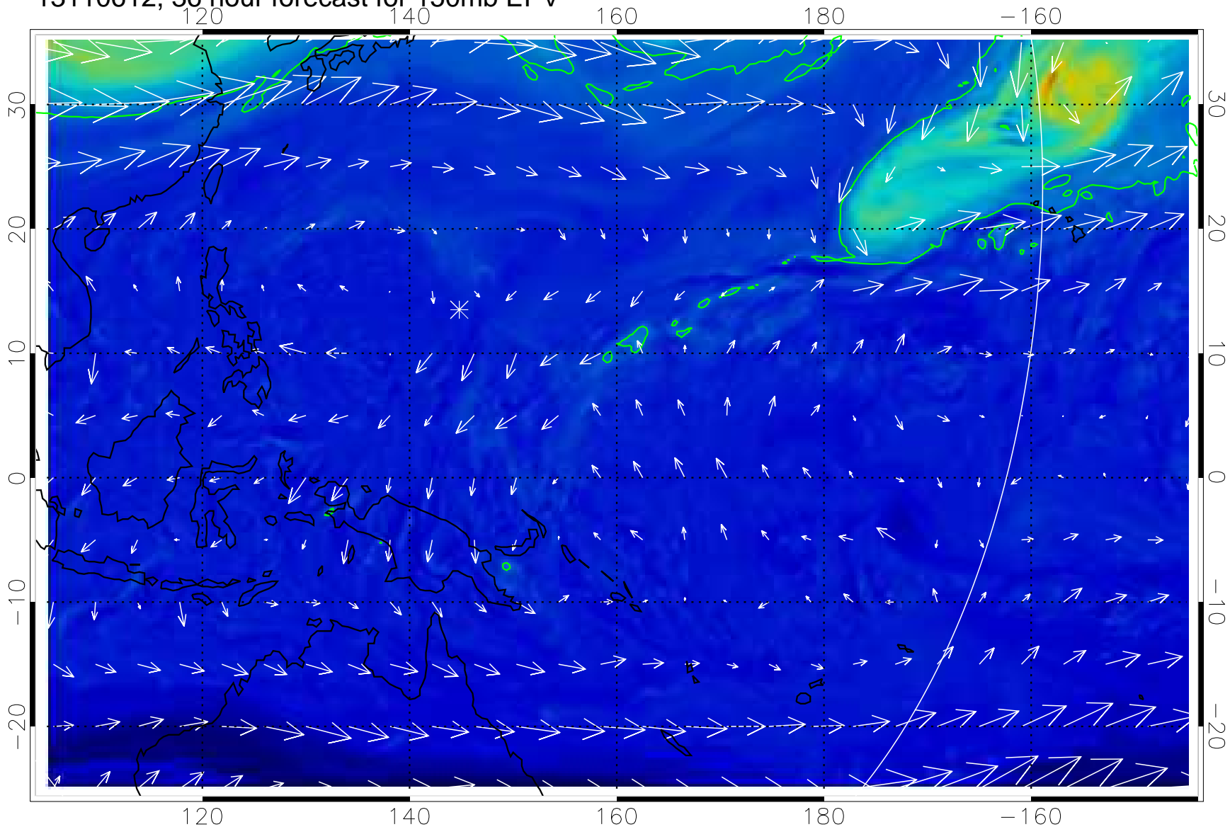
13110612, 36 hour forecast for 150mb EPV
