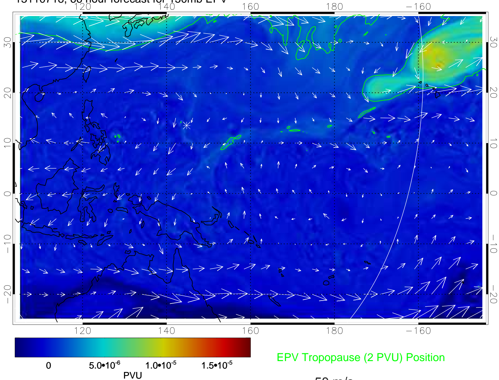
13110718, 66 hour forecast for 150mb EPV
