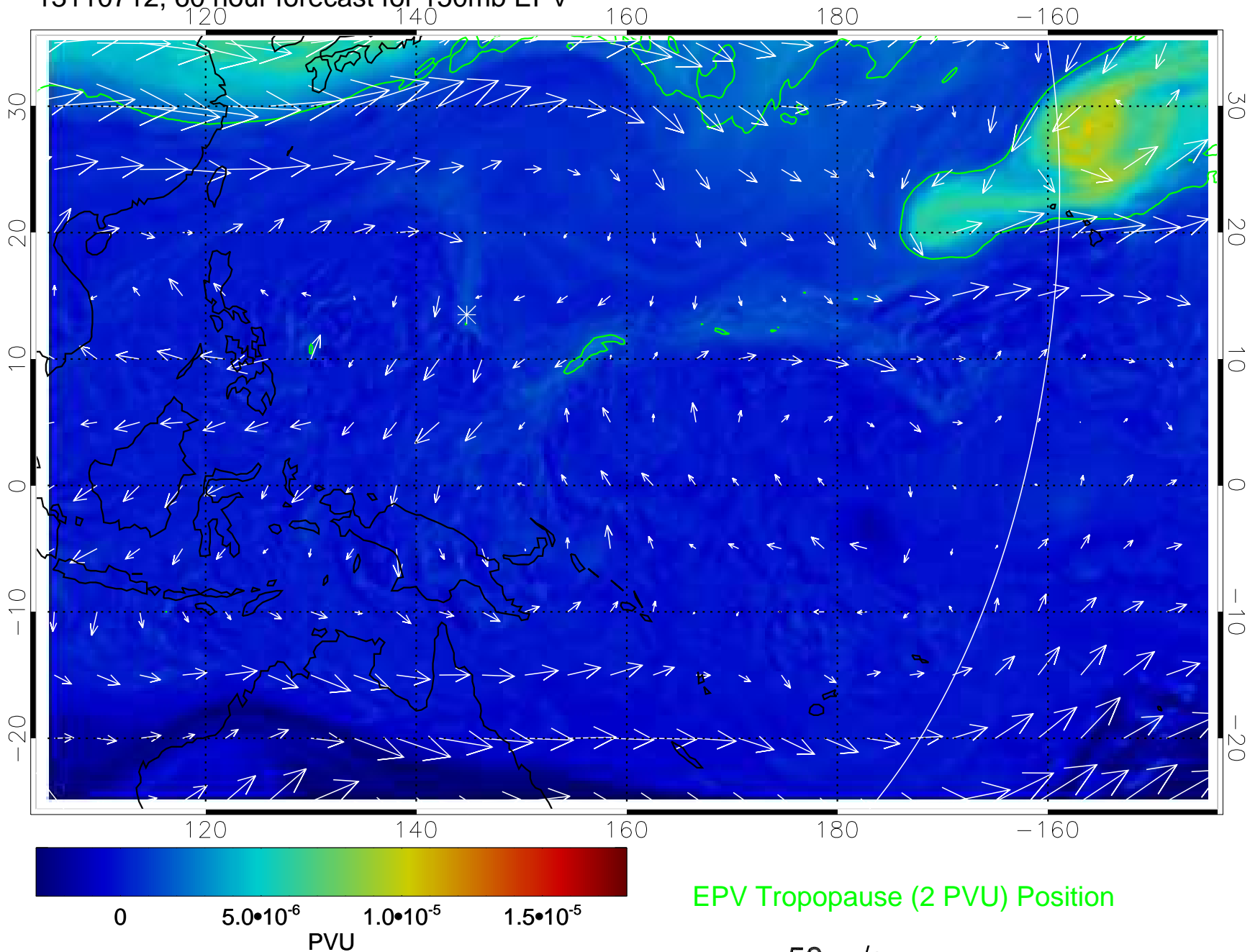
13110712, 60 hour forecast for 150mb EPV
