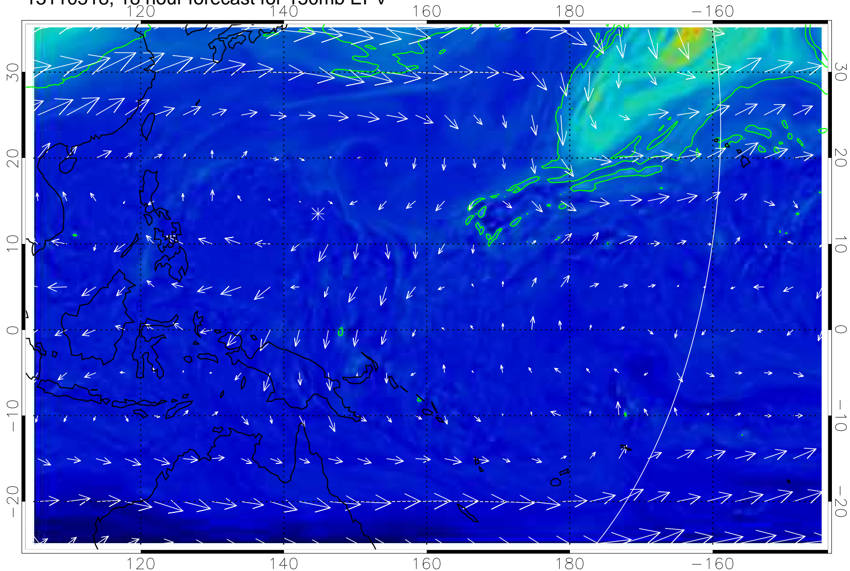
13110518, 18 hour forecast for 150mb EPV
