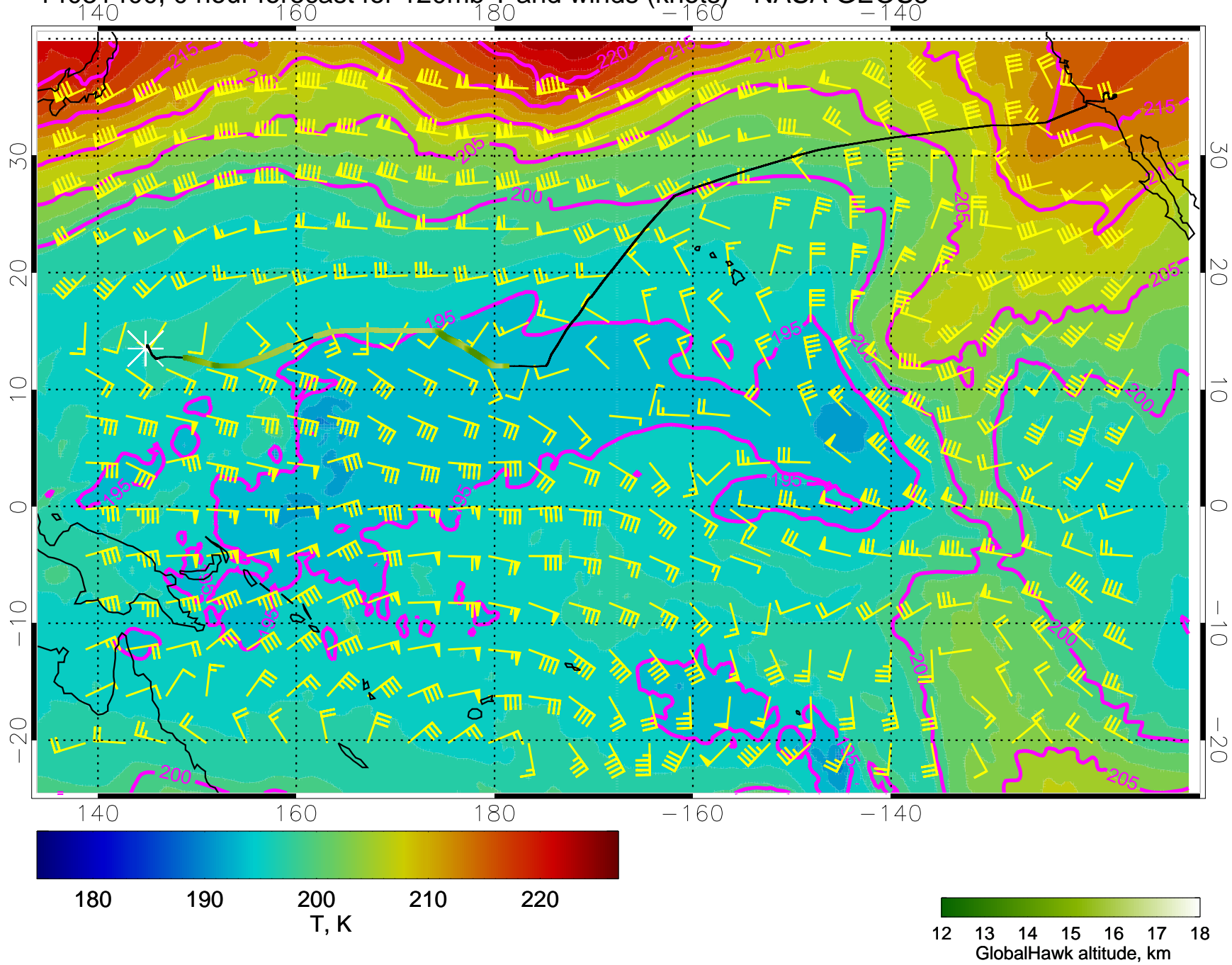
14031400, 0 hour forecast for 120mb T and winds (knots) - NASA GEOS5
