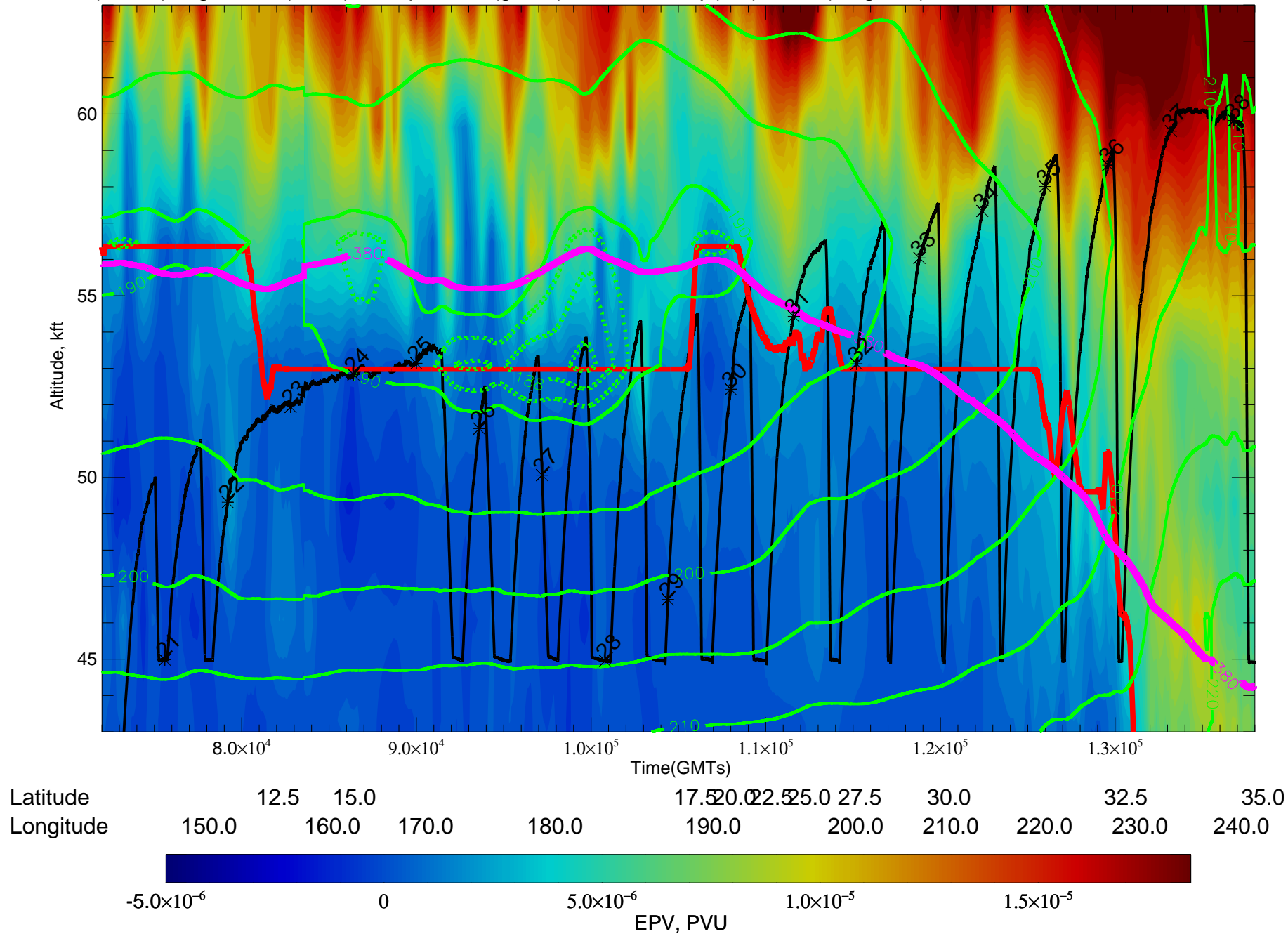
EPV(shade), flight track(black), Temperature(green), Thermal Trop(red), 380K(magenta) for 72000-138000 GMTs at 14031400
