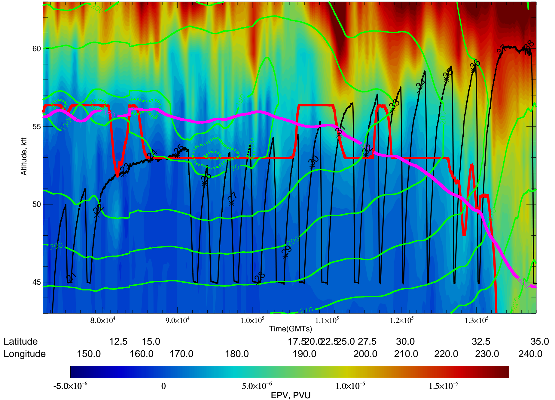
EPV(shade), flight track(black), Temperature(green), Thermal Trop(red), 380K(magenta) for 72000-138000 GMTs at 14031406
