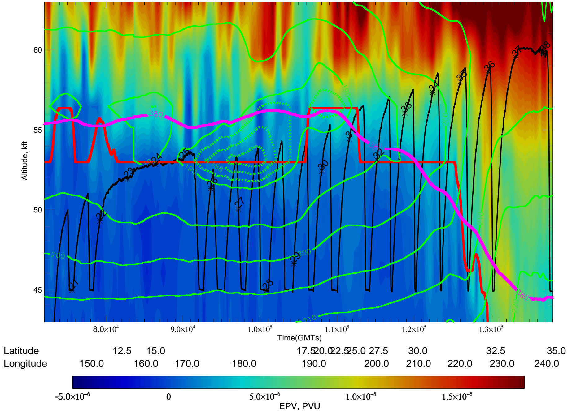
EPV(shade), flight track(black), Temperature(green), Thermal Trop(red), 380K(magenta) for 72000-138000 GMTs at 14031318
