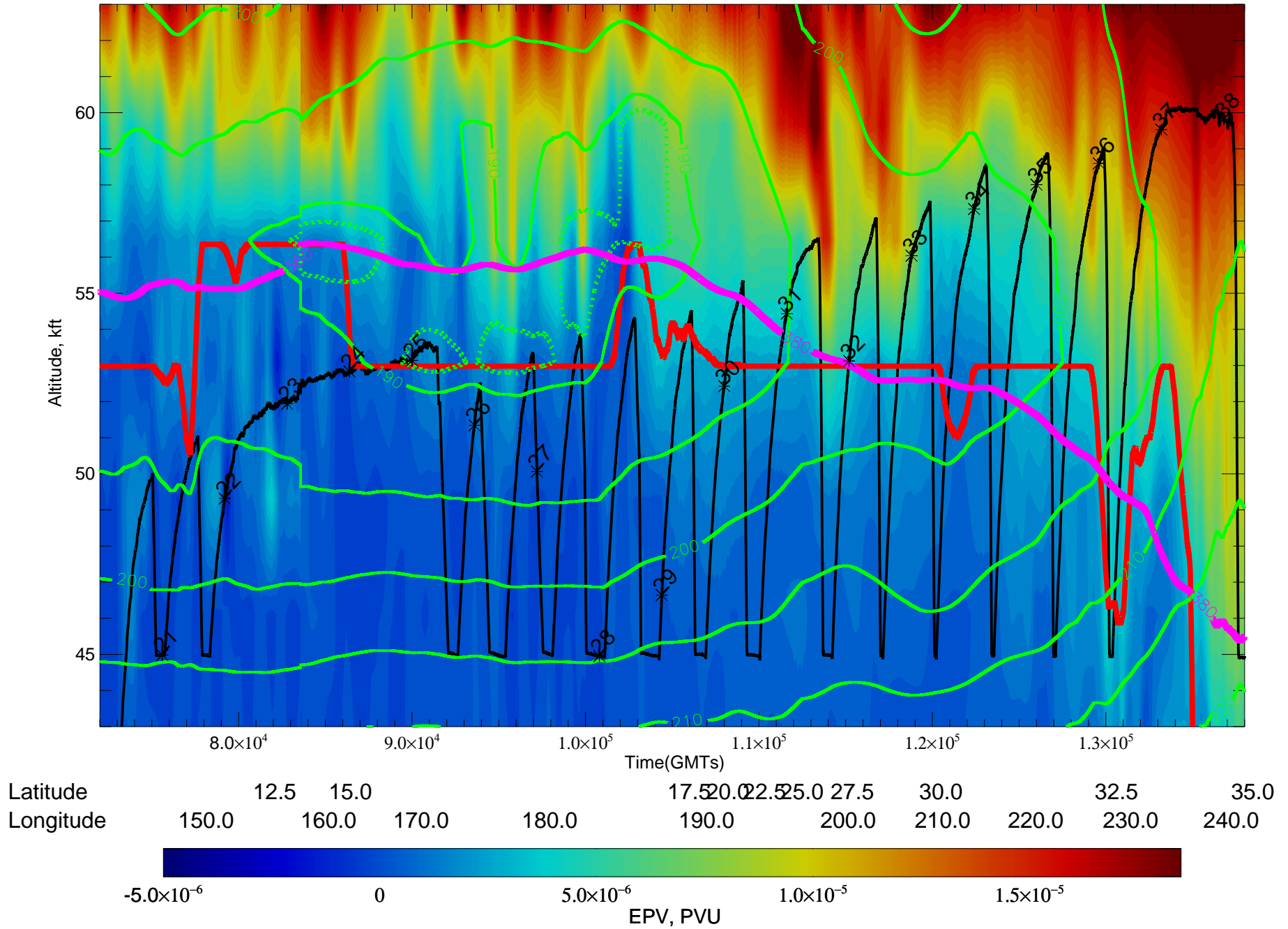
EPV(shade), flight track(black), Temperature(green), Thermal Trop(red), 380K(magenta) for 72000-138000 GMTs at 14031412
