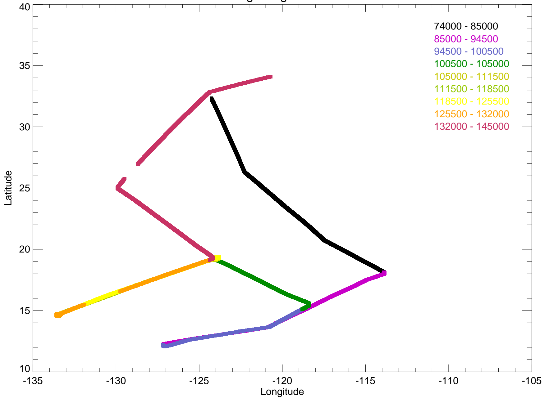
Color coded flight segments for 20111109
