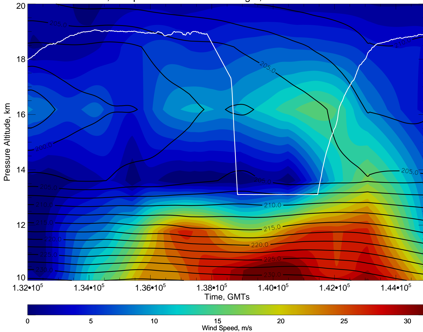
Wind, Temp X-sect for 20111109 flight, GMA anal at 11111018
