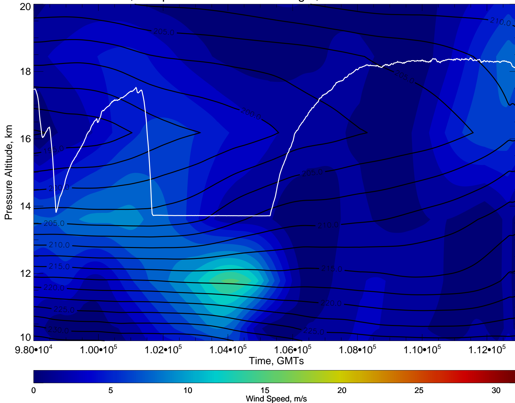
Wind, Temp X-sect for 20111105 flight, GMA anal at 11110606
