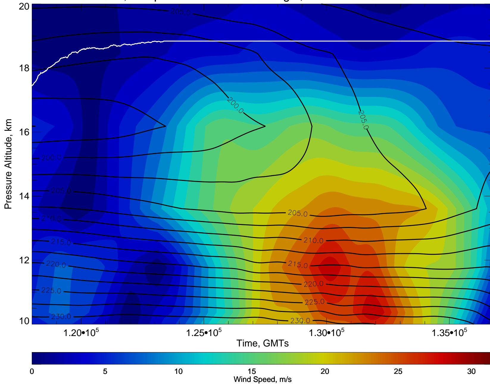
Wind, Temp X-sect for 20111028 flight, GMA anal at 11102912
