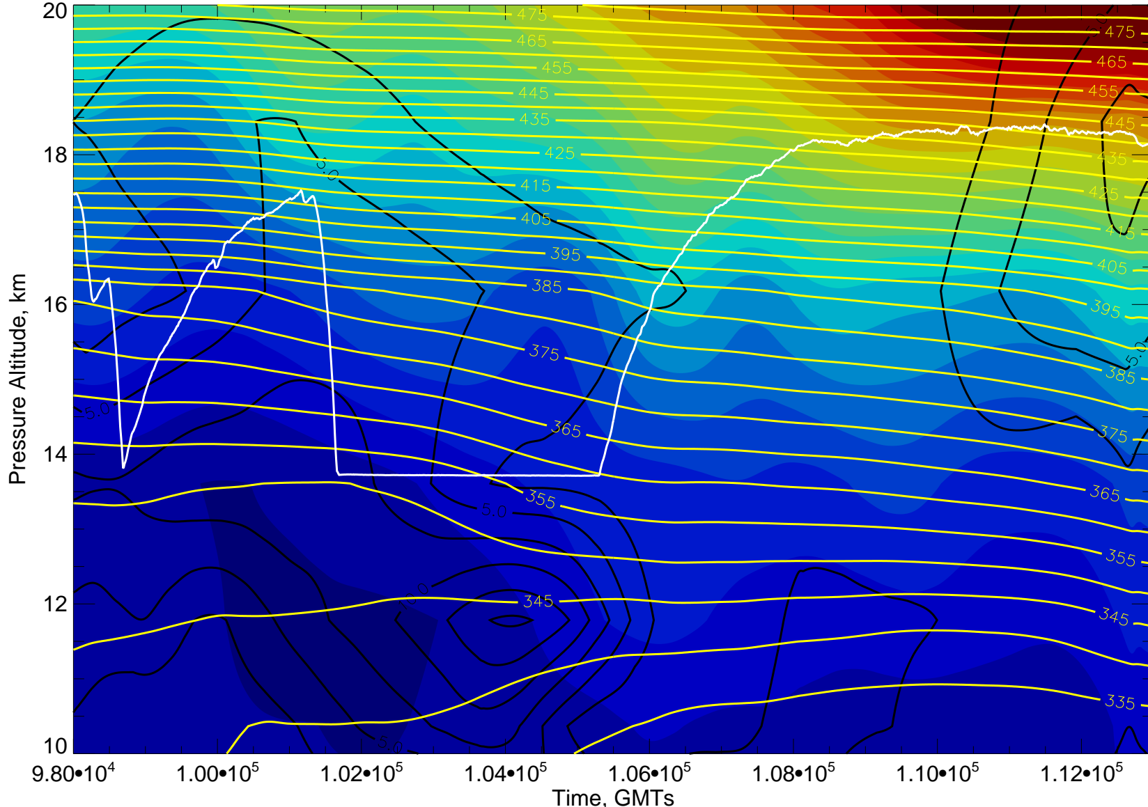
EPV, Wind, Theta, X-sect for 20111105 flight, GMA anal at 11110606
