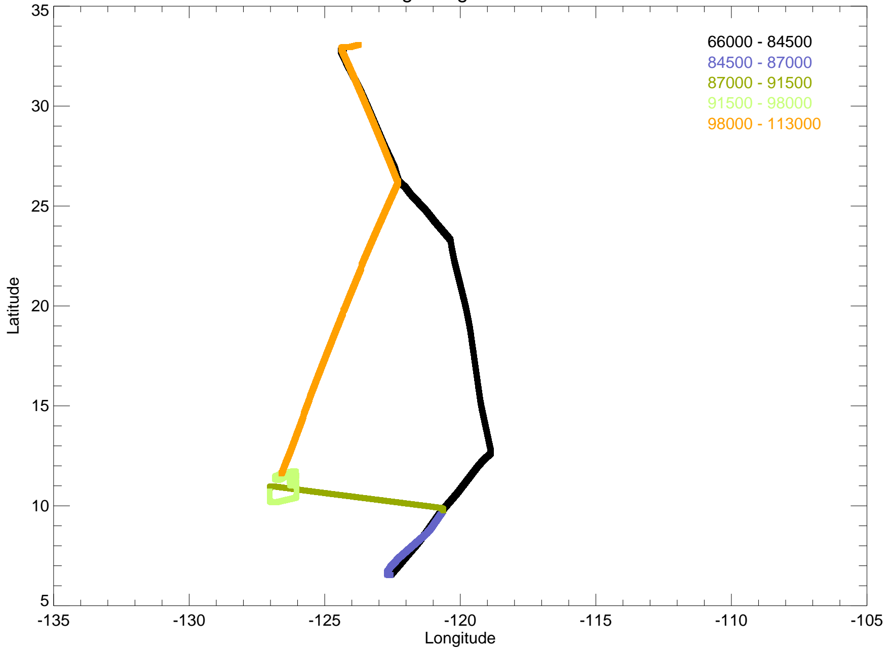
Color coded flight segments for 20111105
