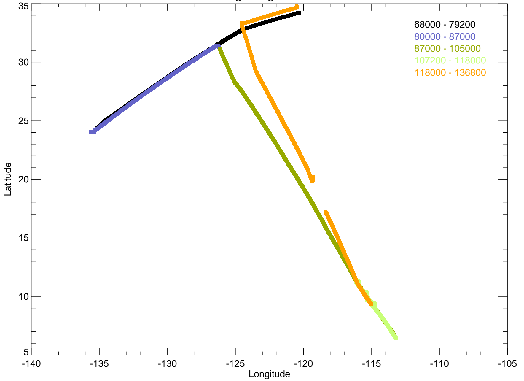
Color coded flight segments for 20111028
