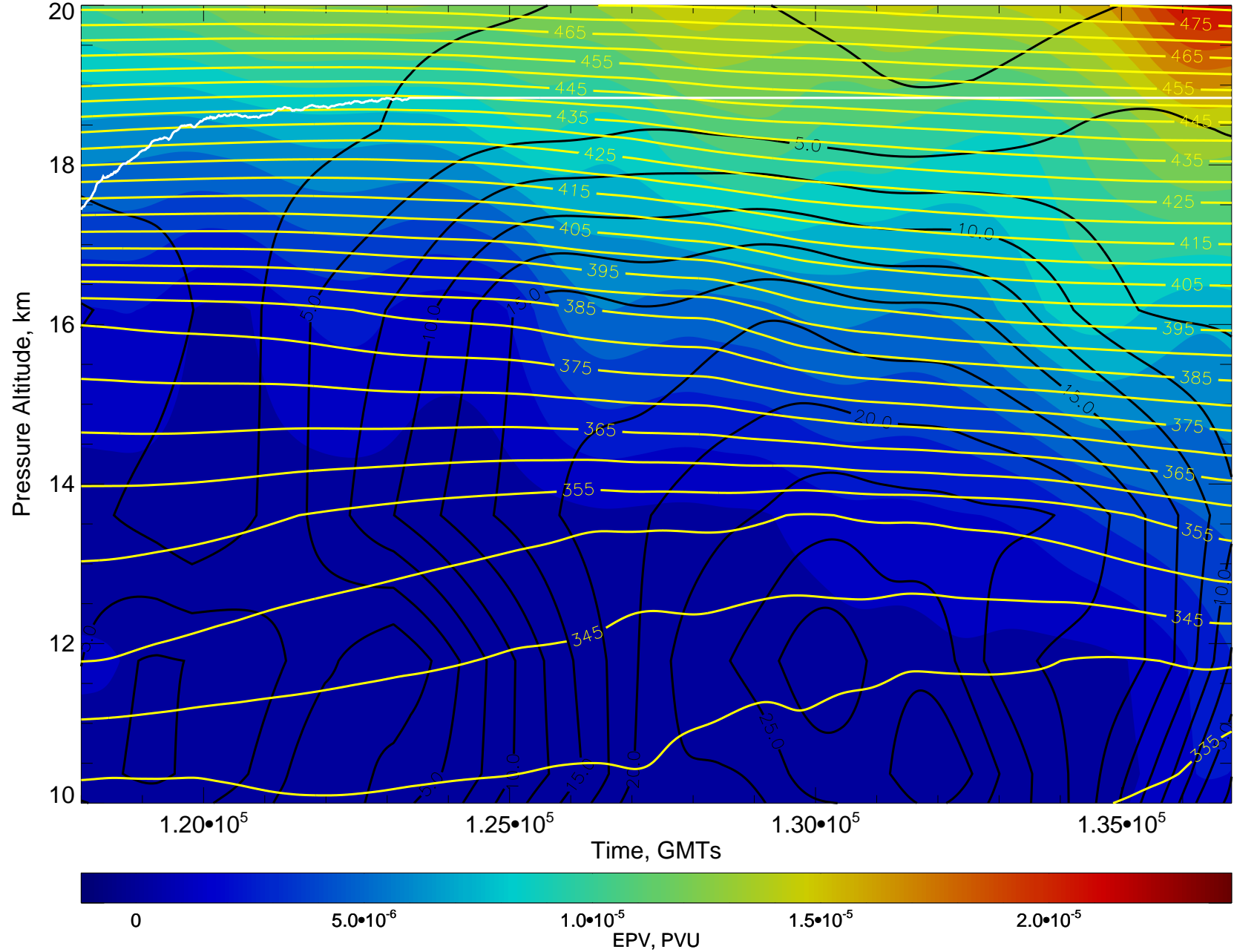
EPV, Wind, Theta, X-sect for 20111028 flight, GMA anal at 11102912
